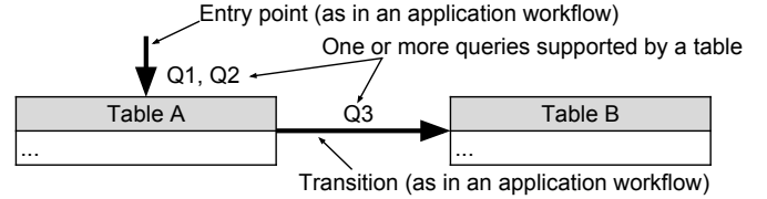
Fig. 6: The notation of Chebotko Diagrams.
