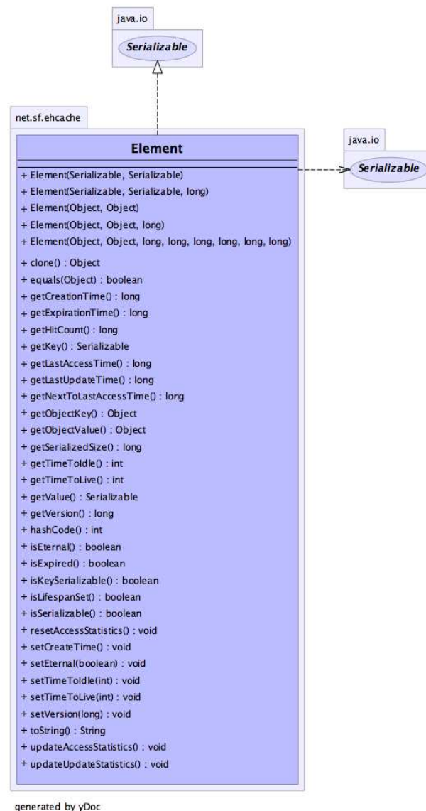
Element Class Diagram
