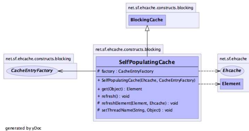
SelfPopulatingCache
