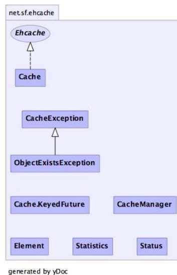
Top Level Package Diagram
