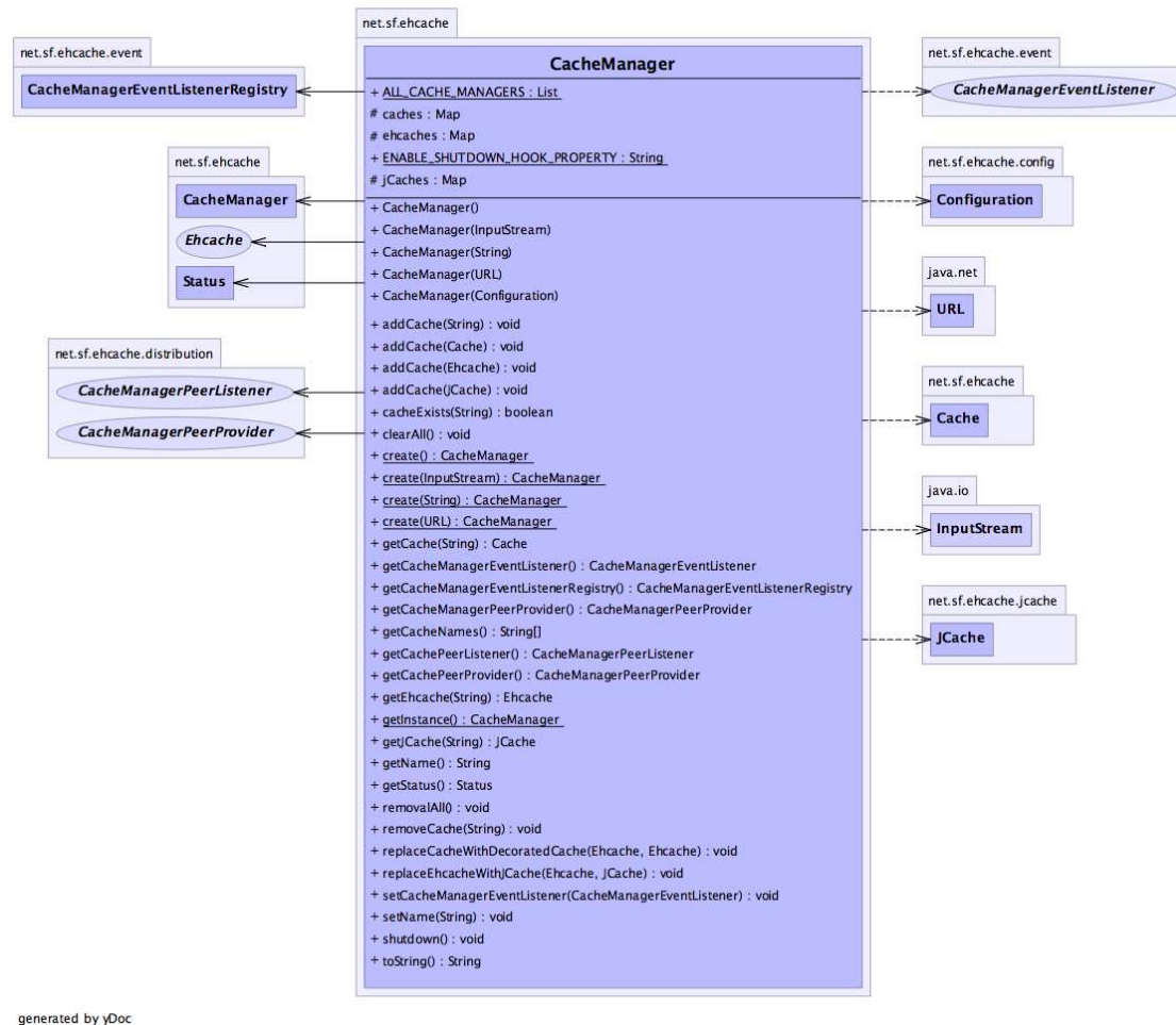
CacheManager Class Diagram
