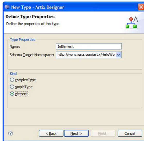
Figure 5: The Define Type Properties Panel
