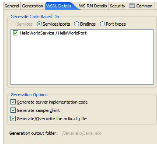
Figure 25: Artix Tools panel, WSDL Details tab
