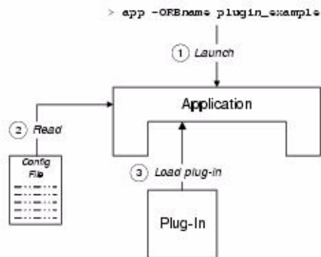
Figure 12: Loading a Plug-In
