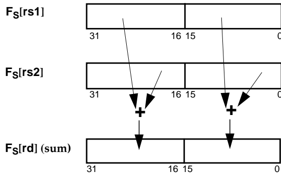
FIGURE 7-22 FPADD16S Operation
