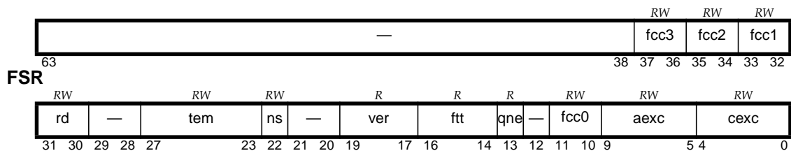
FIGURE 6-4 FSR Fields
