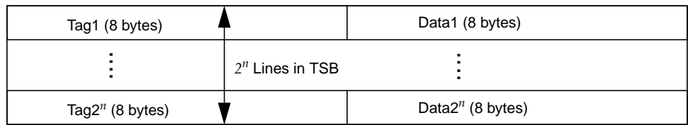
FIGURE 14-3 TSB Organization
