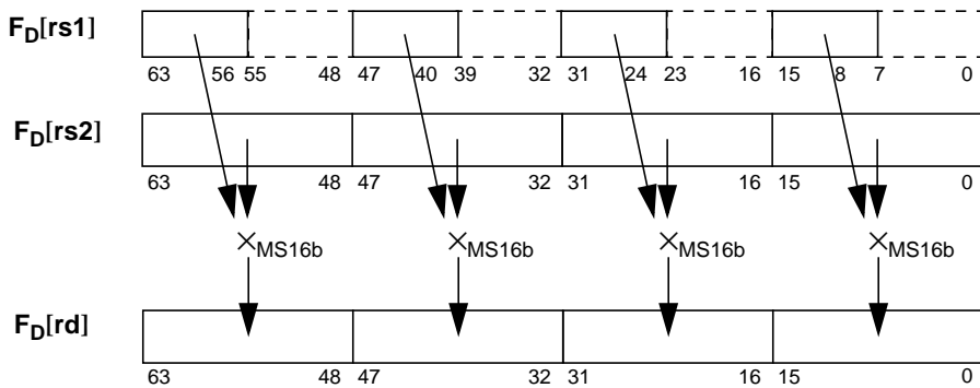
FIGURE 7-13 FMUL8SUx16 Operation
