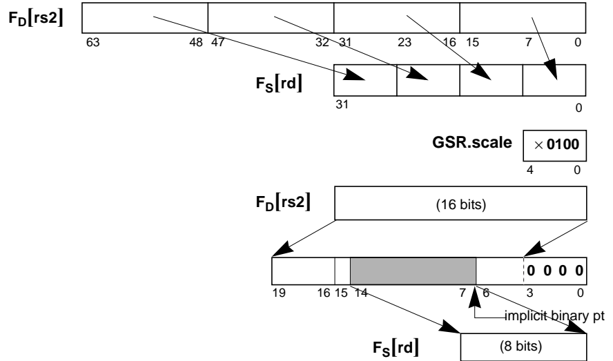
FIGURE 7-17 FPACK16 Operation
