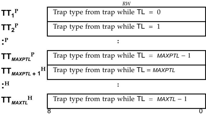
FIGURE 6-32 Trap Type Register Stack
