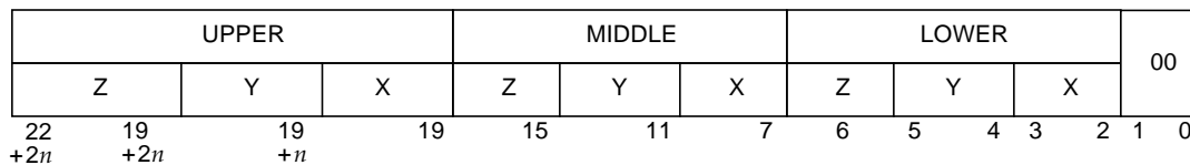
FIGURE 7-5 Three Dimensional Array Blocked-Address Format (ARRAY32)
