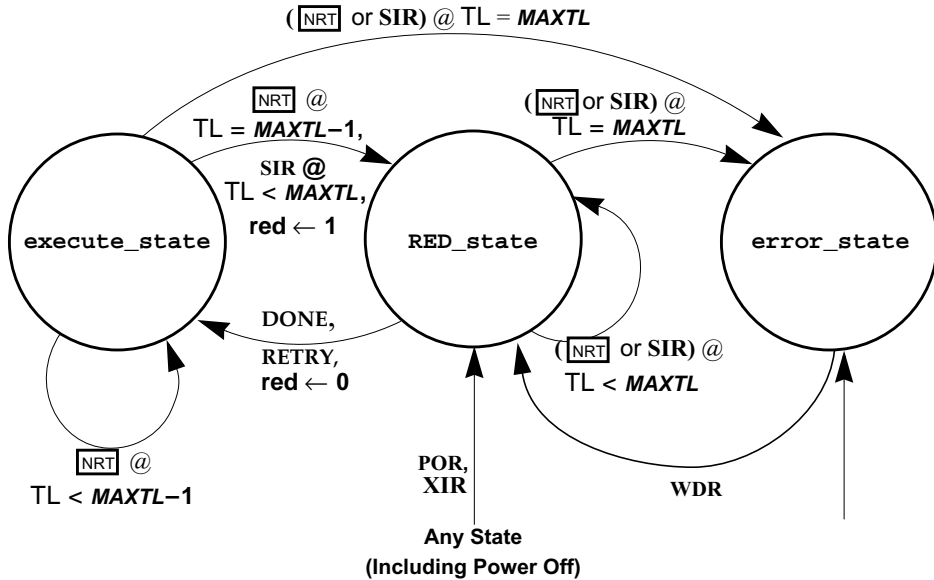
FIGURE 12-2 Virtual Processor State Diagram (“ NRT ” = “non-reset trap”)
