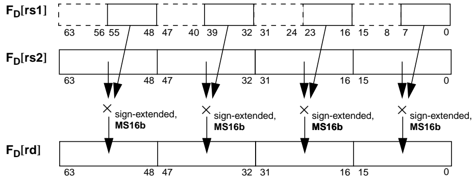
FIGURE 7-14 FMUL8ULx16 Operation
