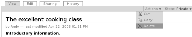
Figure 4.13: Actions menu
