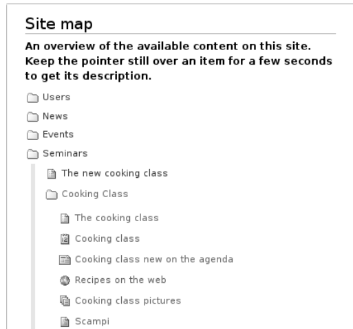
Figure 8.6: Site map
