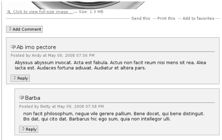
Figure 6.28: Commentary
