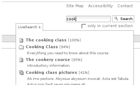
Figure 8.9: Live search
