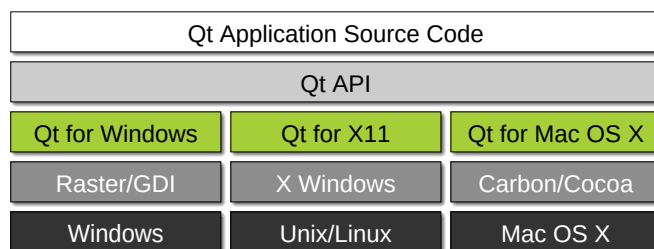
Figure 29: An overview of Qt's architecture on supported desktop platforms.
