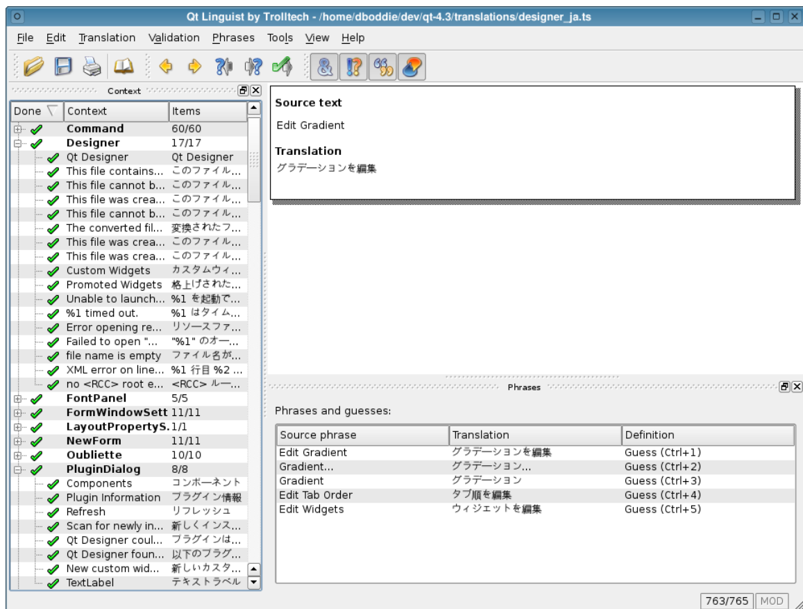
Figure 23: Working on a Japanese translation with Qt Linguist .
