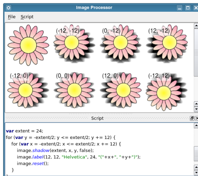
Figure 24: A simple image processing application using Qt Script.
