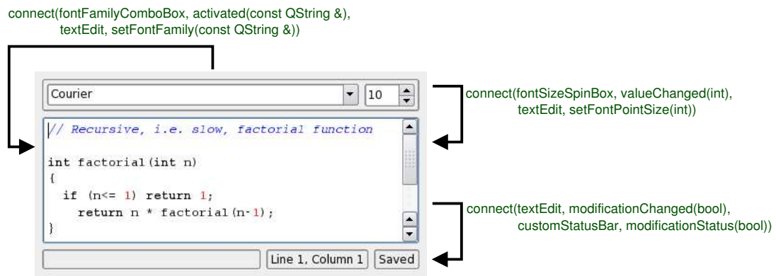
Figure 3: An example of signals and slots connections.
