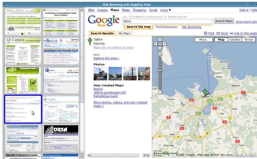
Figure 20: Qt widgets can be embedded into Web pages displayed with Qt's WebKit integration; Web Pages can be displayed as items in the Graphics View framework.
