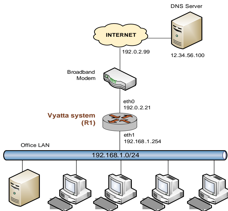
Figure 5-2 The Vyatta system configured as an Internet gateway
