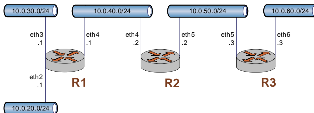
Figure 1-1 RIP configuration reference diagram
