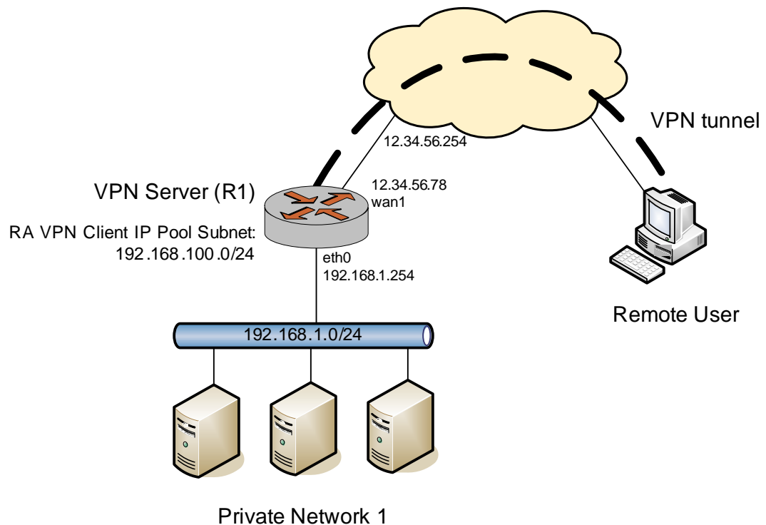
Figure 4-8 Remote Access VPN Example
