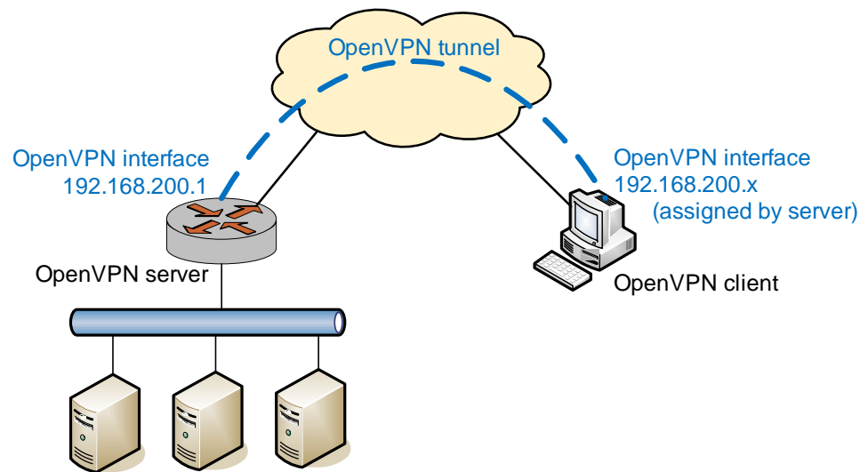
Figure 5-2 Remote access operation
