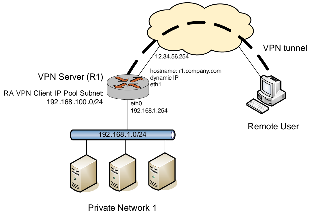
Figure 4-9 Remote Access VPN Example with a Dynamic IP Address
