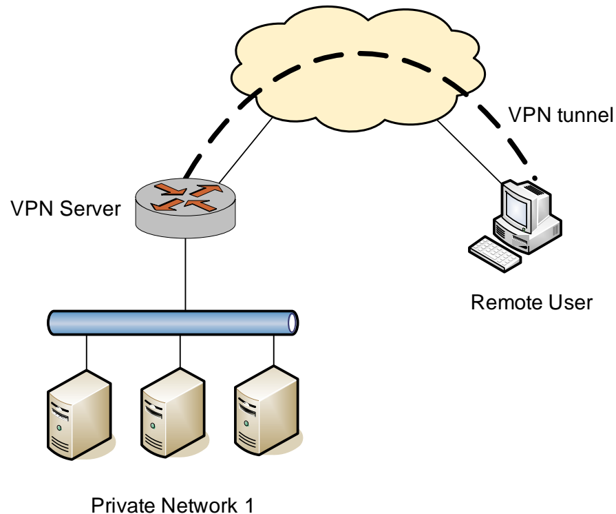
Figure 4-2 Remote Access VPN
