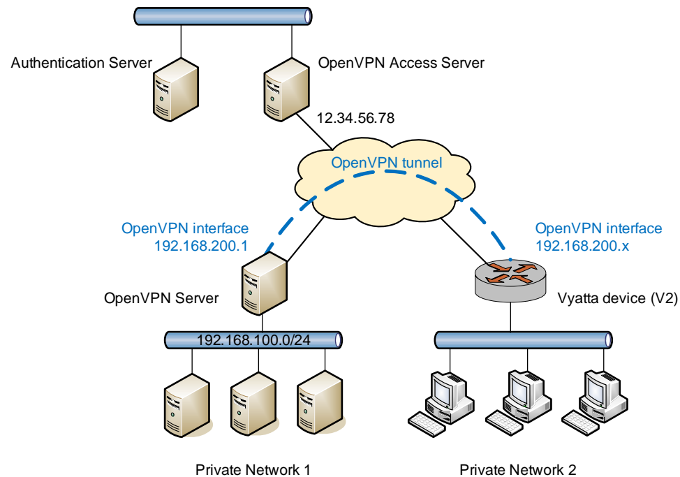
Figure 5-6 Using an OpenVPN Access Server to establish an OpenVPN tunnel
