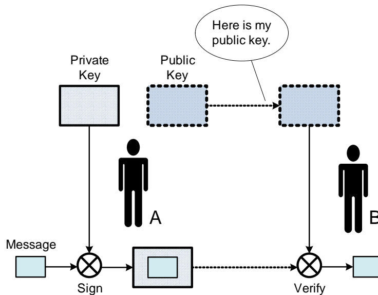
Figure 4-5 Digital signature
