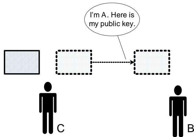
Figure 4-6 Malicious attacker
