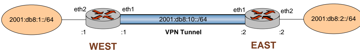
Figure 2-8 Basic site-to-site IPsec VPN connection over IPv6
