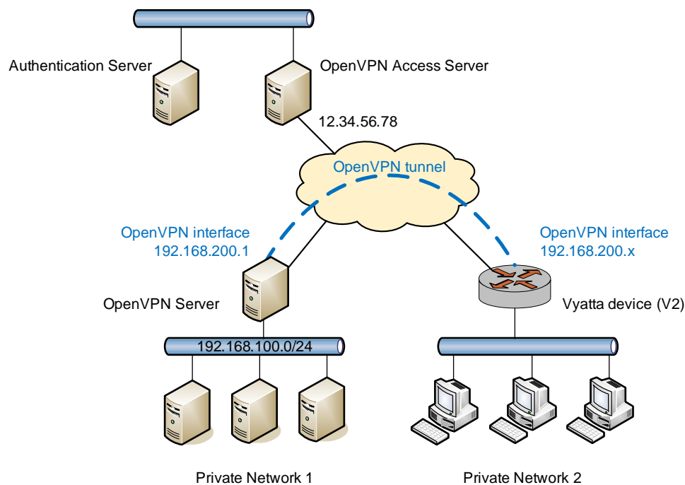
Figure 5-3 Client-side access to an OpenVPN Access Server
