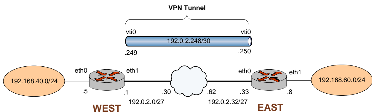
Figure 2-7 IPsec VPN connection with virtual tunnel interfaces
