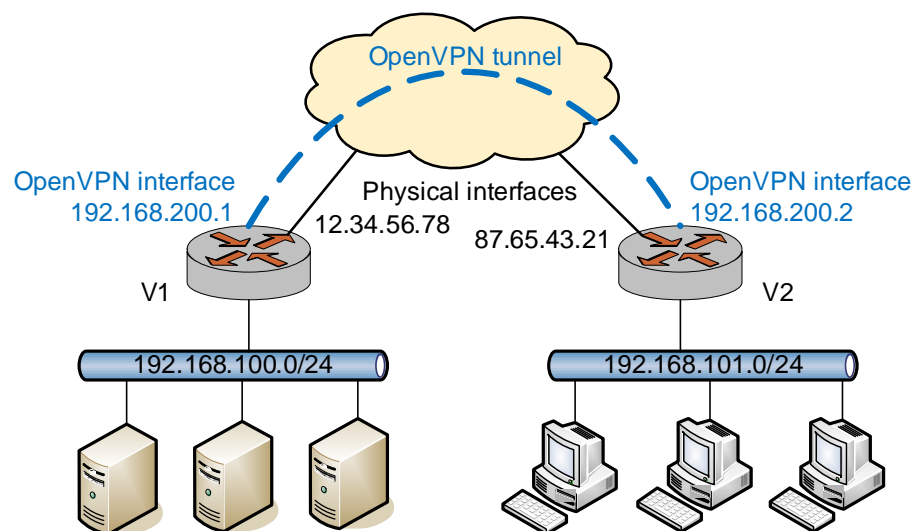
Figure 5-4 Site-to-site VPN with pre-shared secret
