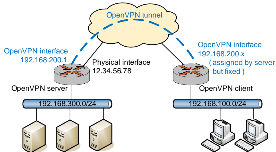
Figure 5-7 Client-server mode
