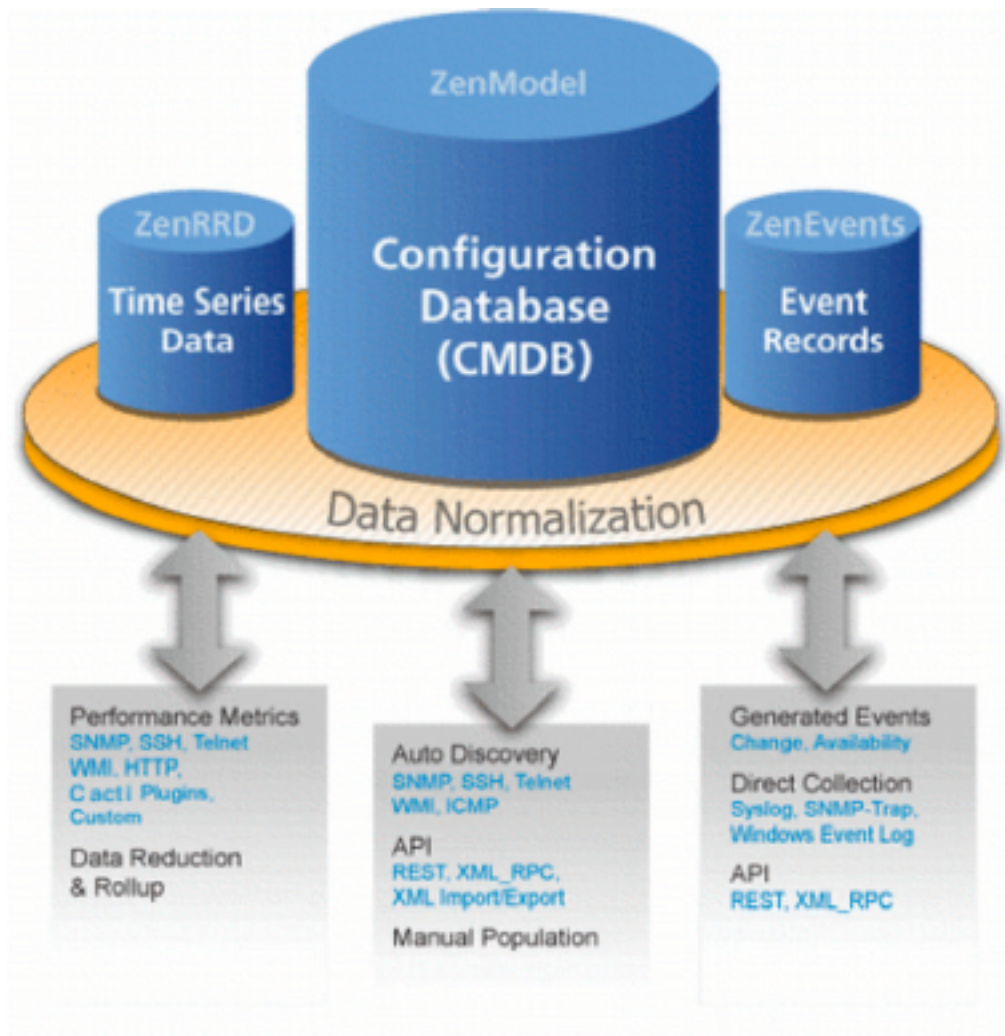
Figure 4.1. Datastores Overview
