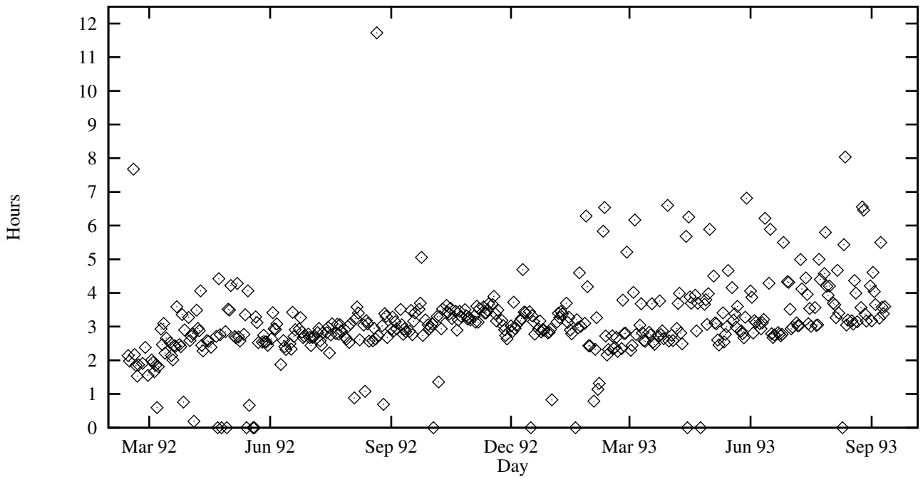
Figure 5: Nightly Amanda run times at CS.UMD.EDU
