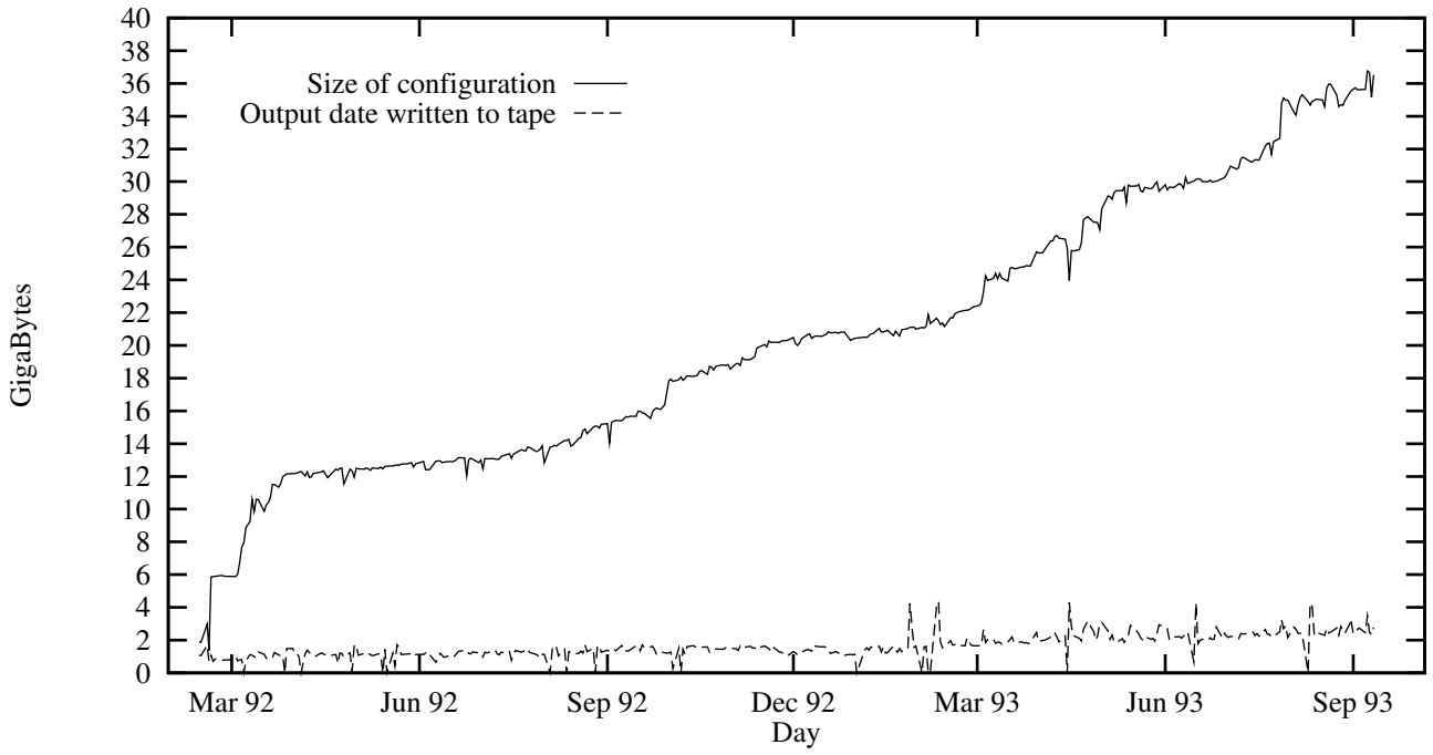
Figure 4: Nightly Amanda Backup Size at CS.UMD.EDU
