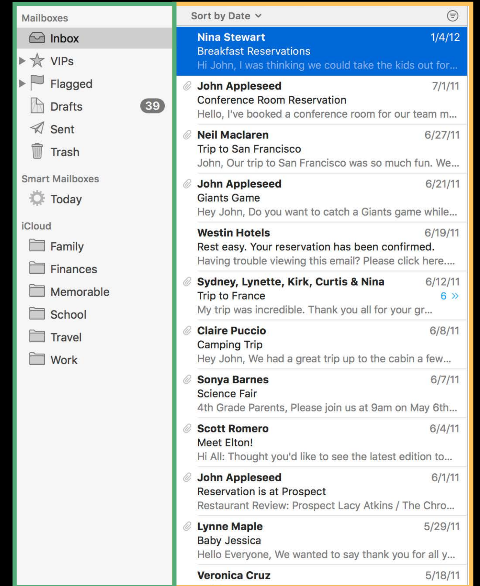
NSOutlineView
