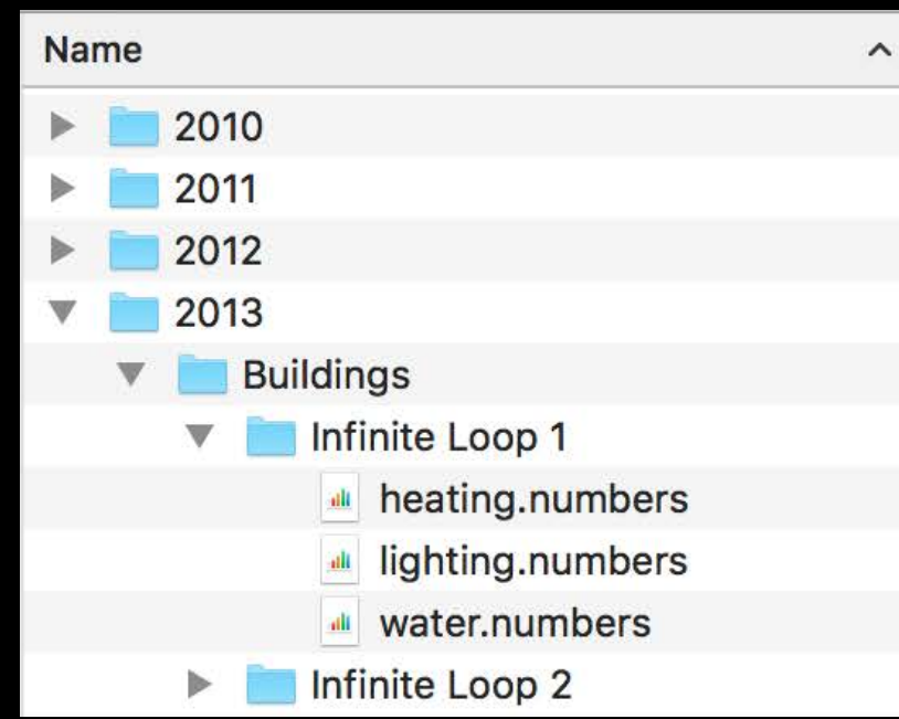
NSOutlineView
