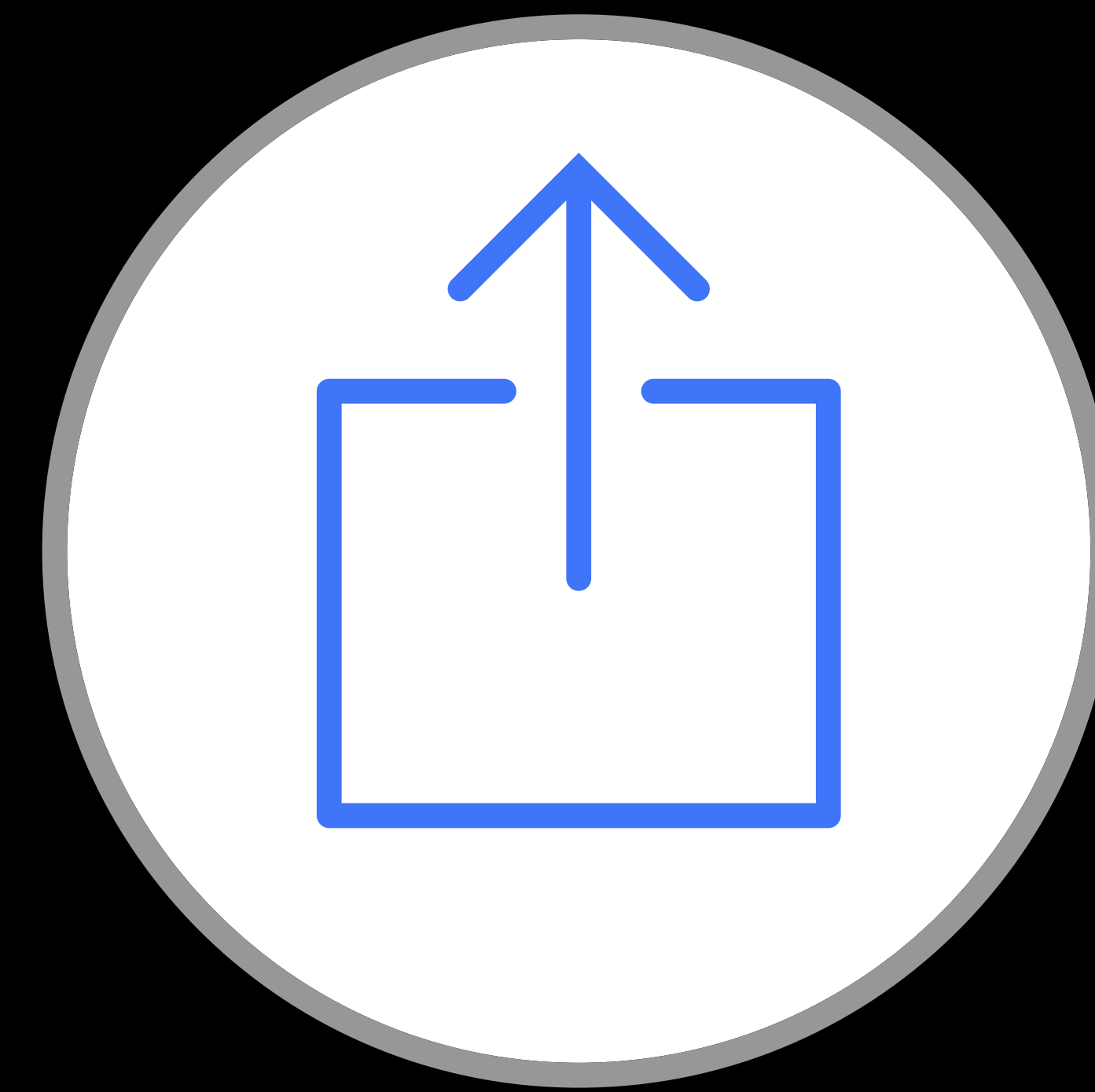
Share Extensions
