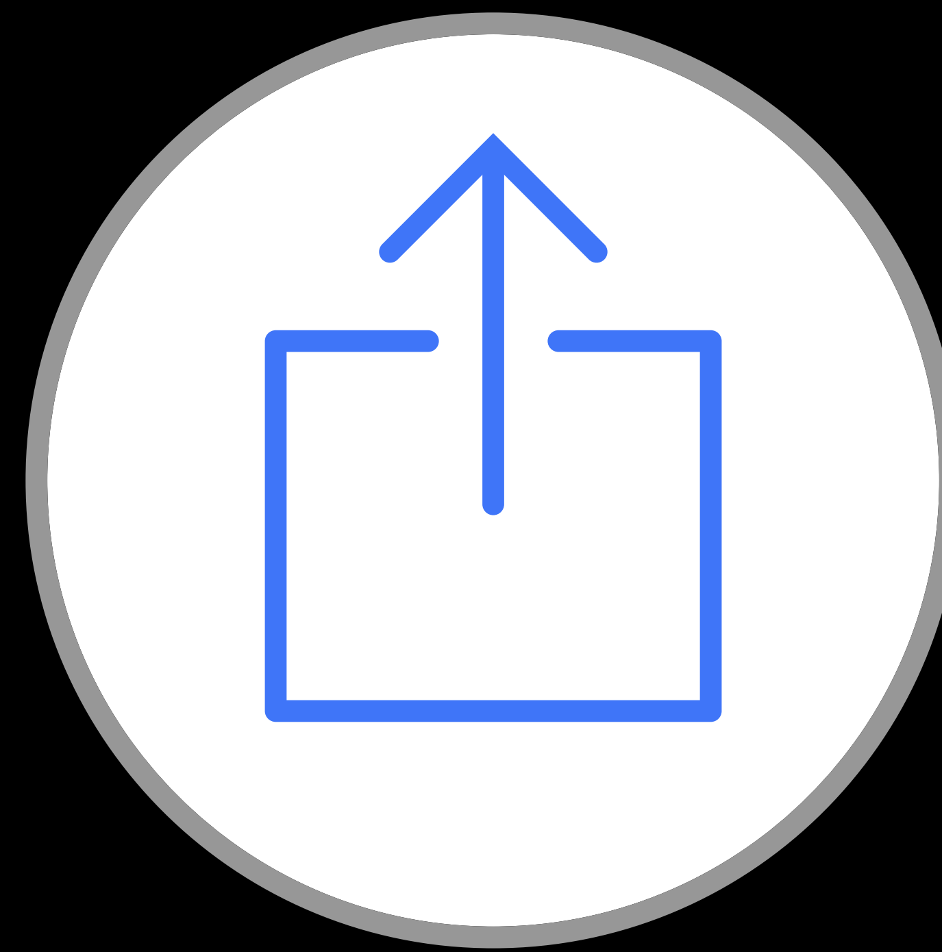
Share Extensions
