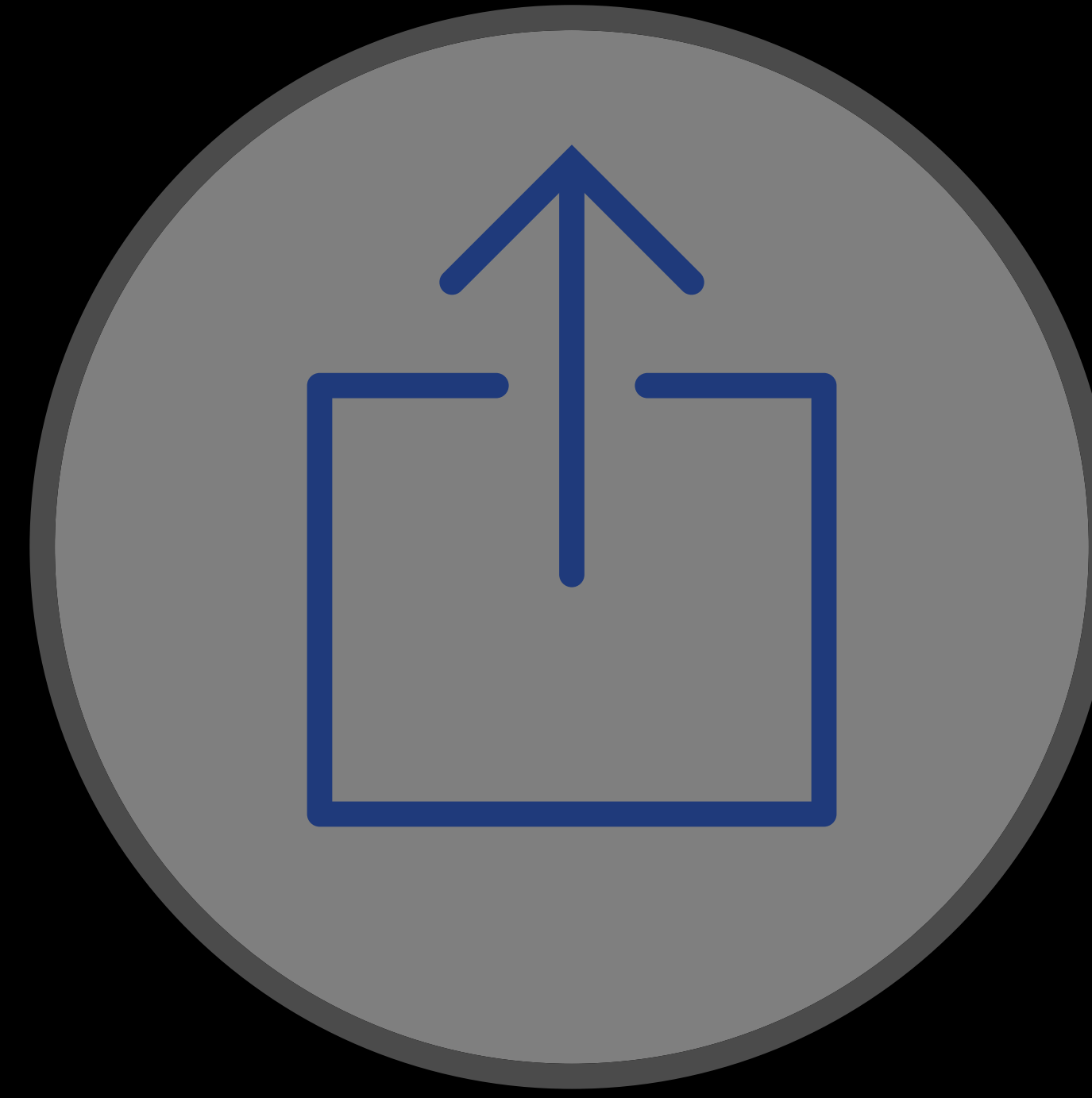
Share Extensions
