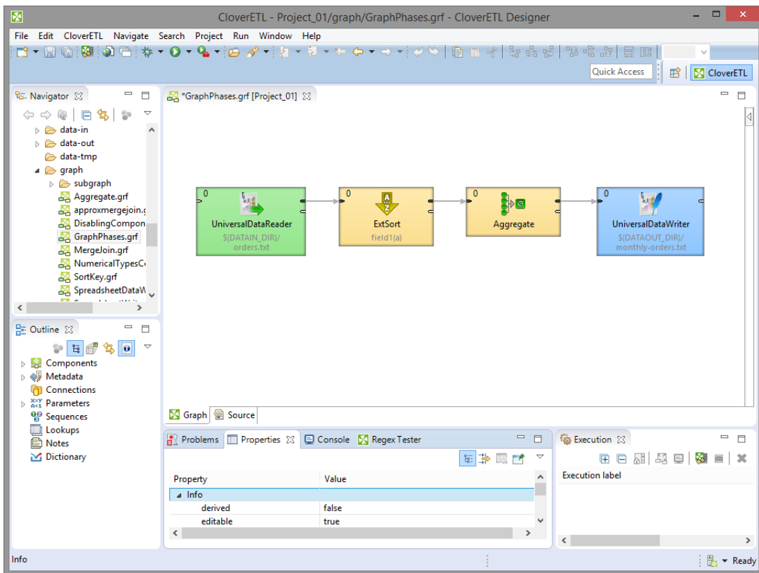
Figure 30.9. Running a Graph with Various Phases
