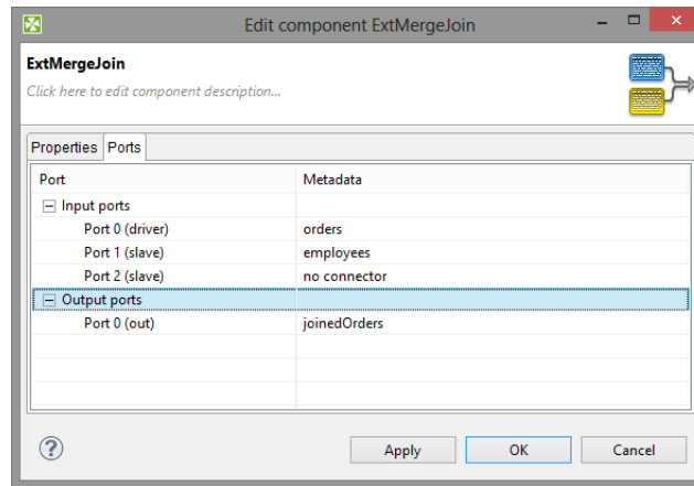
Figure 30.4. Edit Component Dialog (Ports Tab)
