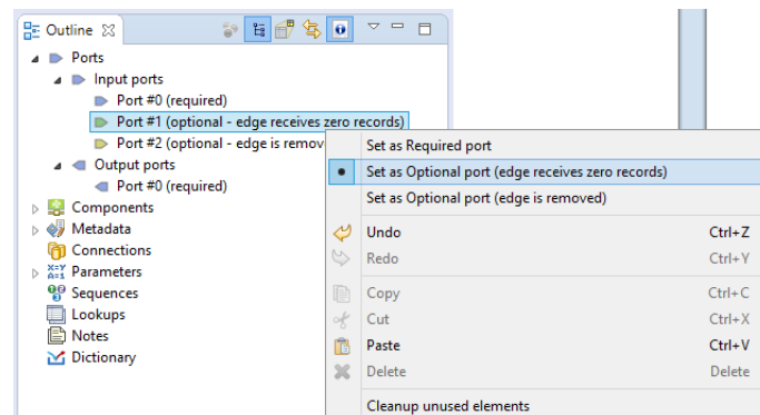
Figure 44.9. Setting up an Optional Port
