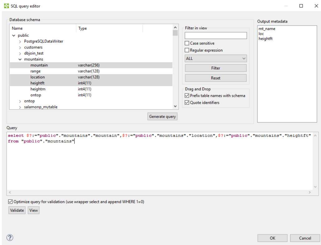
Figure 53.7. Generated Query with Question Marks
