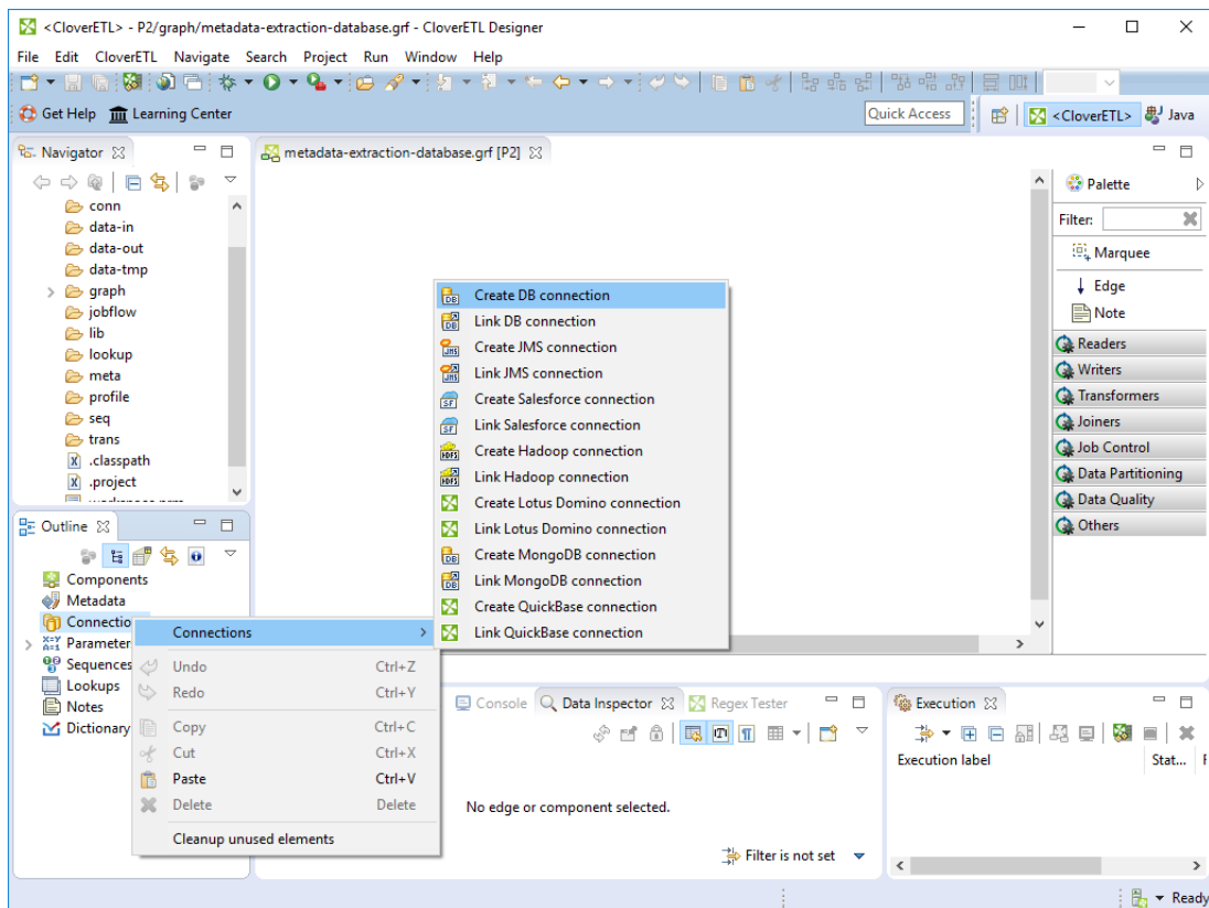
Figure 33.1. Creating Internal Database Connection
