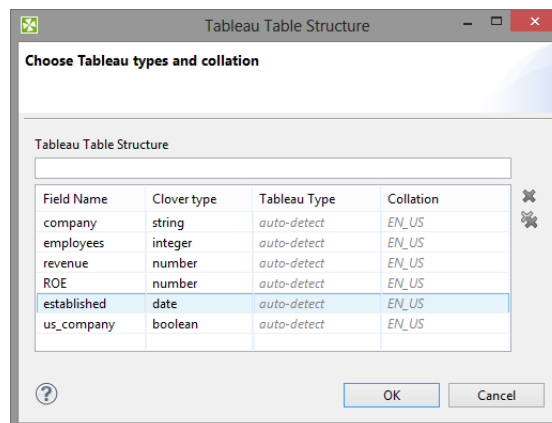
Figure 54.27. Tableau Table Structure
