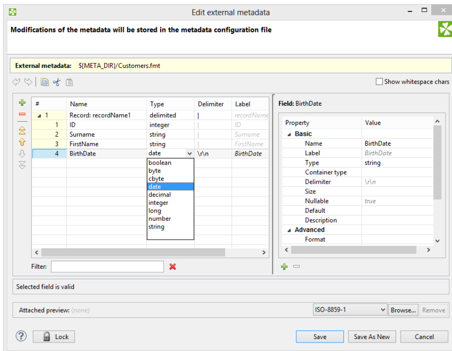
Figure 32.37. Metadata Editor for a Fixed Length File
