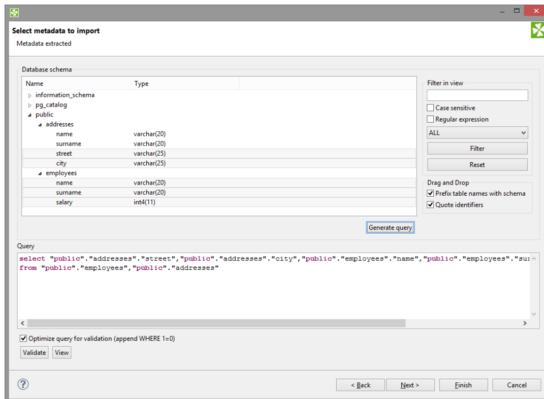
Figure 32.27. Generating a Query
