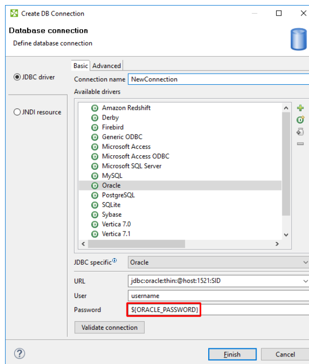
Figure 33.8. Using password from secure graph parameter
