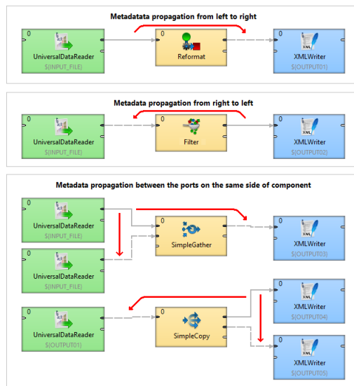
Figure 32.15. Overview of directions of metadata propagation
