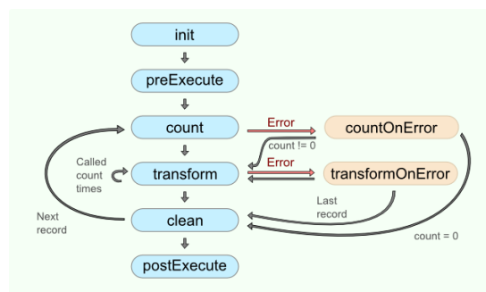
Figure 55.3. Normalizer code workflow
