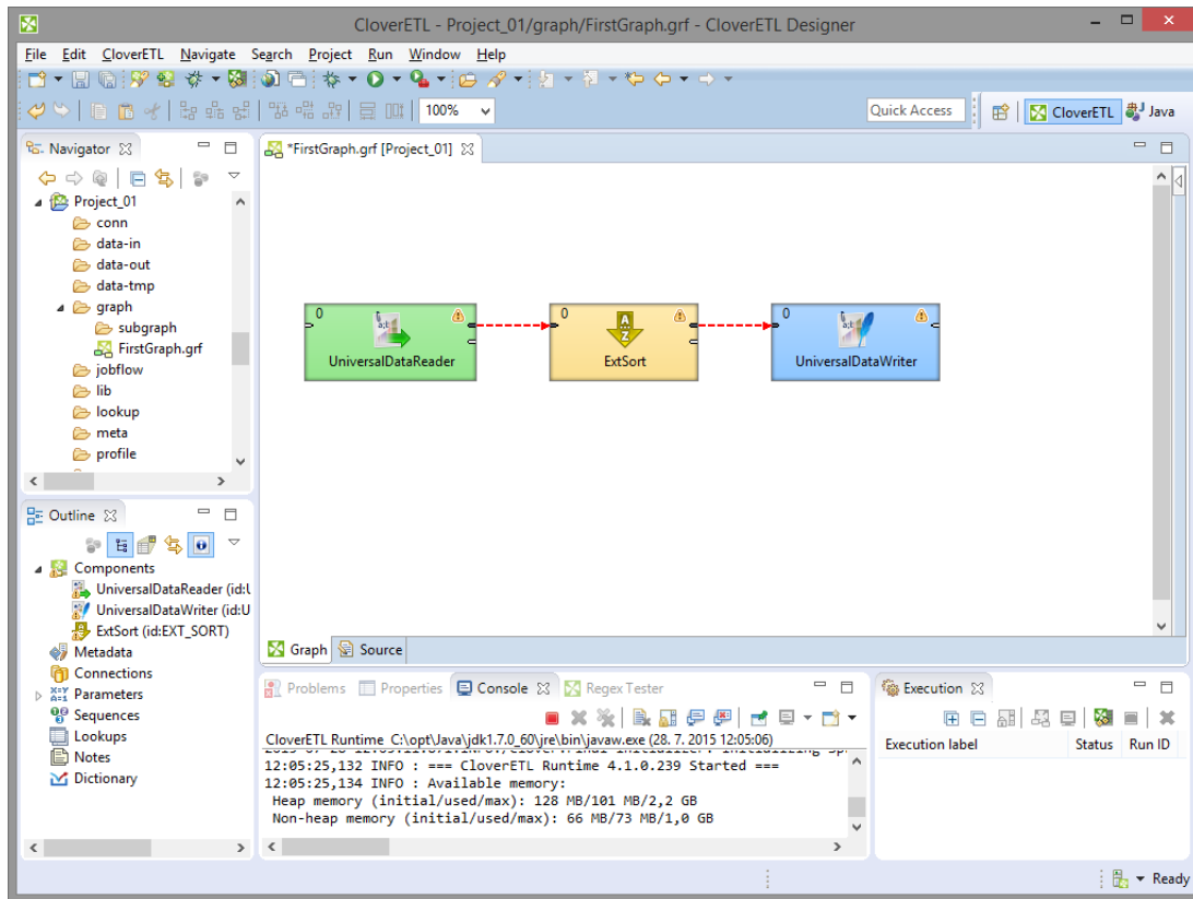
Figure 22.5. Components are Connected by Edges
