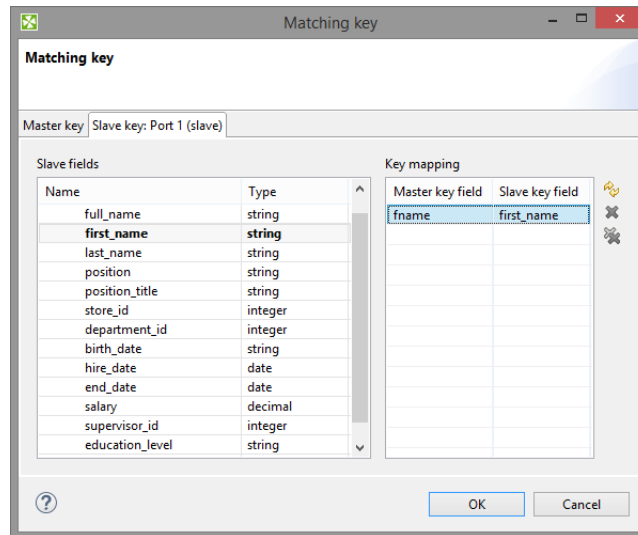
Figure 62.5. Matching Key Wizard (Slave Key Tab)
