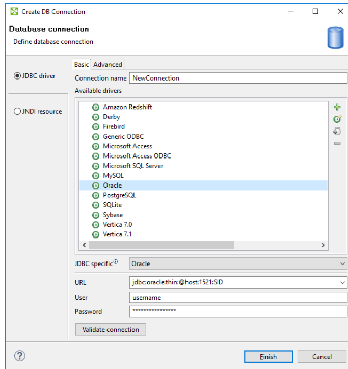
Figure 33.4. Database Connection Properties Dialog
