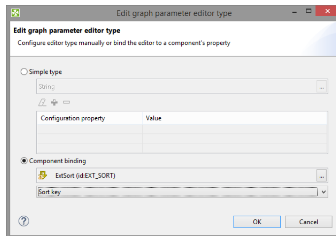
Figure 36.4. Graph Parameters Type Editor
