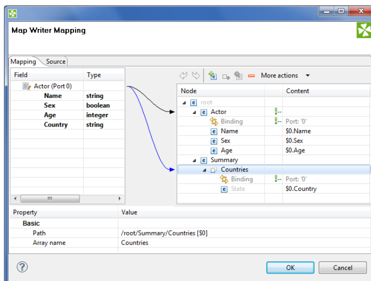
Figure 54.13. Mapping arrays in JavaMapWriter - notice the array contains a dummy element 'State' which you bind the input field to.
