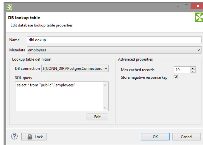
Figure 34.11. Database Lookup Table Wizard
