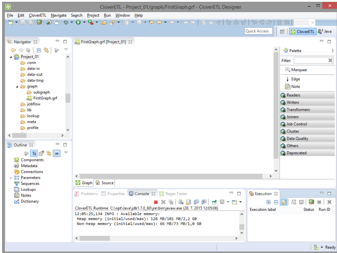
Figure 22.3. Graph Editor with a New Graph and the Palette of Components
