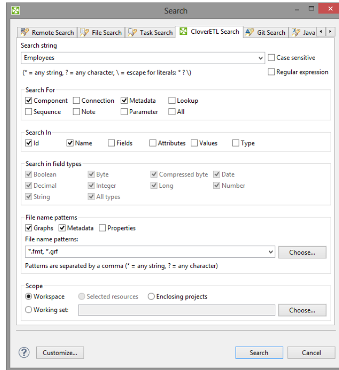
Figure 28.1. CloverETL Search Tab
