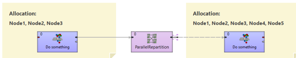
Figure 59.1. Usage example of ParallelRepartition component
