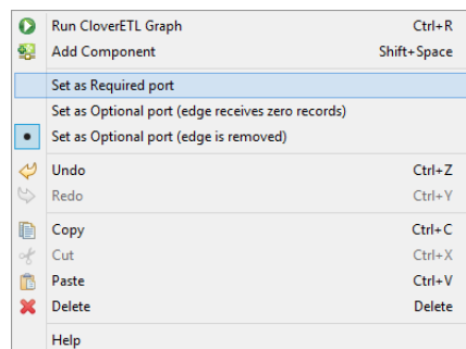
Figure 44.10. Setting up an Optional Port in Graph Editor
