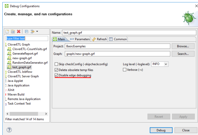
Figure 31.16. Debugging option in the Debug Configuration window
