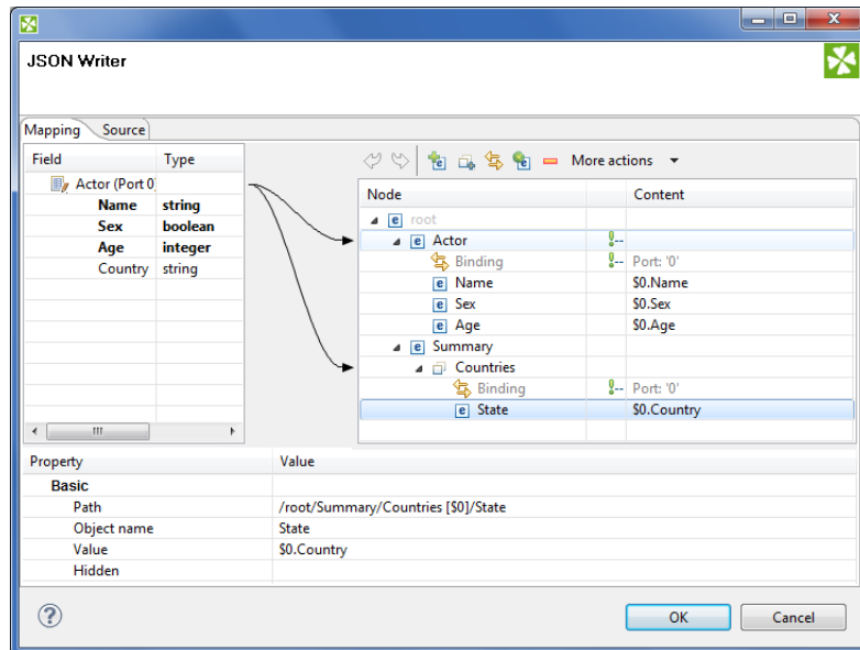
Figure 54.16. Mapping arrays in JSONWriter - notice the array contains a dummy element 'State' which you bind the input field to.
