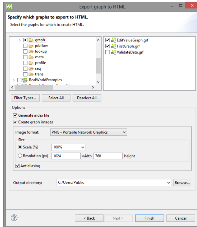
Figure 26.8. Export Graphs to HTML
