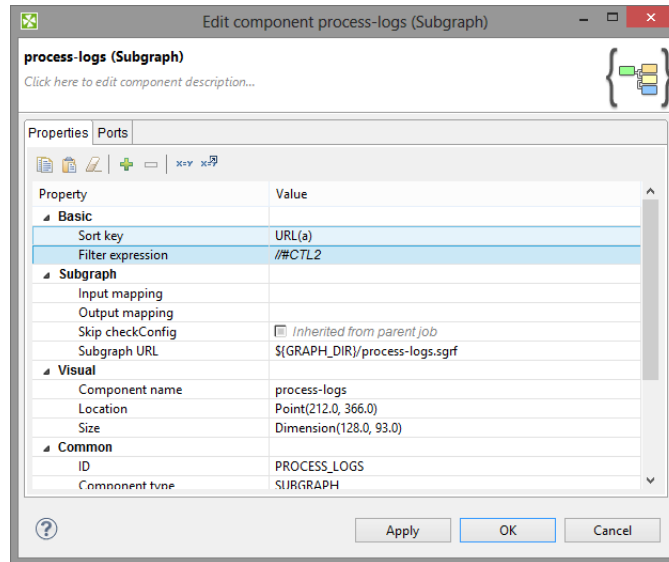
Figure 43.2. Example of User-defined Component
