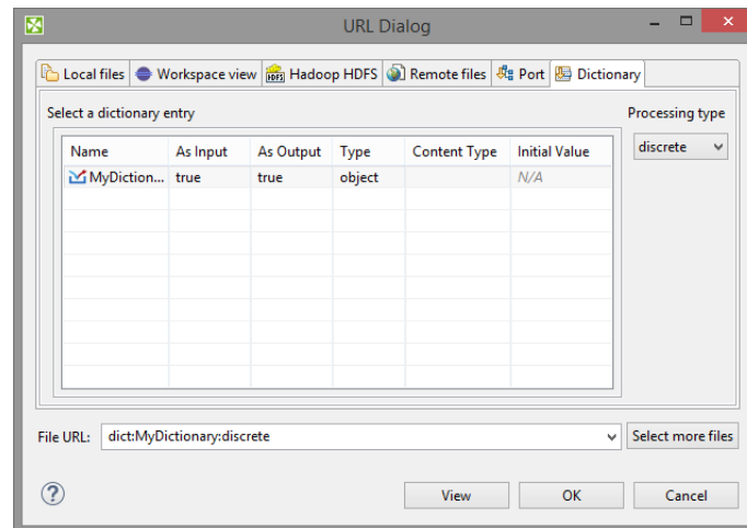
Figure 24.12. URL File Dialog - Dictionary
