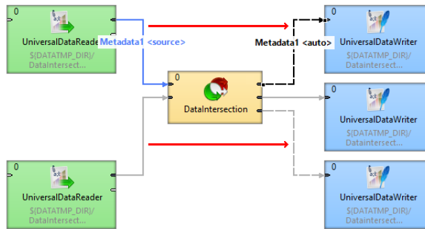
Figure 32.14. Advanced metadata propagation - DataIntersection
