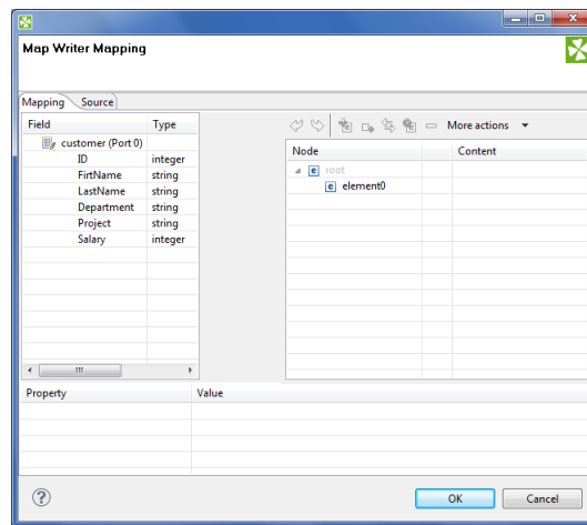
Figure 54.11. Mapping editor in JavaMapWriter after first open. Metadata on the input edge(s) are displayed on the left hand side. The right hand pane is where you design the desired output tree. Mapping is then performed by dragging metadata from left to right (and performing additional tasks described below).
