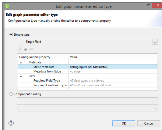
Figure 36.13. Single Field - Configuration
