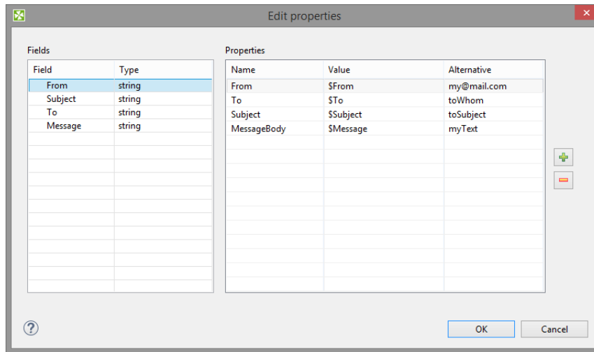
Figure 54.5. EmailSender Message Wizard
