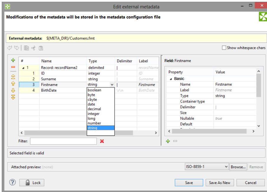
Figure 32.36. Metadata Editor for a Delimited File
