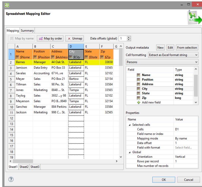
Figure 53.13. Basic Mapping – notice leading cells and dashed borders marking the area data will be taken from
