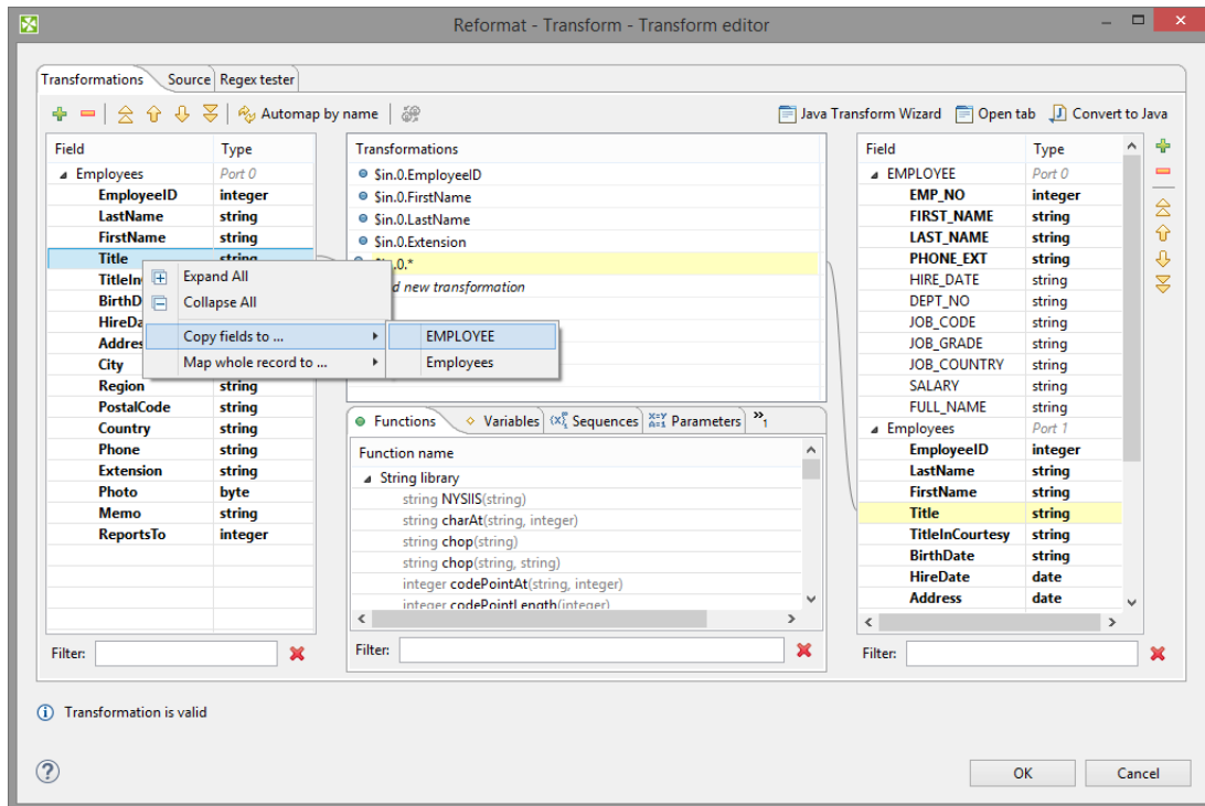
Figure 40.3. Copying the Input Field to the Output
