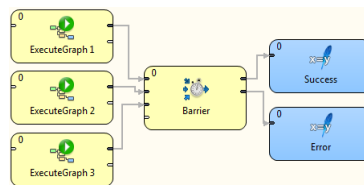
Figure 57.1. Example of typical usage of Barrier component
