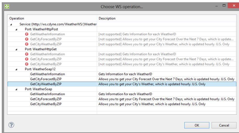
Figure 61.7. Choosing WS operation name in WebServiceClient .
