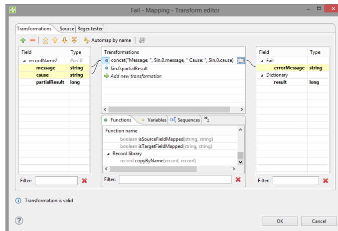
Figure 57.2. Example of mapping for Fail component
