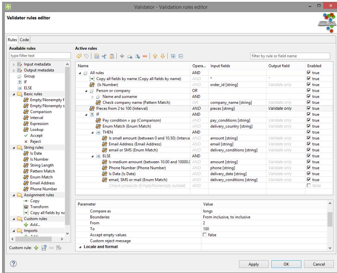
Figure 60.8. Validator rules editor
