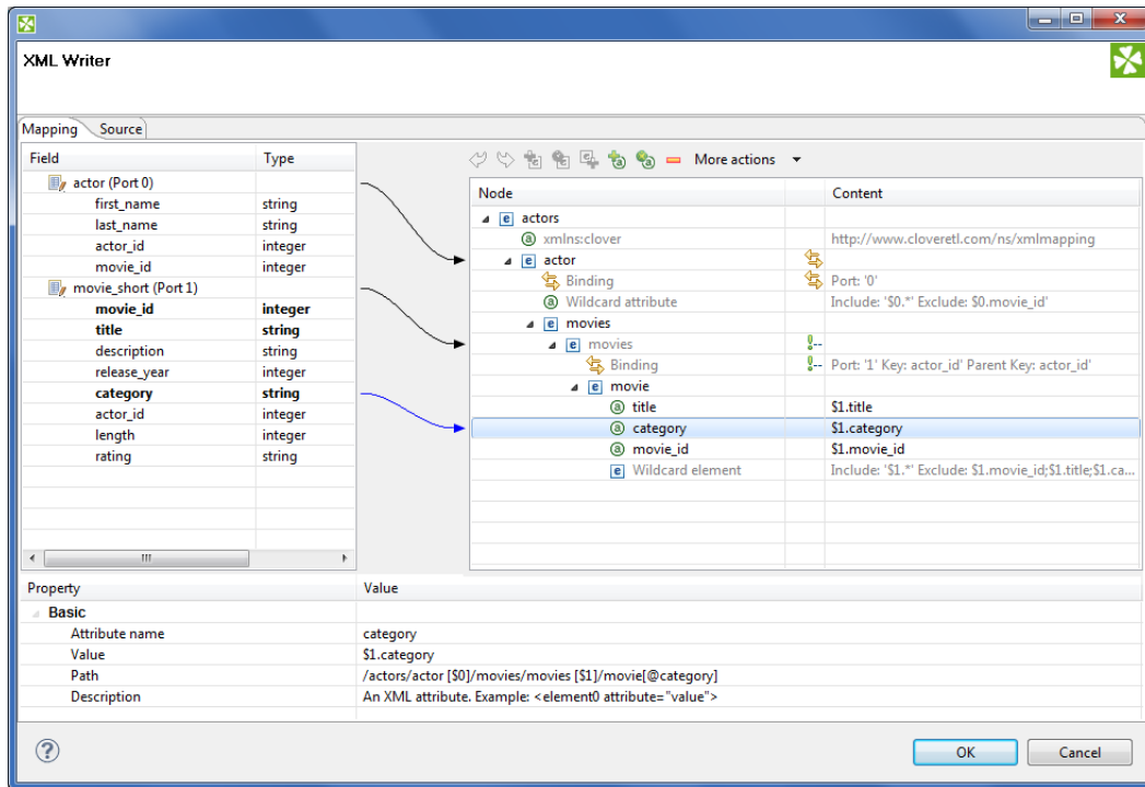
Figure 54.31. Attribute and its properties
