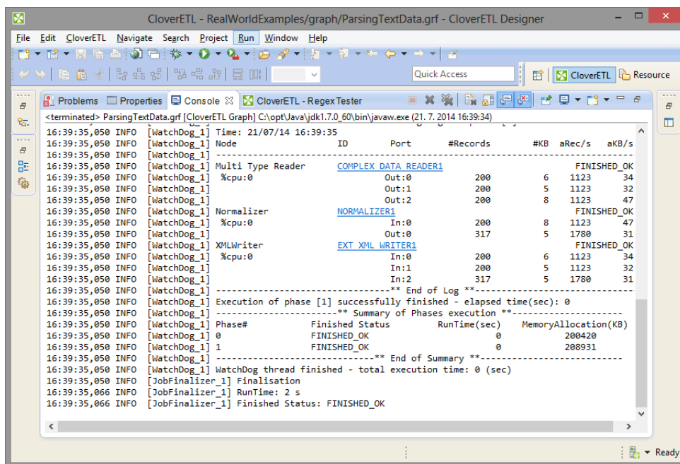
Figure 23.5. Console Tab with an Overview of the Graph Execution
