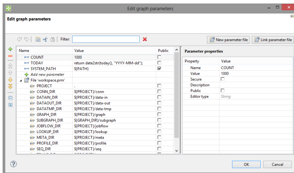
Figure 36.3. Example of a Graph parameters editor
