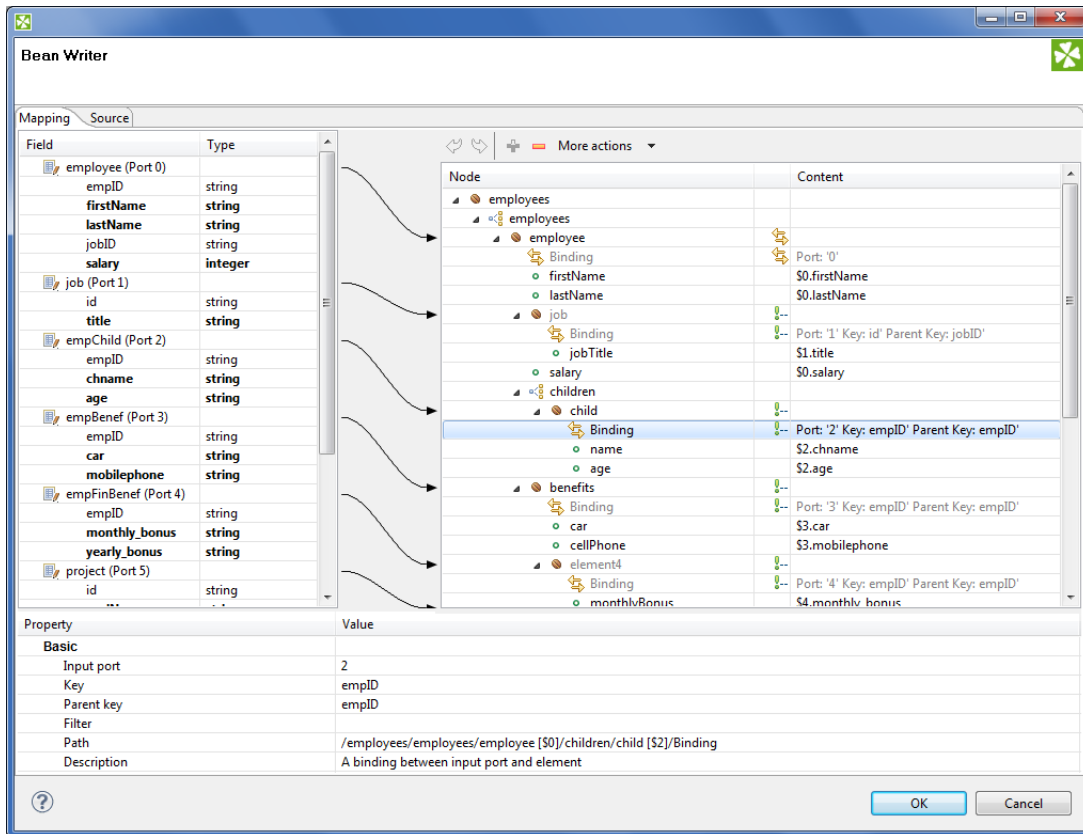
Figure 54.10. Example mapping in JavaBeanWriter - employees are joined with projects they work on. Fields in bold (their content) will be printed to the output dictionary, i.e. they are used in the mapping.
