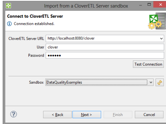
Figure 25.5. Import from CloverETL Server Sandbox Wizard (Connect to CloverETL Server)
