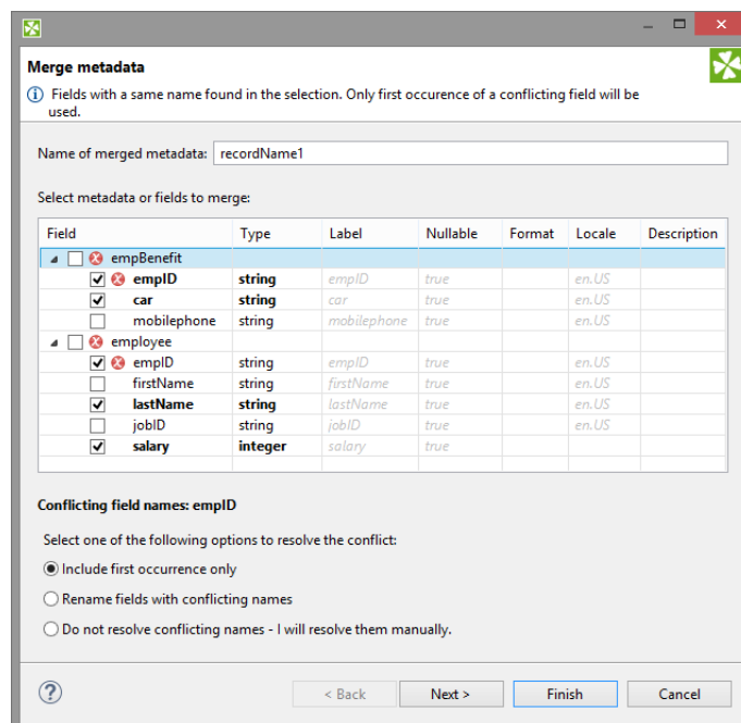
Figure 32.34. Merging two metadata - conflicts can be resolved in one of the three ways (notice radio buttons at the bottom).
