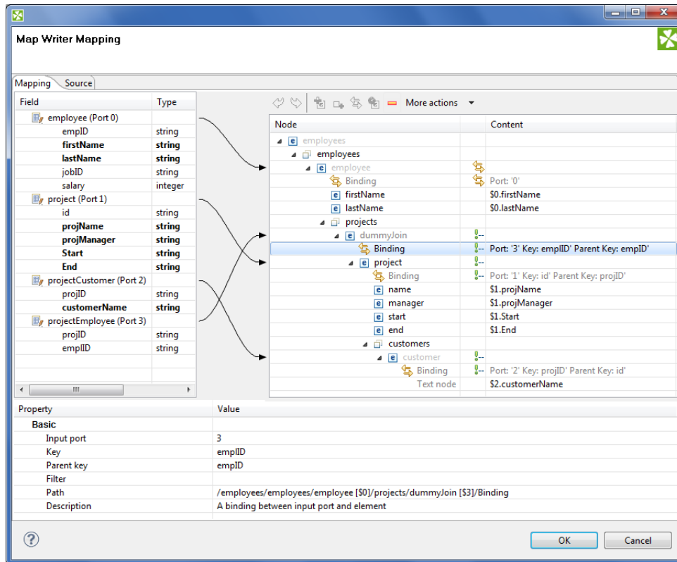
Figure 54.12. Example mapping in JavaMapWriter - employees are joined with projects they work on. Fields in bold (their content) will be printed to the output dictionary.
