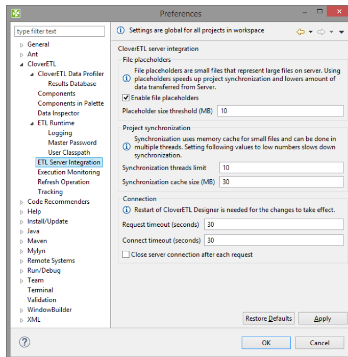
Figure 15.1. ETL Server Integration
