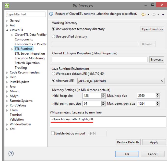
Figure 33.10. Adding path to the native dll to VM parameters.
