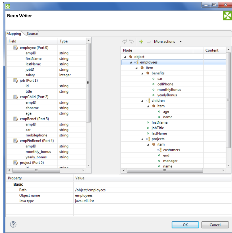
Figure 54.9. Mapping editor in JavaBeanWriter after first open. Metadata on the input edge(s) are displayed on the left hand side. The right hand pane is where you design the desired output tree - it is pre-defined by your bean's structure (note: in the example, the bean contains employees and projects they are working on). Mapping is then performed by dragging metadata from left to right (and performing additional tasks described below).
