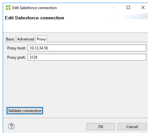
Figure 33.21. Salesforce Connection Dialog III
