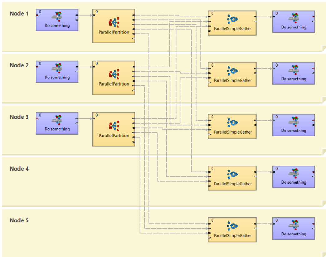
Figure 59.2. Example of actual working of ParallelRepartition component in runtime
