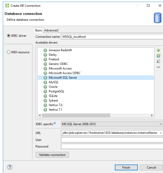
Figure 33.9. Connecting to MS SQL with Windows authentication.
