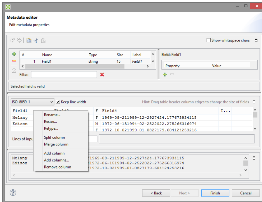
Figure 32.21. Setting Up Fixed Length Metadata
