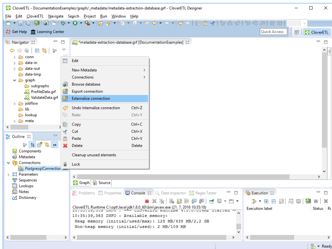
Figure 33.2. Externalizing Internal Database Connection
