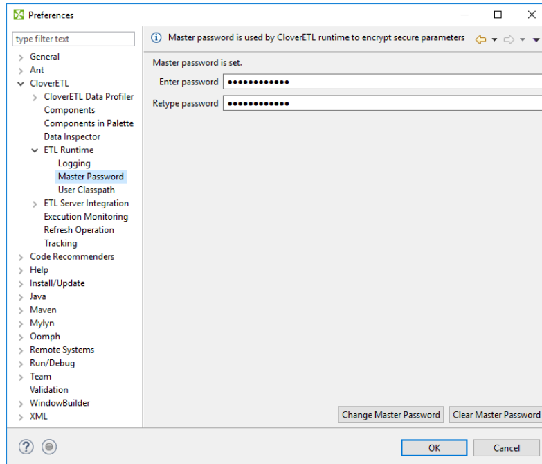
Figure 14.6. Setting the Master password
