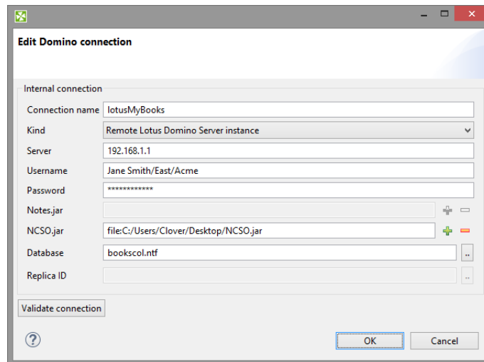
Figure 33.14. Lotus Notes Connection Dialog
