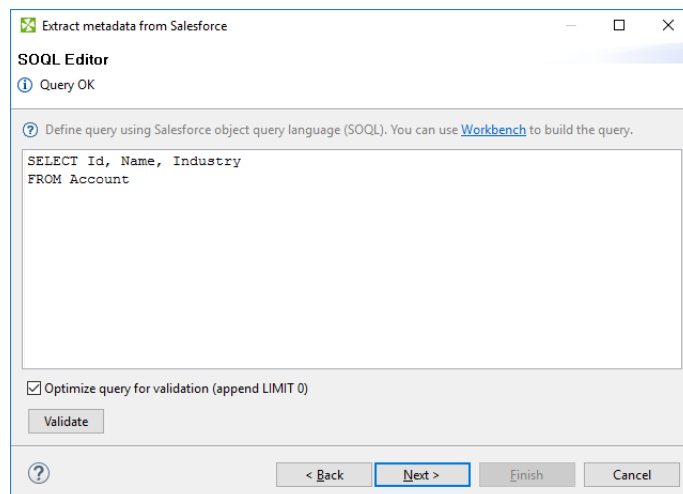
Figure 32.30. Extract metadata from Salesforce - enter SOQL query
