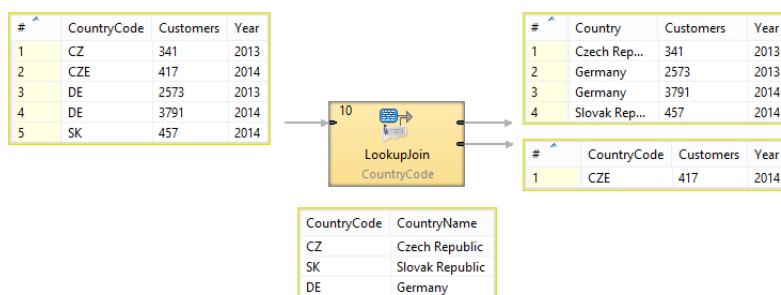
Figure 56.5. LookupJoin - how it works
