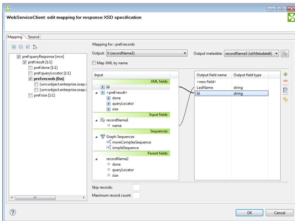
Figure 53.20. The Mapping Dialog for XMLExtract
