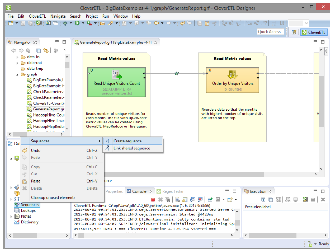
Figure 35.1. Creating a Sequence
