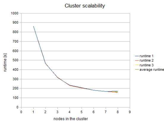
Figure 29.7. Cluster Scalability
