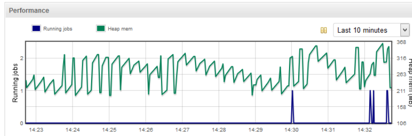
Figure 16.2. Performance
