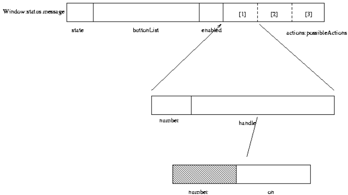
Figure 4.3: Bytes of a Window:status Message
