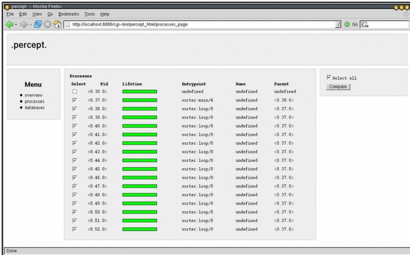
Figure 1.2: Processes selection
