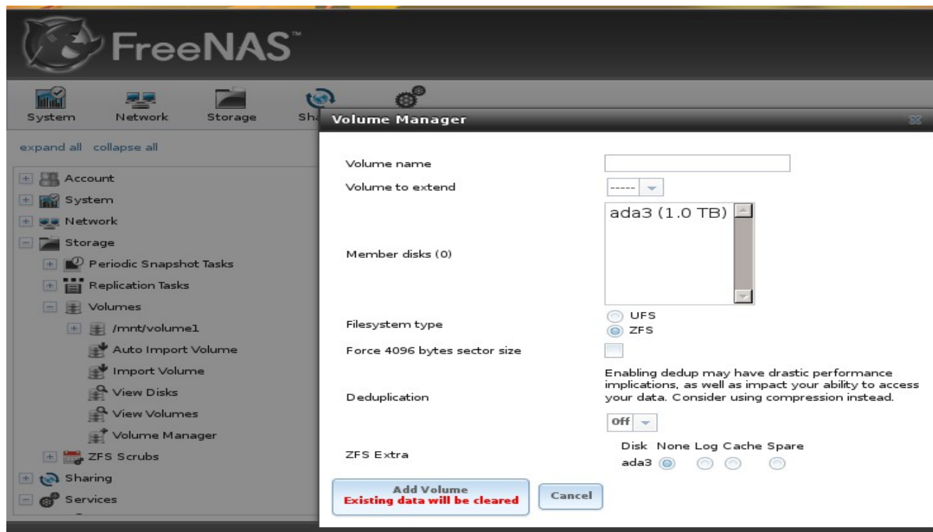
Figure 6.3d: Volume to Extend Field
