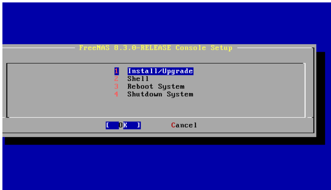
Figure 2.3a: FreeNAS® Console Setup
