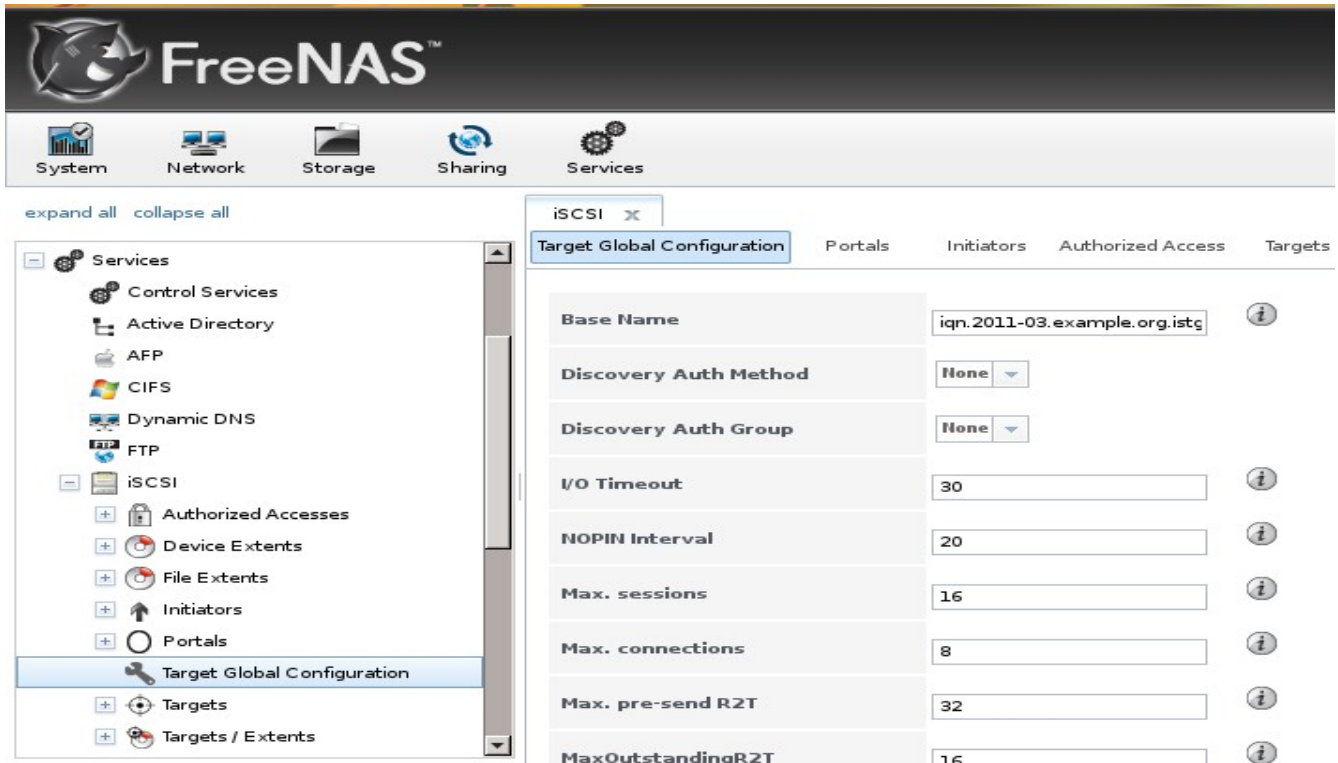
Figure 8.7h: iSCSI Target Global Configuration Variables
