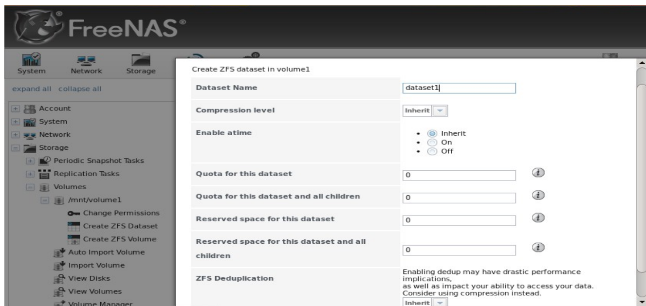
Figure 6.3e: Creating a ZFS Dataset
