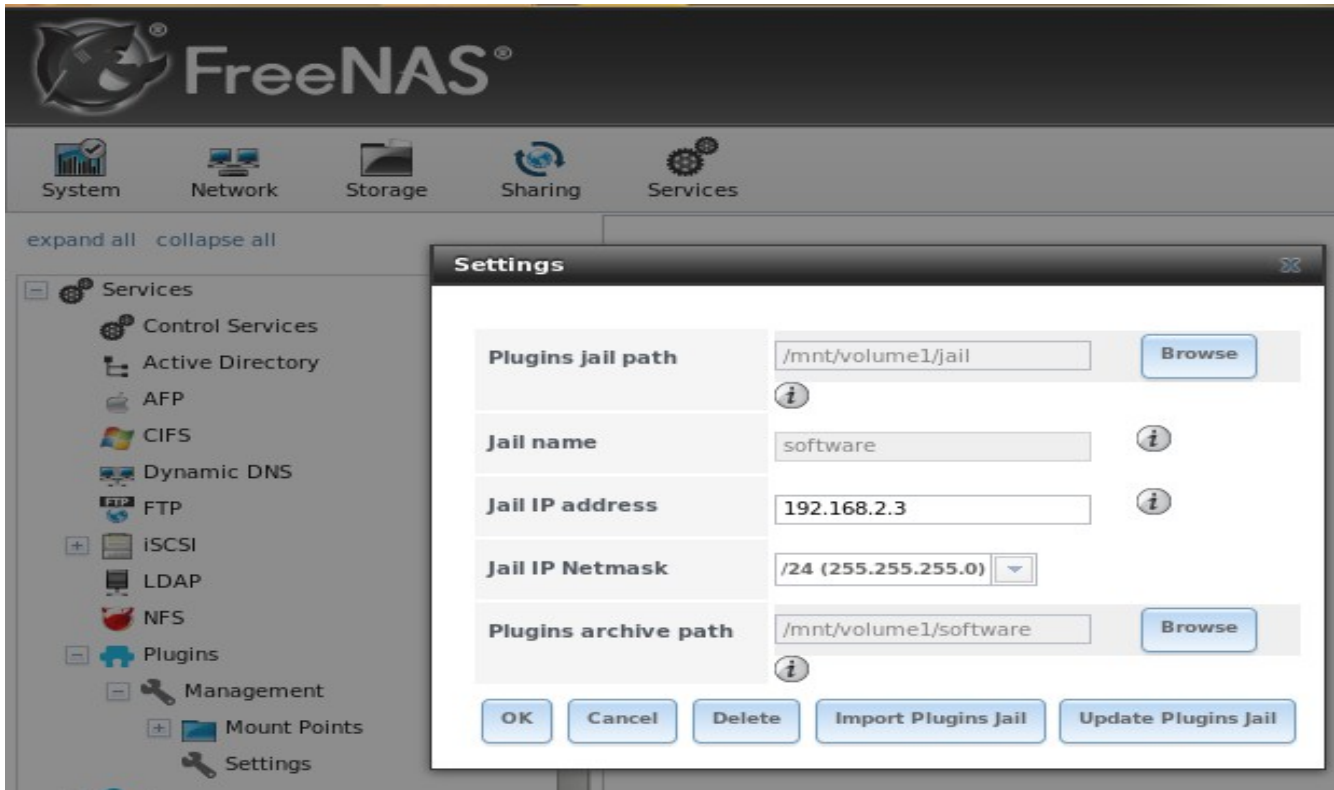
Figure 8.10b: Plugins Jail Settings
