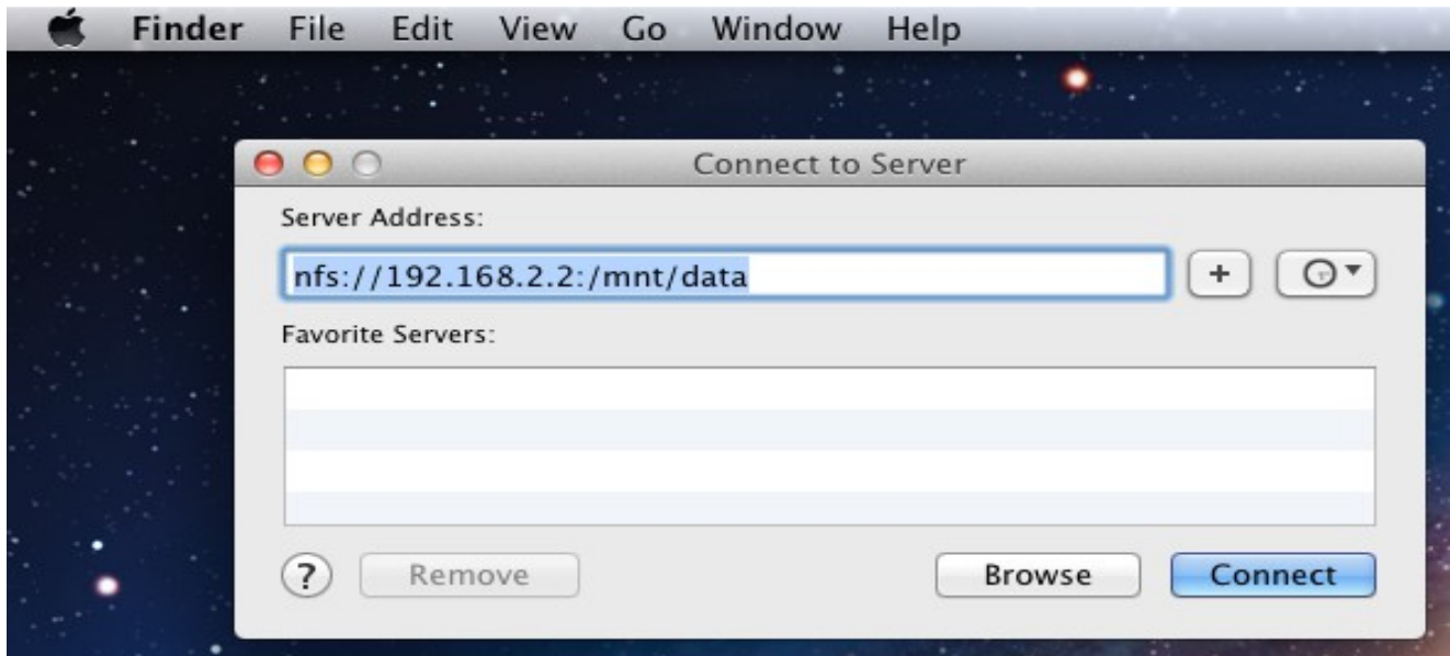
Figure 7.2c: Mounting the NFS Share from Mac OS X
