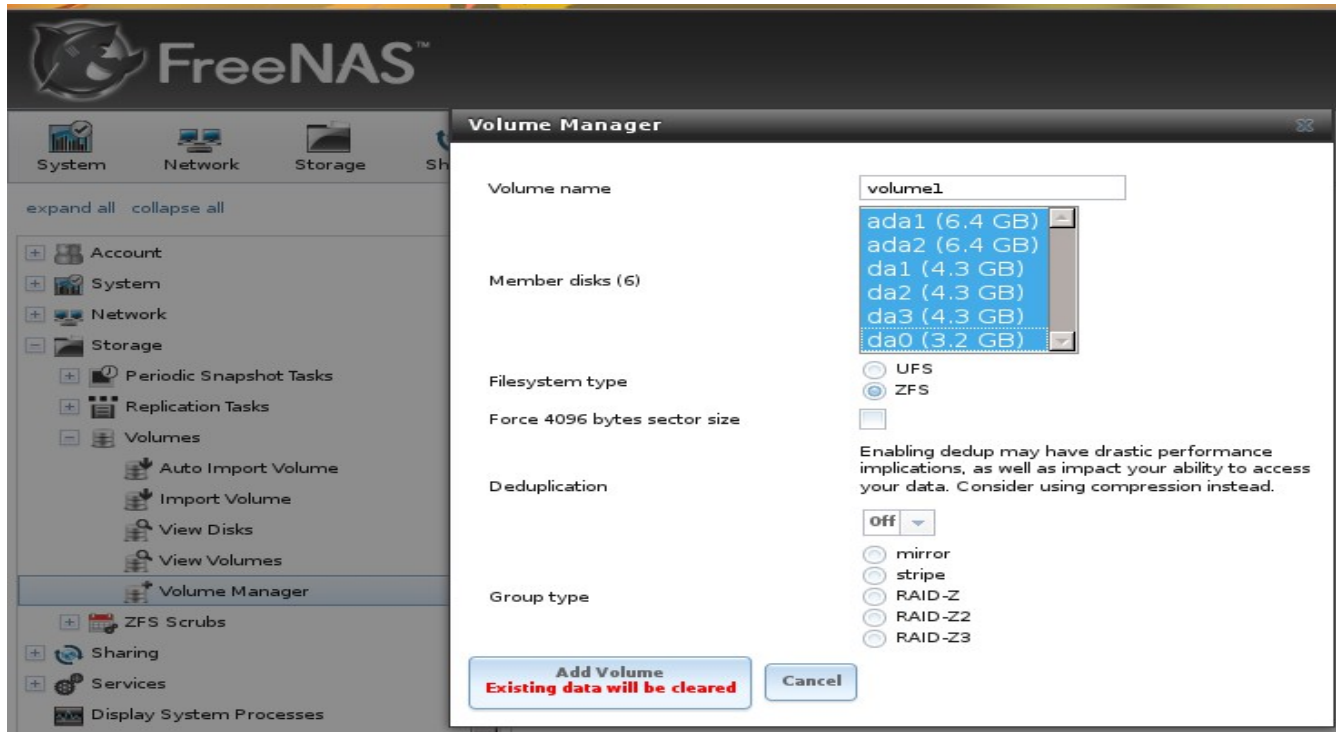
Figure 6.3c: Creating a ZFS Pool Using Volume Manager
