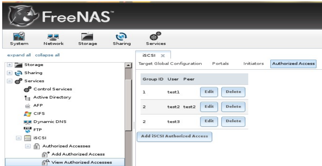
Figure 8.7b: Viewing Authorized Accesses
