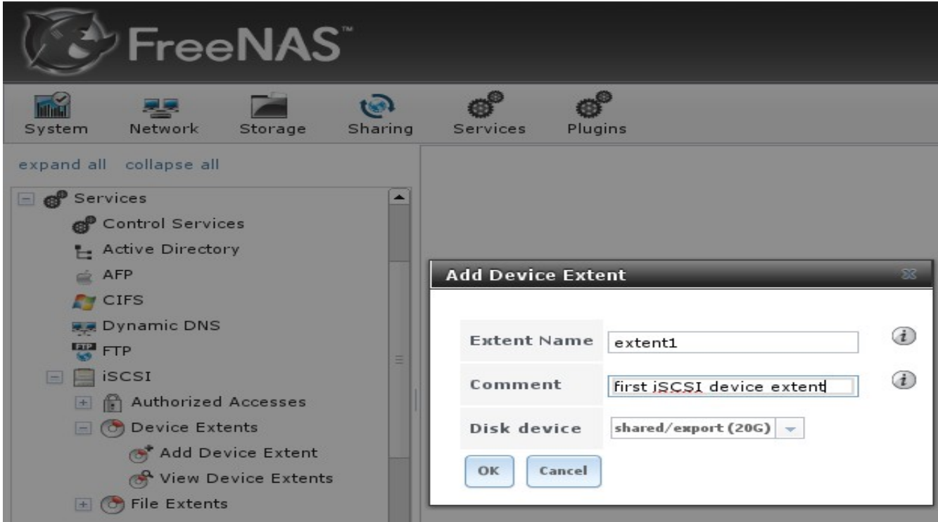
Figure 8.7c: Adding an iSCSI Device Extent
