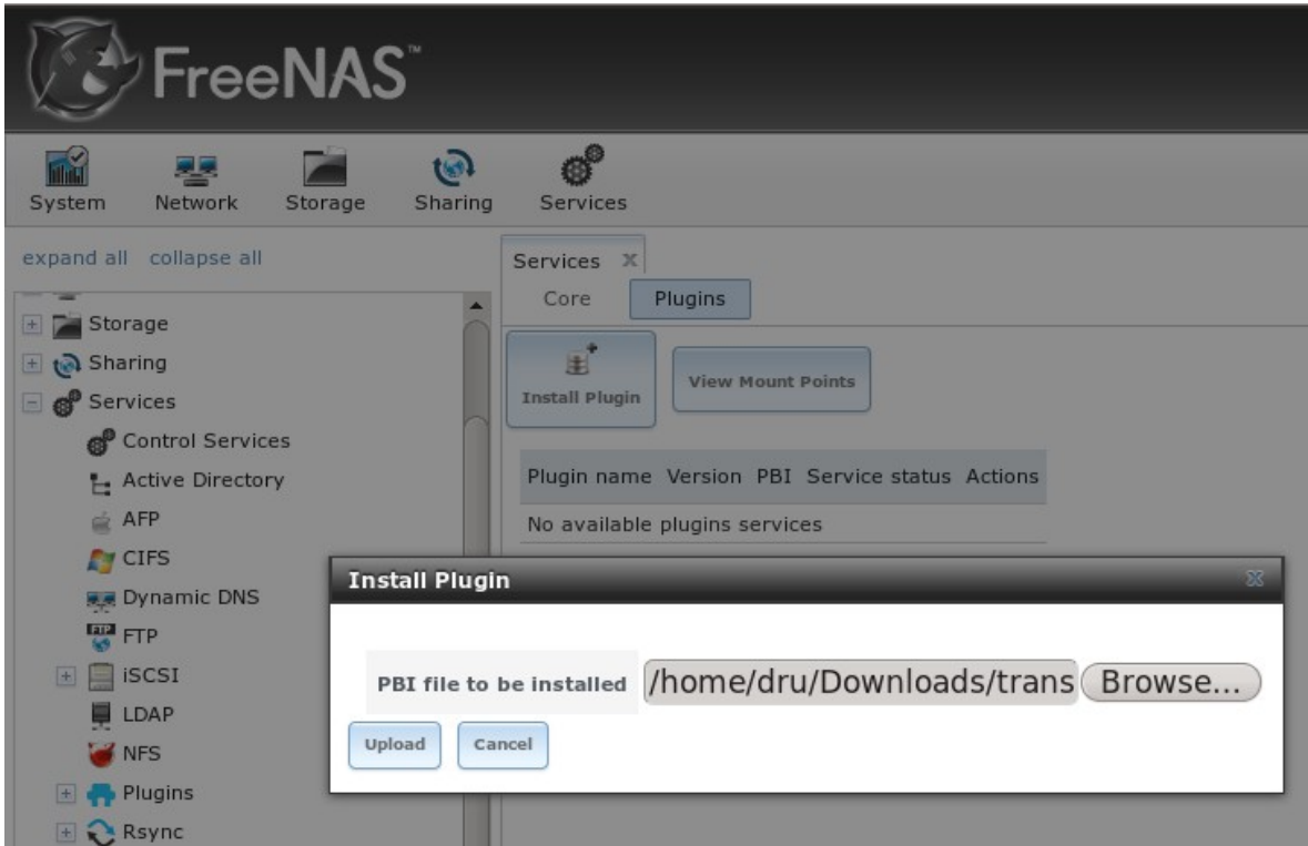
Figure 8.10e: Installing a PBI
