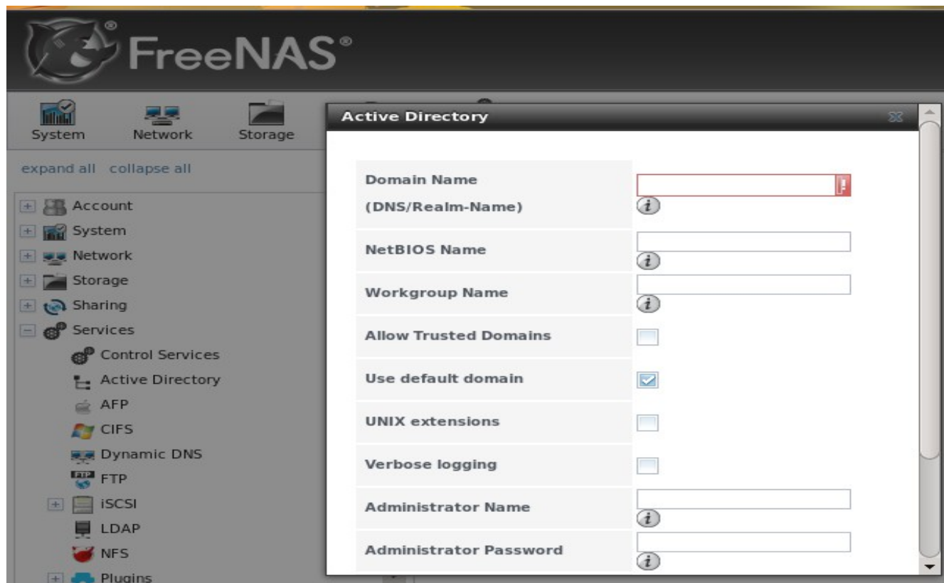
Figure 8.2a: Configuring Active Directory
