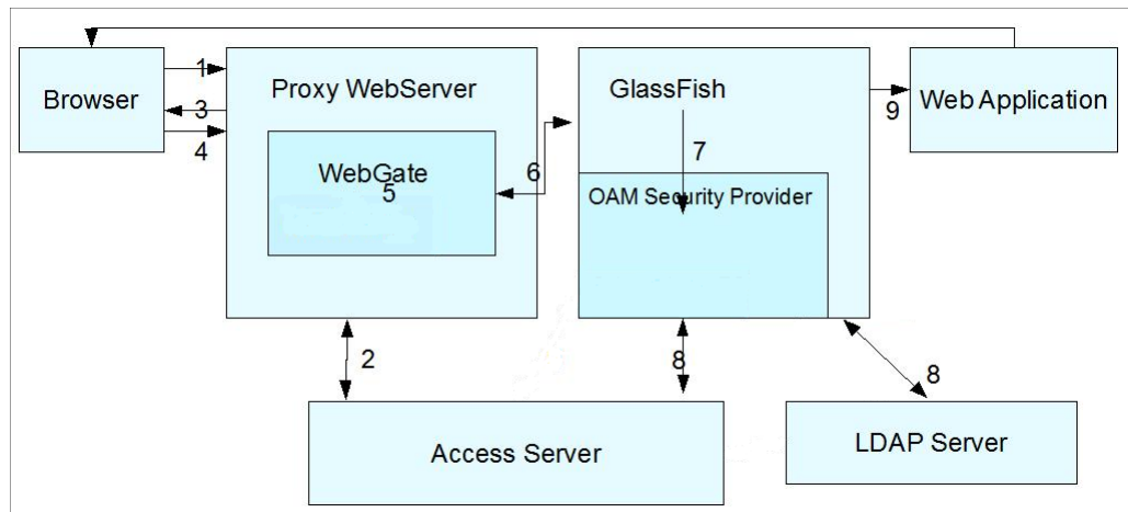
Figure 7-2 Identity Assertion via WebGate
