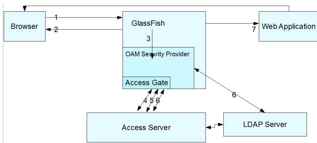
Figure 7-1 Authentication (FORM/BASIC) for Web resources Via AccessGate
