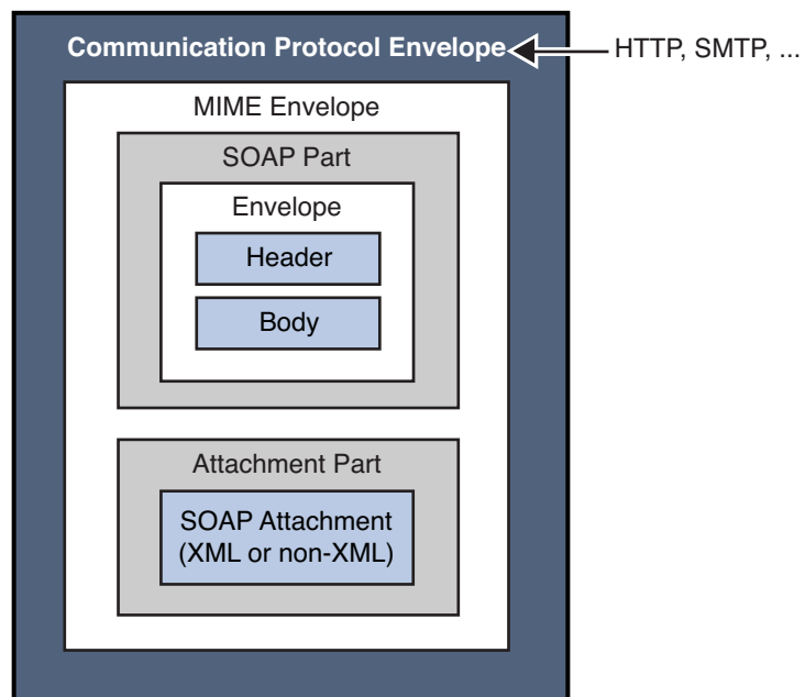
Figure 5-4 SOAP Message with Attachments
