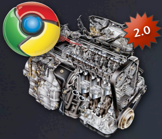
Chrome's V8
