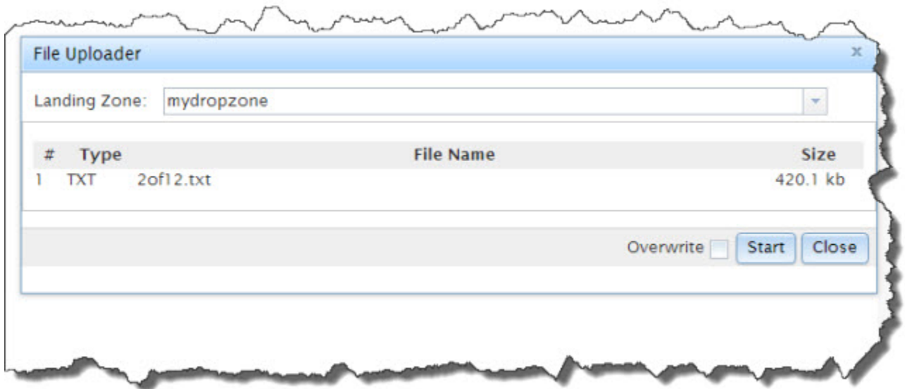
Figure 21. File Uploader
