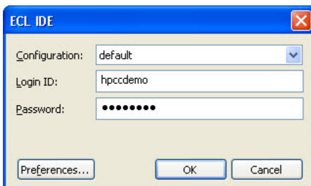
Figure 12. Login Window
