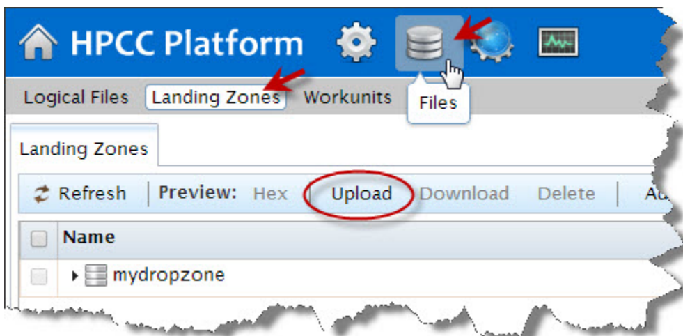
Figure 31. Upload/download
