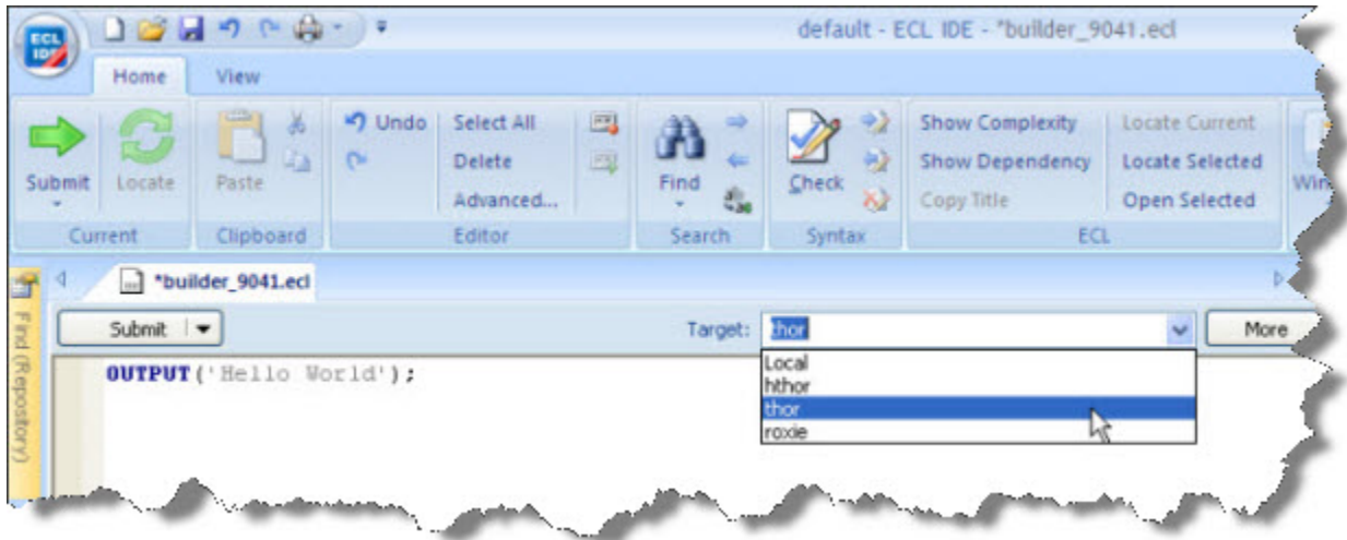
Figure 14. Select target
