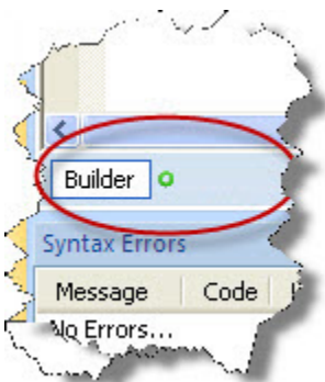
Figure 27. Compiled
