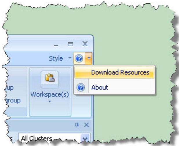
Figure 35. Help Menu
