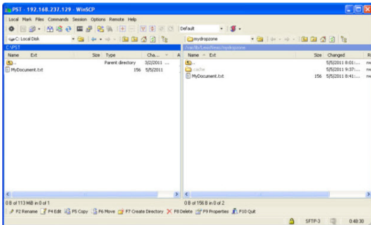
Figure 33. WinSCP
