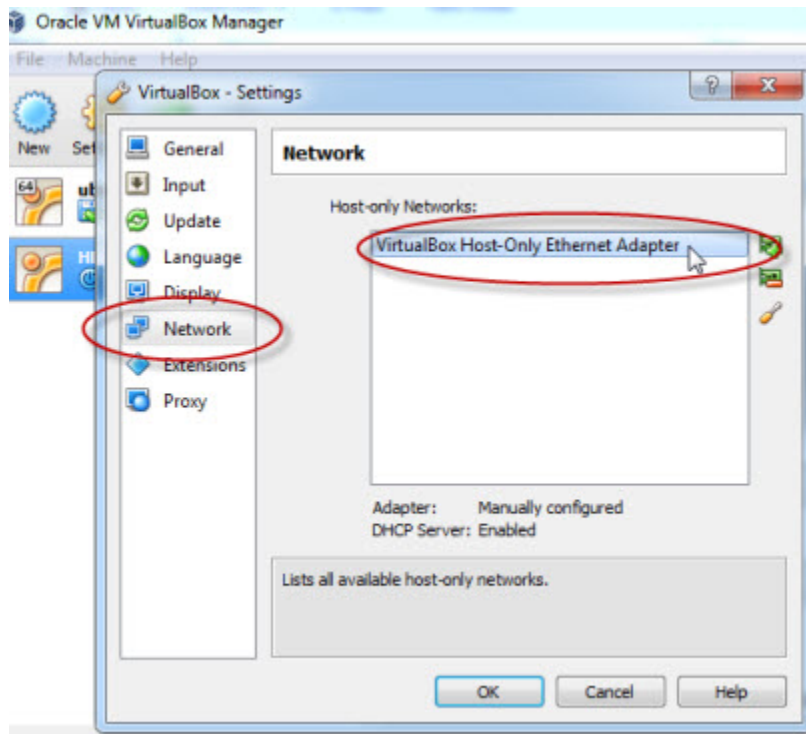
Figure 1. VirtualBox - Settings
