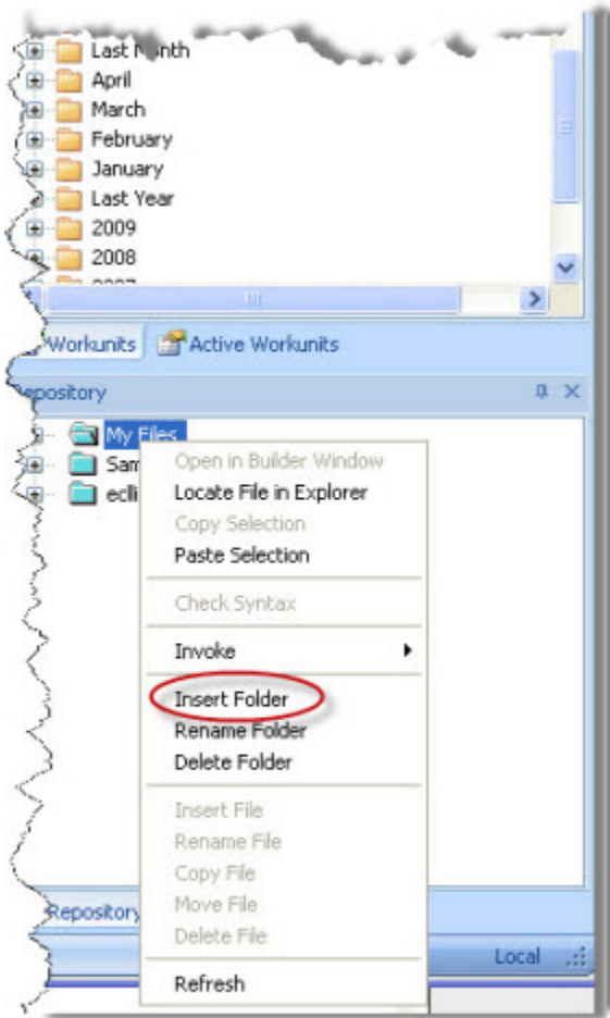
Figure 23. Insert Folder
