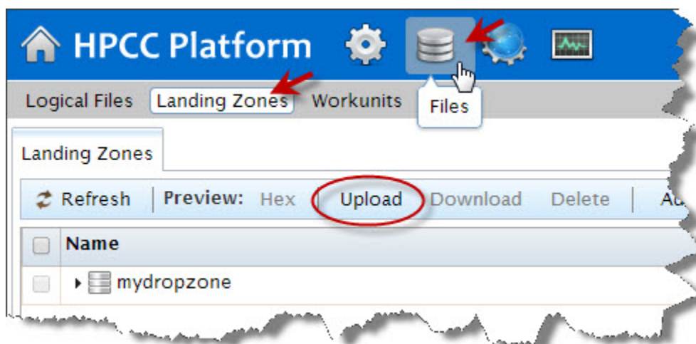
Figure 20. Upload
