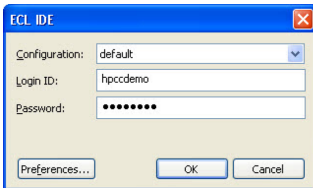
Figure 13. Login Window
