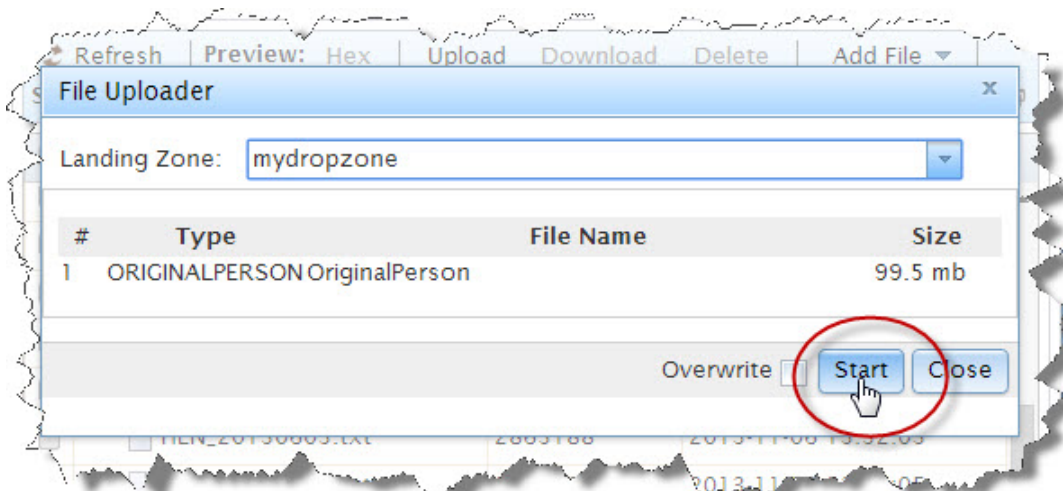
Figure 32. Dropzones
