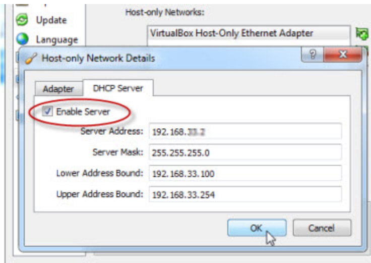
Figure 2. Network Details
