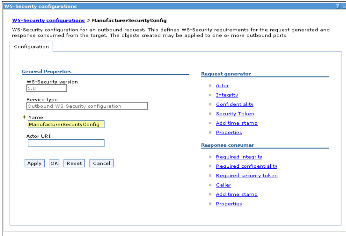
Figure 11-54 WS-Security configuration
