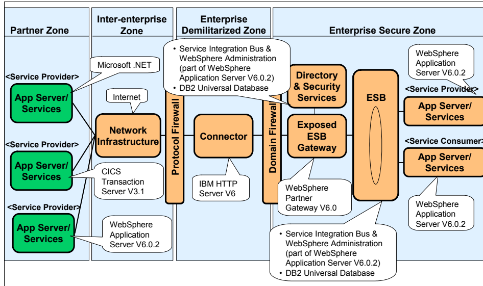
Figure 7-4 Exposed Router variation: SOA profile product mapping
