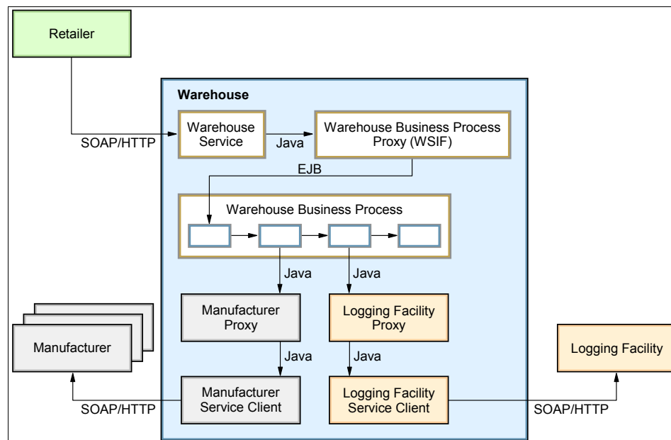
Figure 14-3 Scenario implementation for the Exposed Serial Process
