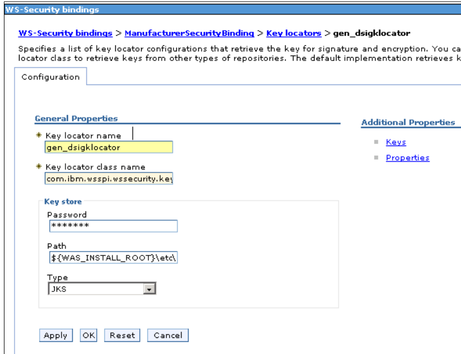
Figure 11-61 Creating a key locator
