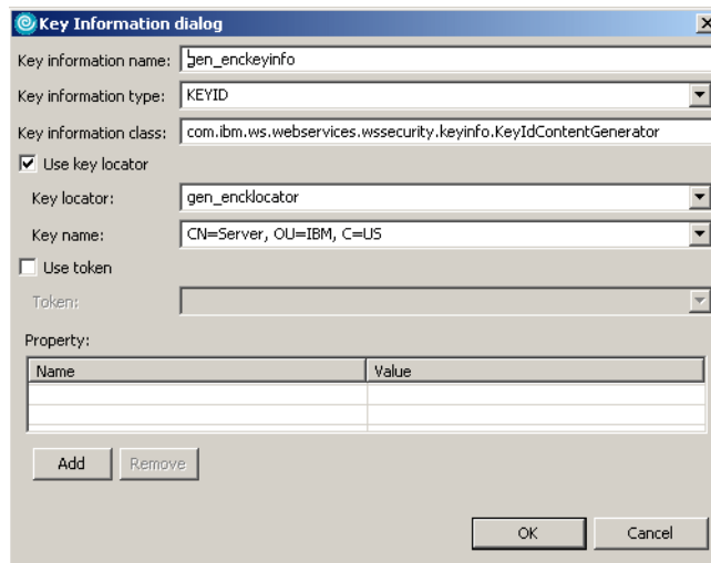
Figure 10-33 Key Information dialog for body content encryption
