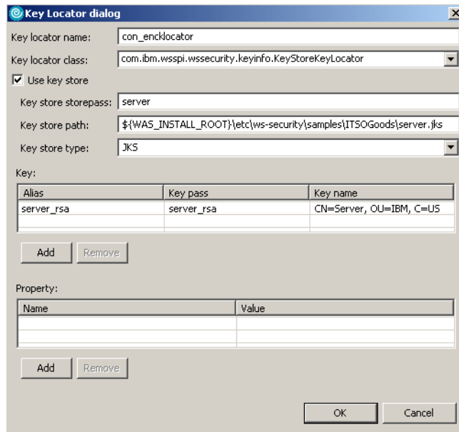
Figure 10-37 Key Locator dialog for body content decryption
