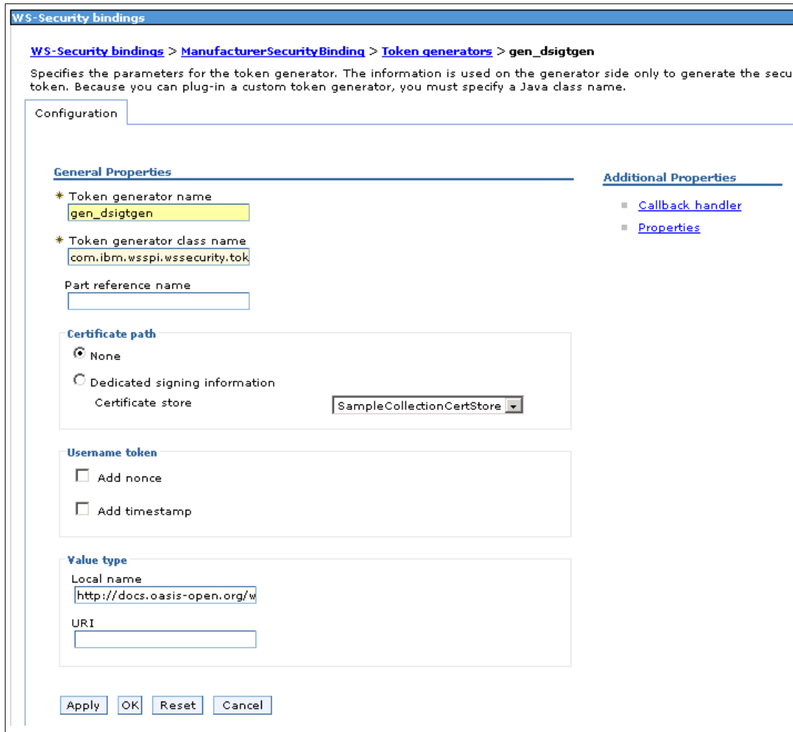
Figure 11-58 Creating a token generator
