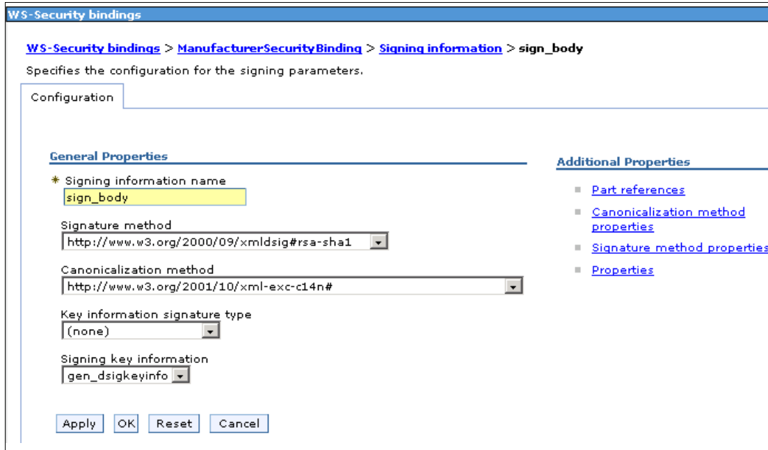
Figure 11-63 Creating the signing information
