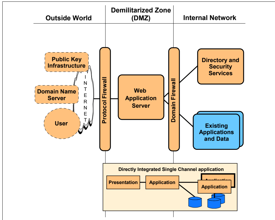
Figure 2-6 Directly Integrated Single Channel application pattern::Runtime pattern
