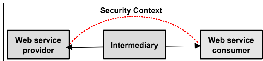
Figure 10-10 End-to-end security with message-level security
