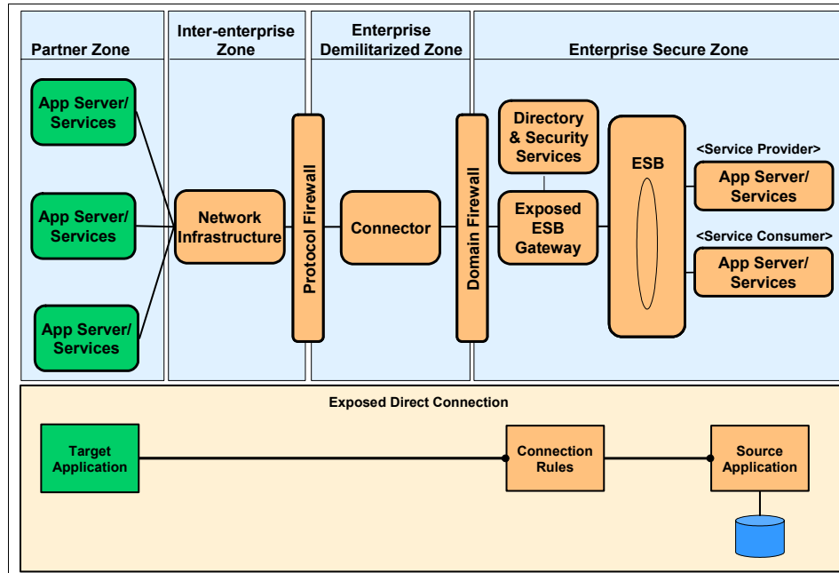
Figure 6-3 Exposed Direct Connection runtime pattern: SOA profile
