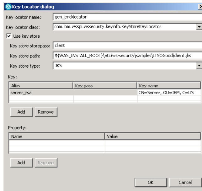
Figure 10-32 Key Locator dialog for body content encryption
