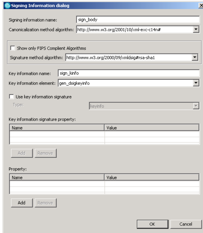
Figure 10-20 Signing Information dialog for signing by an X.509 certificate token
