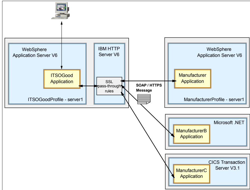
Figure 10-40 Solution topology
