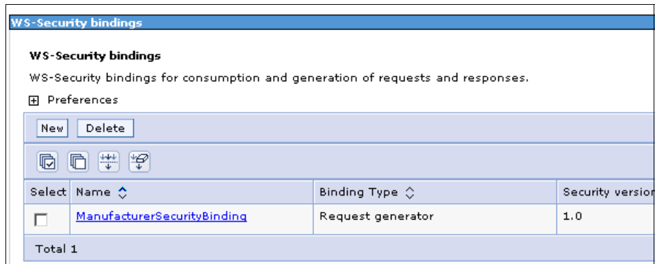
Figure 11-53 WS-Security bindings
