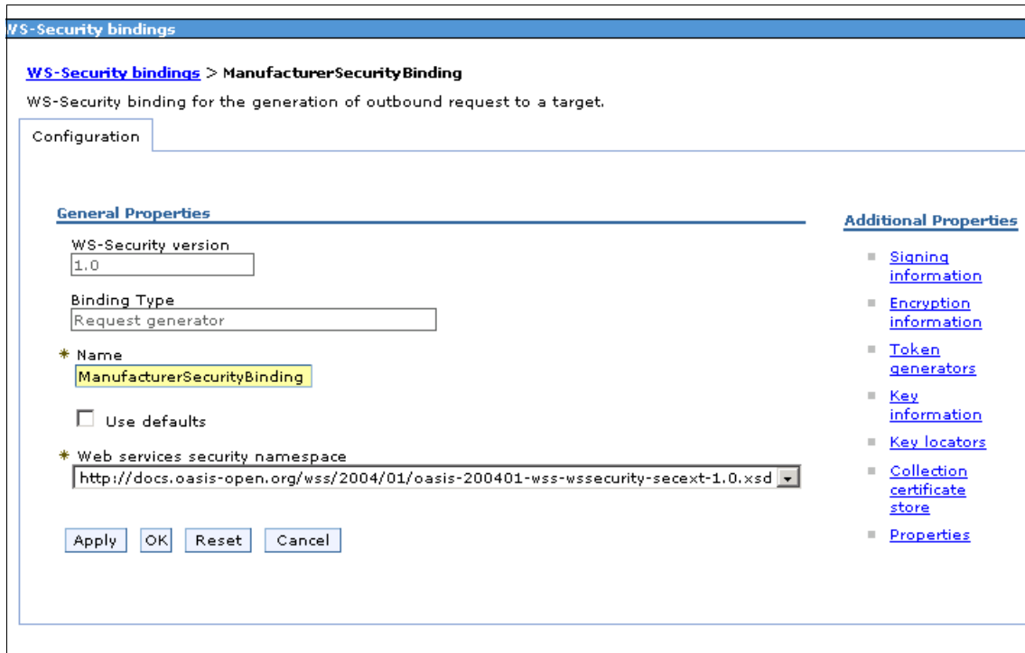
Figure 11-57 WS-Security binding
