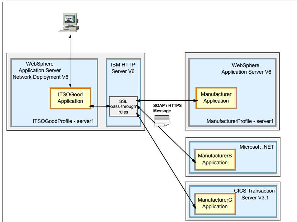
Figure 11-5 Solution topology
