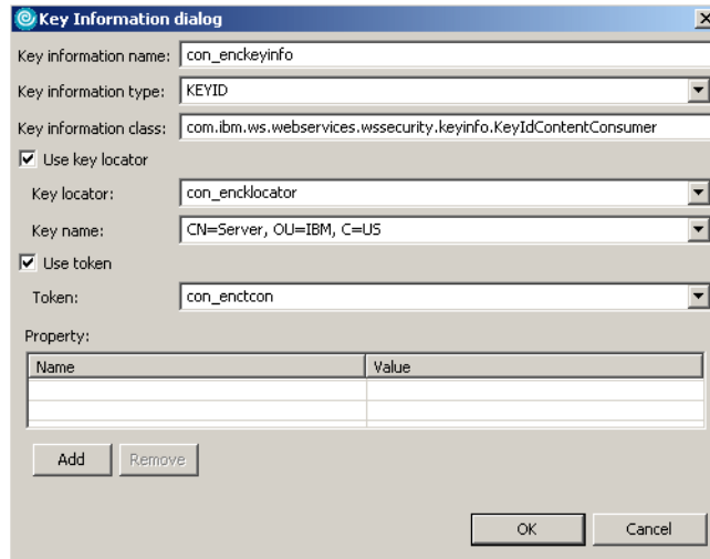
Figure 10-38 Key Information dialog for body content decryption
