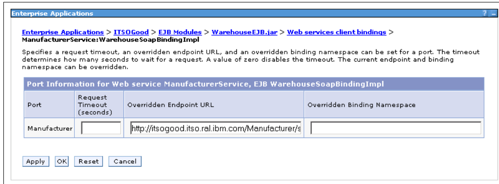
Figure 11-6 Overriding the endpoint URL for the Manufacturer
