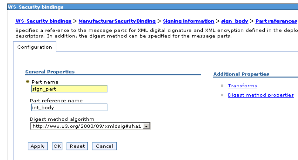
Figure 11-64 Creating the part reference
