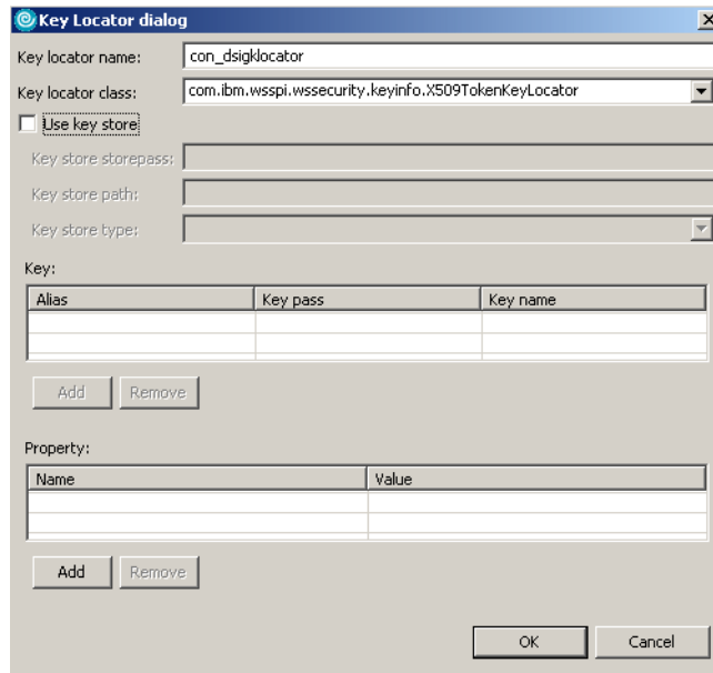
Figure 10-25 Key Locator dialog for signature verification (X.509 certificate)
