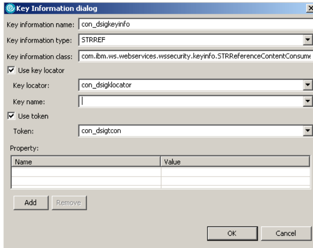
Figure 10-26 Key Information dialog for signature verification (X.509 certificate)
