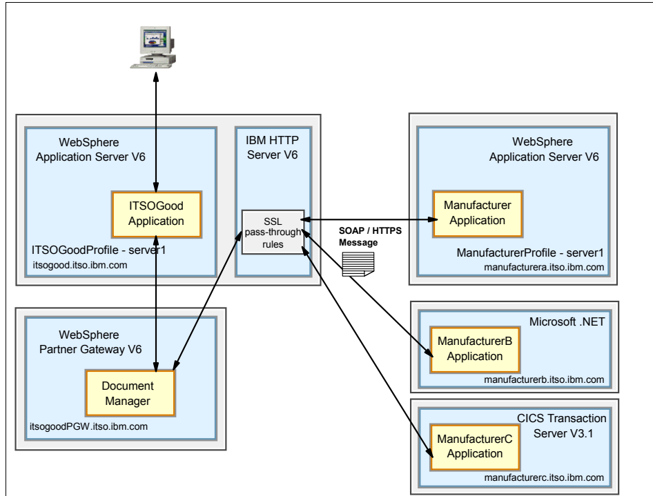
Figure 13-6 Solution topology
