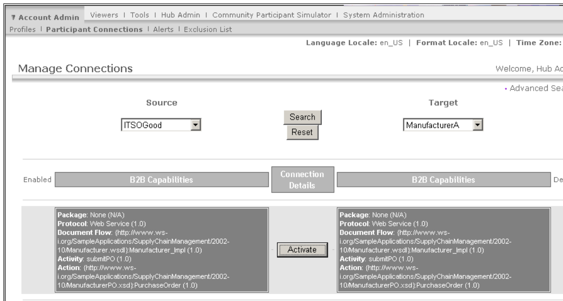
Figure 13-17 Connection awaiting activation
