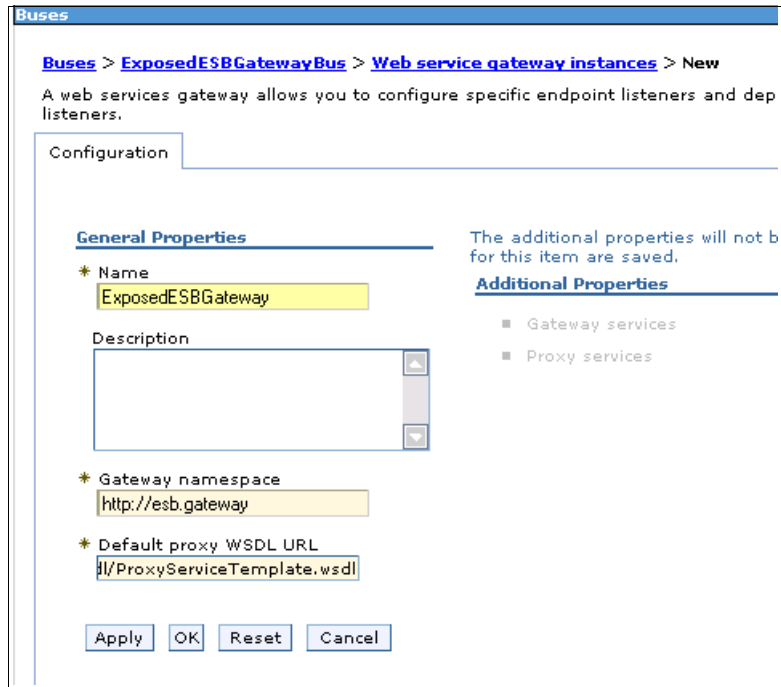
Figure 11-26 Create a gateway instance
