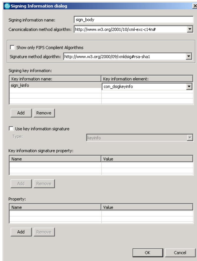
Figure 10-27 Signing Information dialog for signature verification (X.509 certificate)
