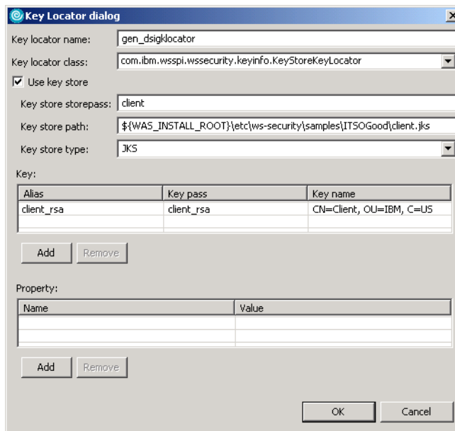
Figure 10-18 Key Locator dialog for signing by an X.509 certificate
