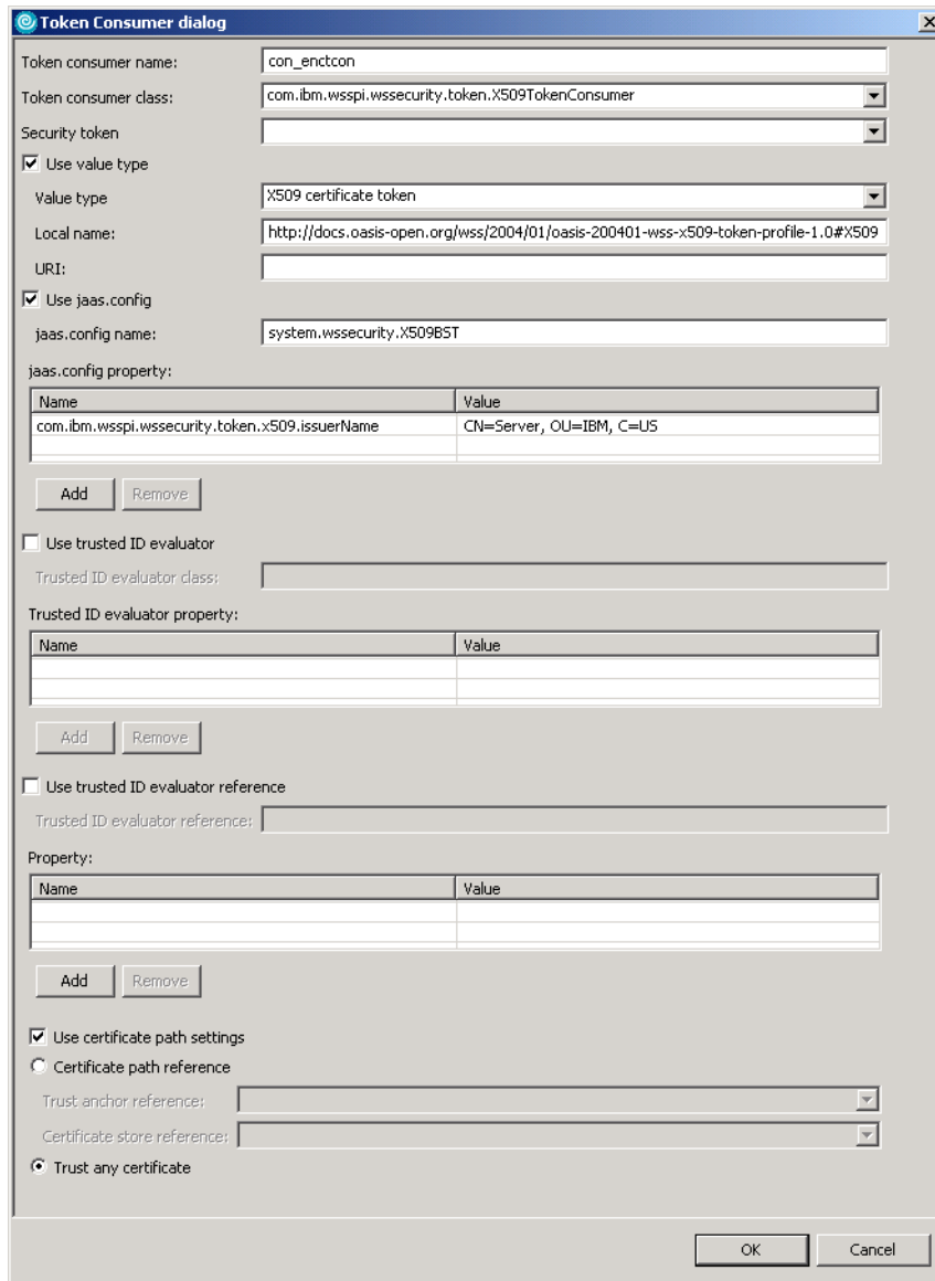
Figure 10-36 Token Consumer dialog for body content decryption
