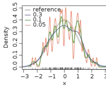
Kernel Density Function
