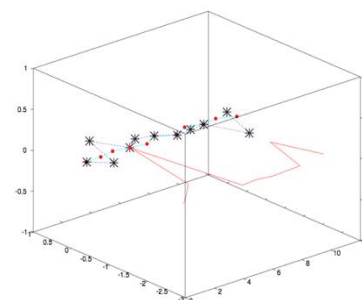
PCs(Principle Components) in EVD (Eigenvalue Value Decomposition)
