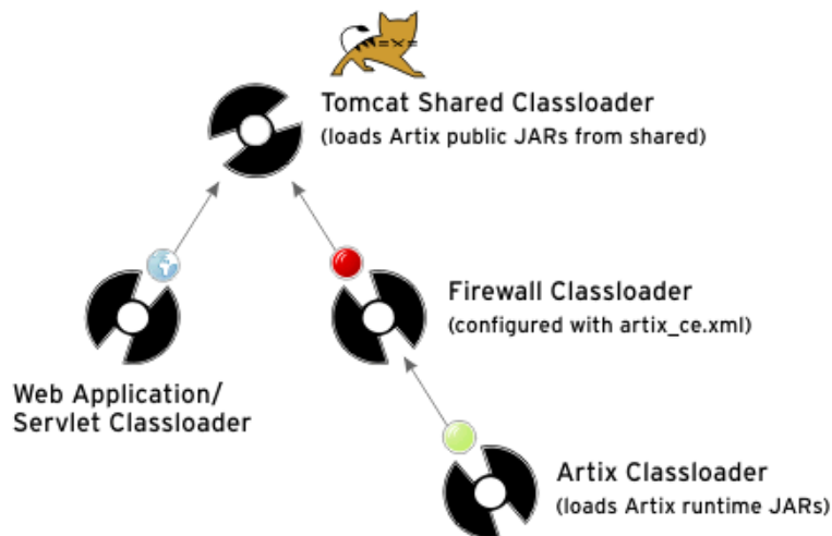
Figure 10: Classloader Configuration
