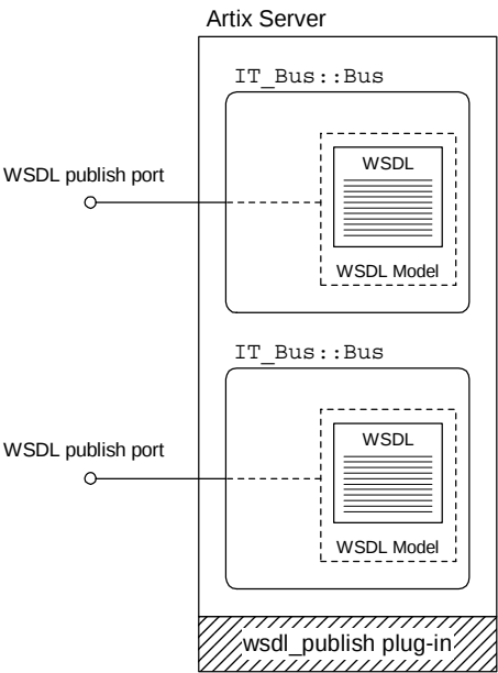
Figure 17: WSDL Publish Plug-In and Multiple Bus Instances
