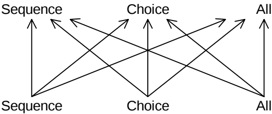
Figure 27: Allowed Inheritance Relationships for Complex Types
