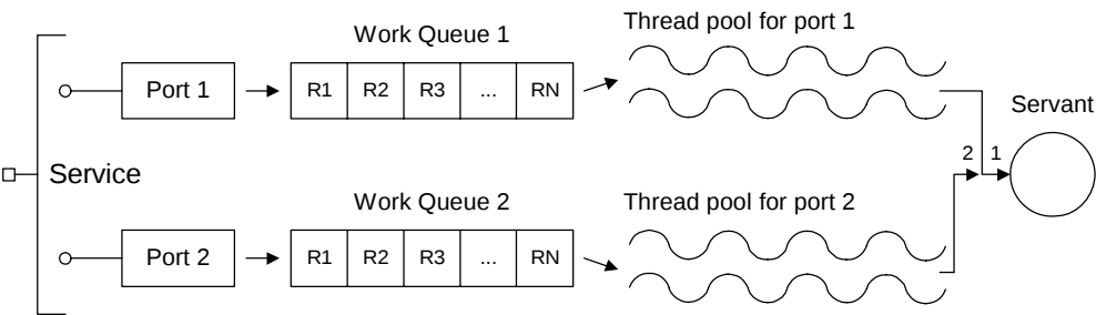
Figure 11: Outline of the Serialized Threading Model
