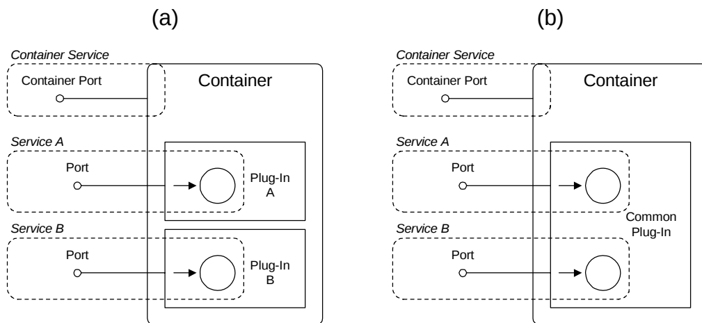
Figure 3: Multiple Services in Separate (a) or Common (b) Plug-In
