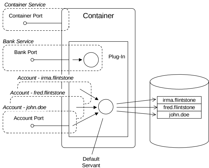
Figure 34: Default Servant Implementing Multiple Account Services
