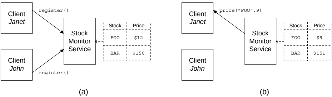
Figure 18: Callback Pattern Illustrated by a Stock Monitor Scenario
