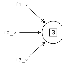
Figure 32: A Reference Counted Object Referenced by Three Vars
