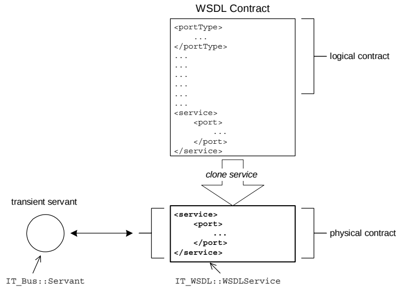
Figure 8: Relationship between a Transient Servant and a WSDL Contract
