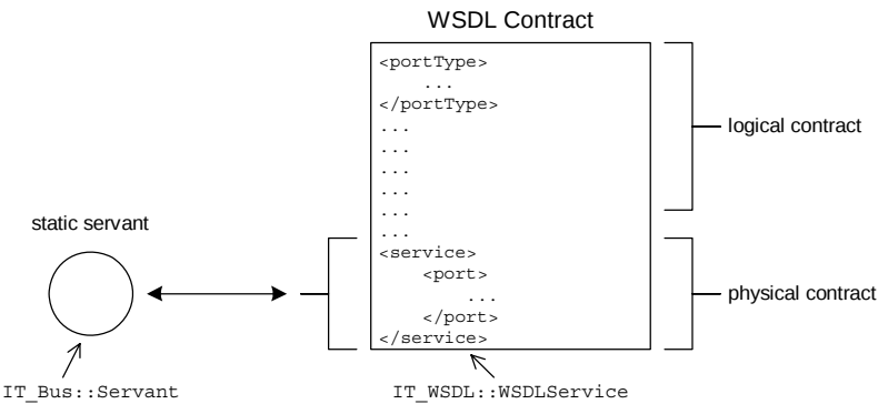
Figure 7: Relationship between a Static Servant and a WSDL Contract
