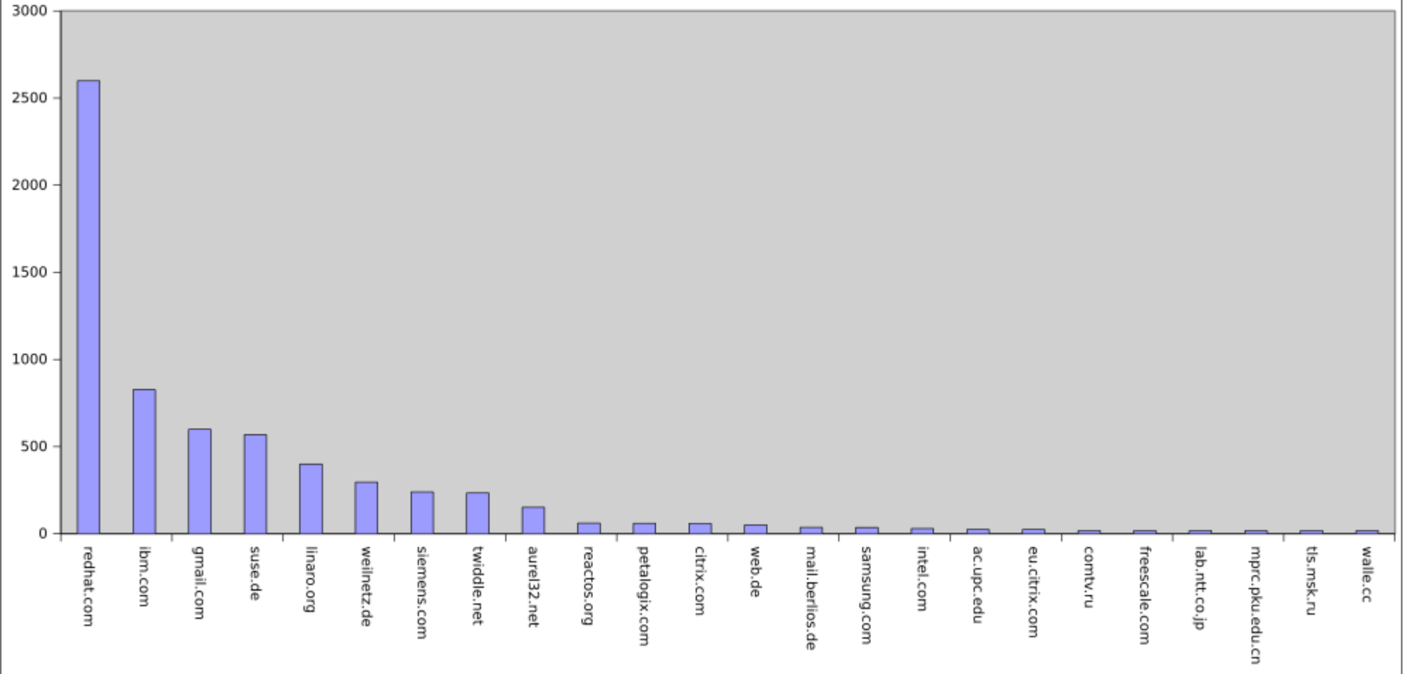
Commits per Domain Since KVM Forum 2011 (95%)
