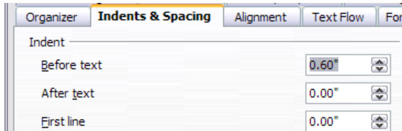
Figure 203: Set indentation
