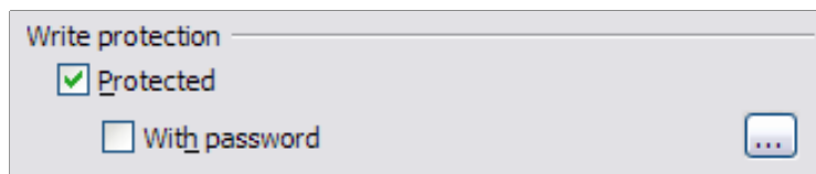
Figure 132: Write-protecting sections
