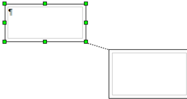
Figure 122: Linked frames
