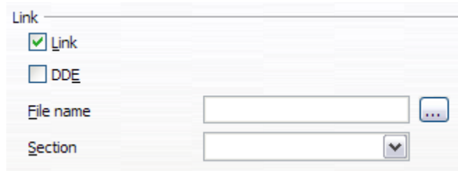
Figure 131: Linking sections
