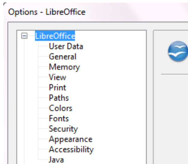
Figure 26: LibreOffice options
