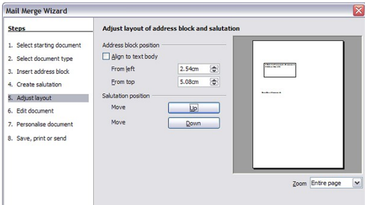
Figure 327: Adjust layout
