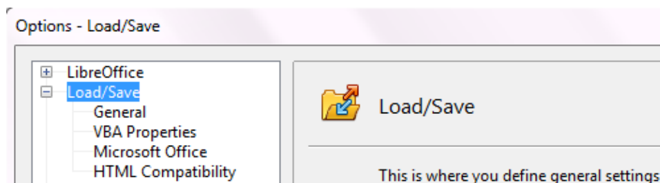
Figure 40: Load/Save options
