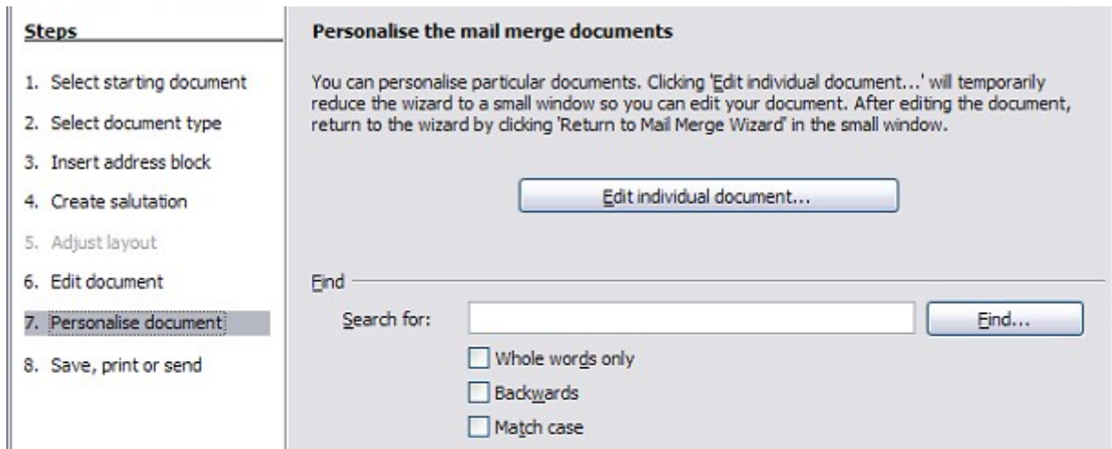
Figure 331: Personalize document
