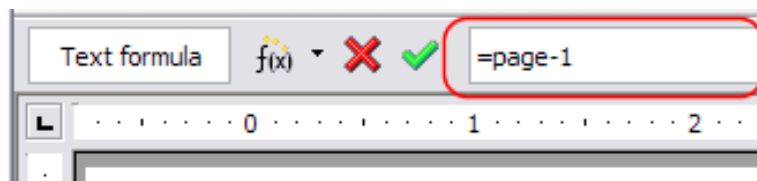
Figure 155: Formula bar
