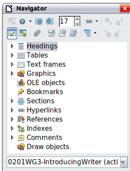
Figure 19. The Navigator
