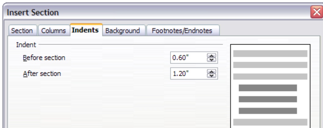
Figure 135: Indenting sections
