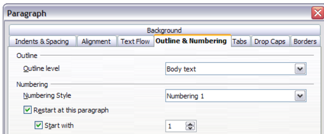
Figure 197: Restarting numbering
