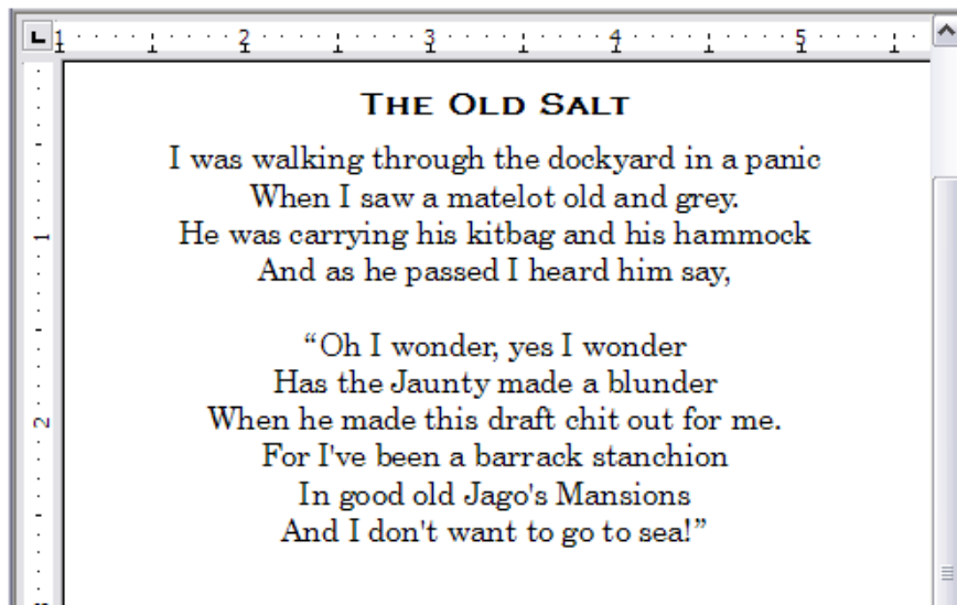
Figure 208: Sample poem
