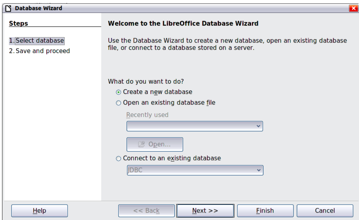
Figure 425: Database Wizard
