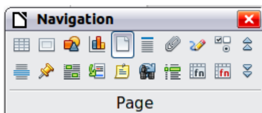
Figure 20: Navigation toolbar
