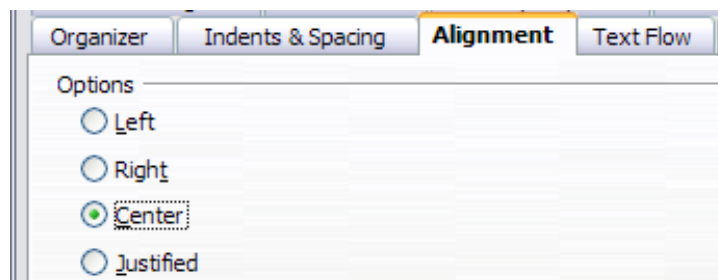
Figure 201: Center Heading 1
