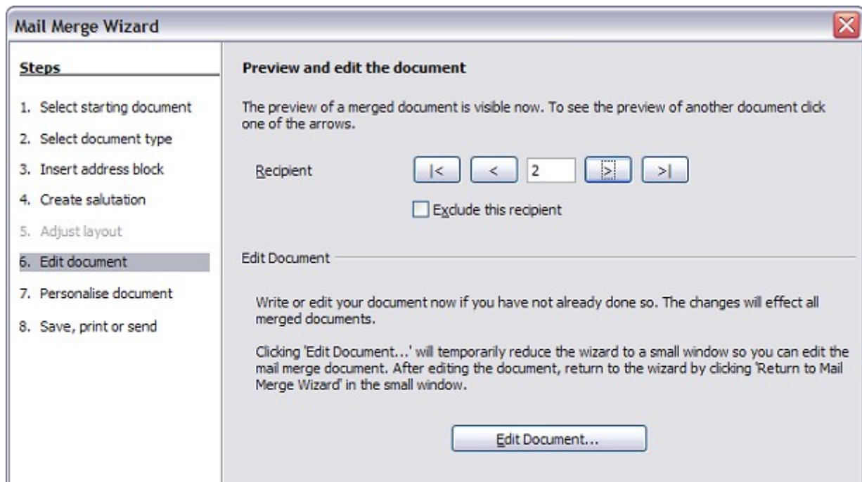
Figure 328: Edit document
