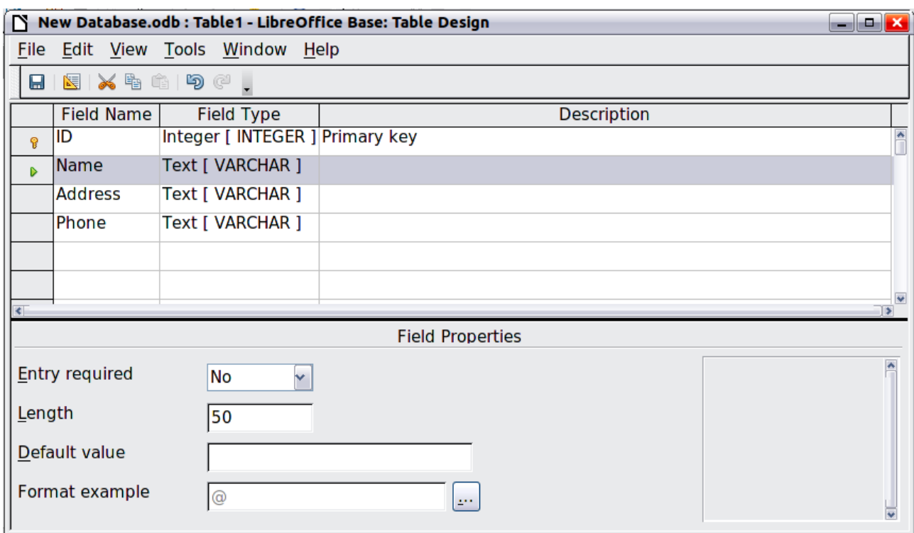
Figure 428: Database table design
