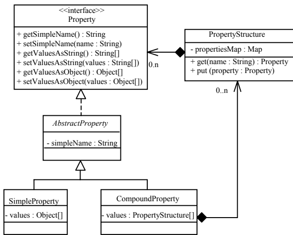
Figure 3. Generic support for property definition.
