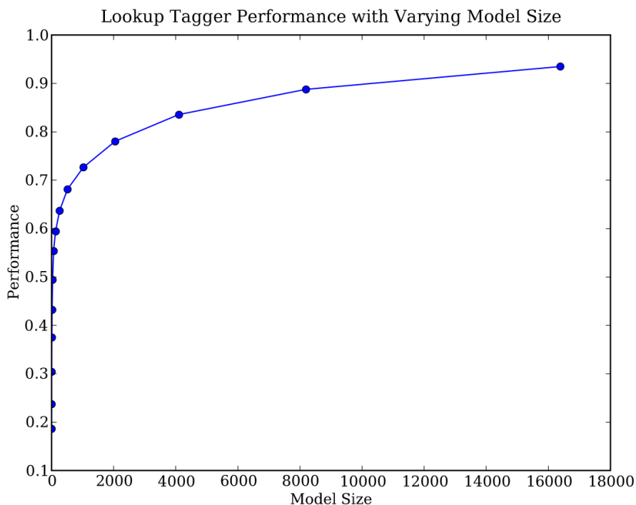
Figure 3.2: Lookup Tagger
