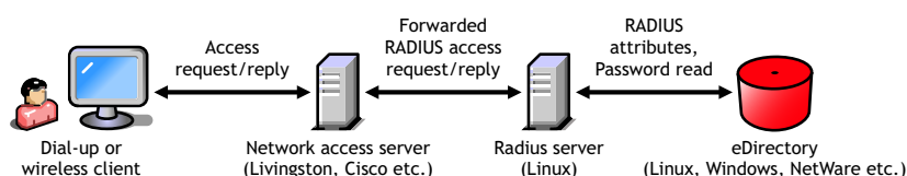
Figure 1-1 Wireless Authentication to eDirectory Integrated with FreeRADIUS
