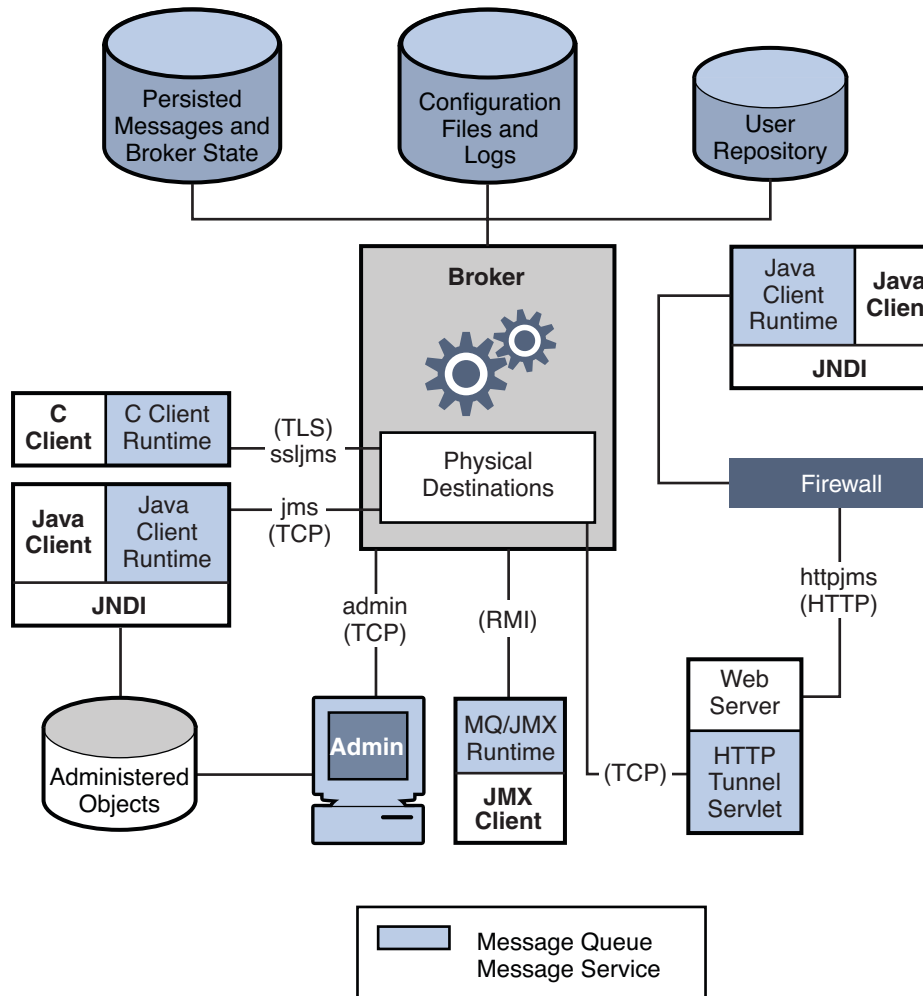
FIGURE 1-6 Message Queue Service
