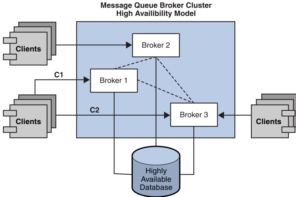
FIGURE 4–2 High Availability Cluster
