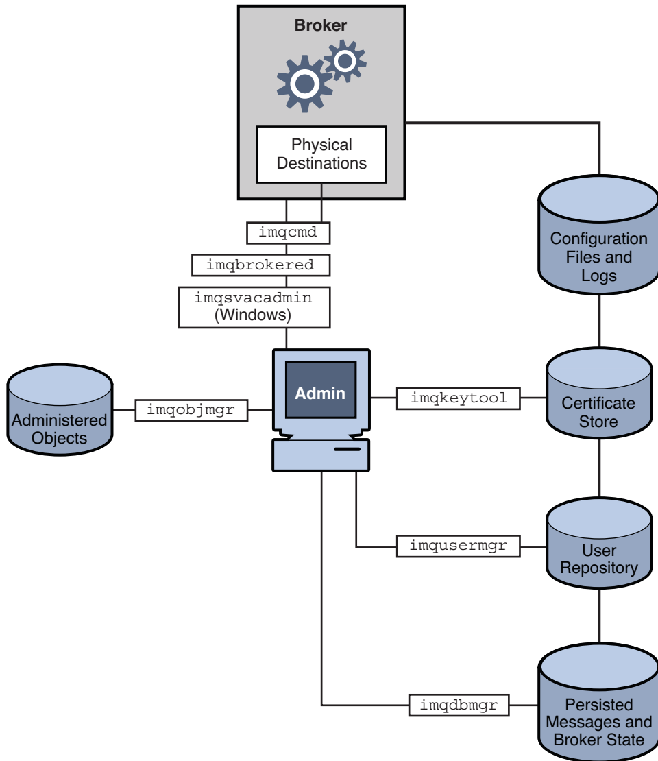
FIGURE 3-5 Administration Tools
