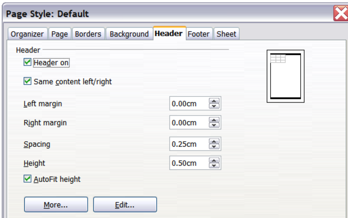
Figure 115: Header dialog
