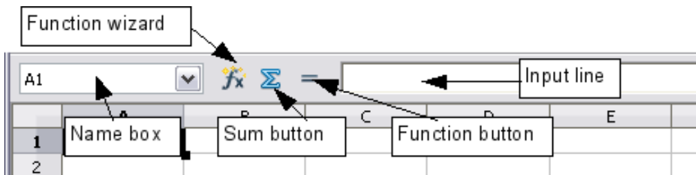
Figure 3: Formula Bar
