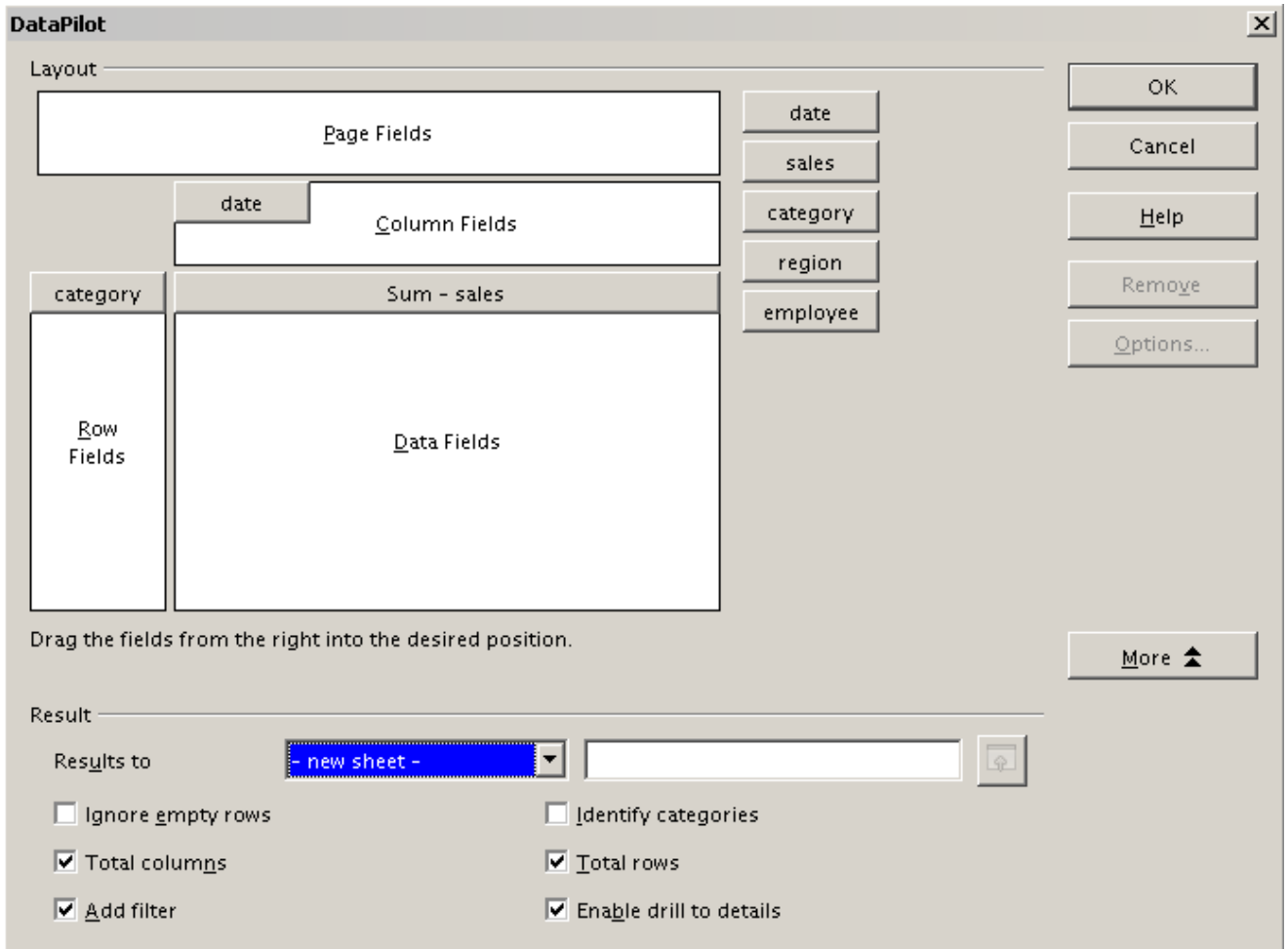
Figure 151: DataPilot dialog
