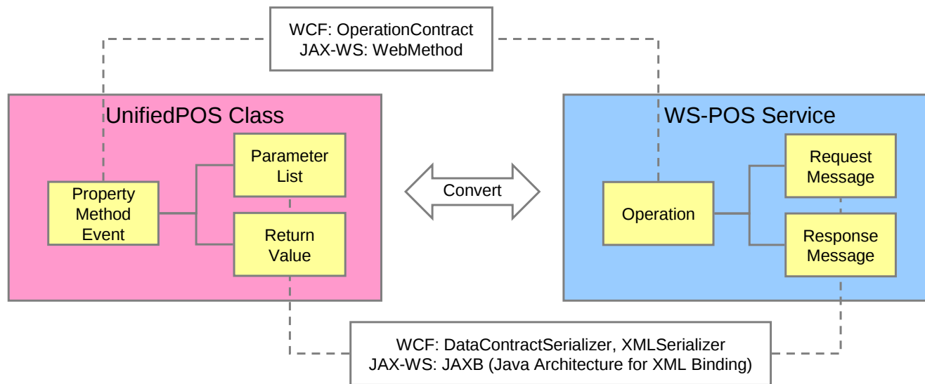
Figure 9: UnifiedPOS and WSDL Mapping
