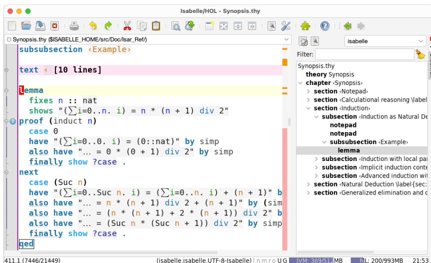
Figure 4.1: Isabelle document outline via SideKick tree view
