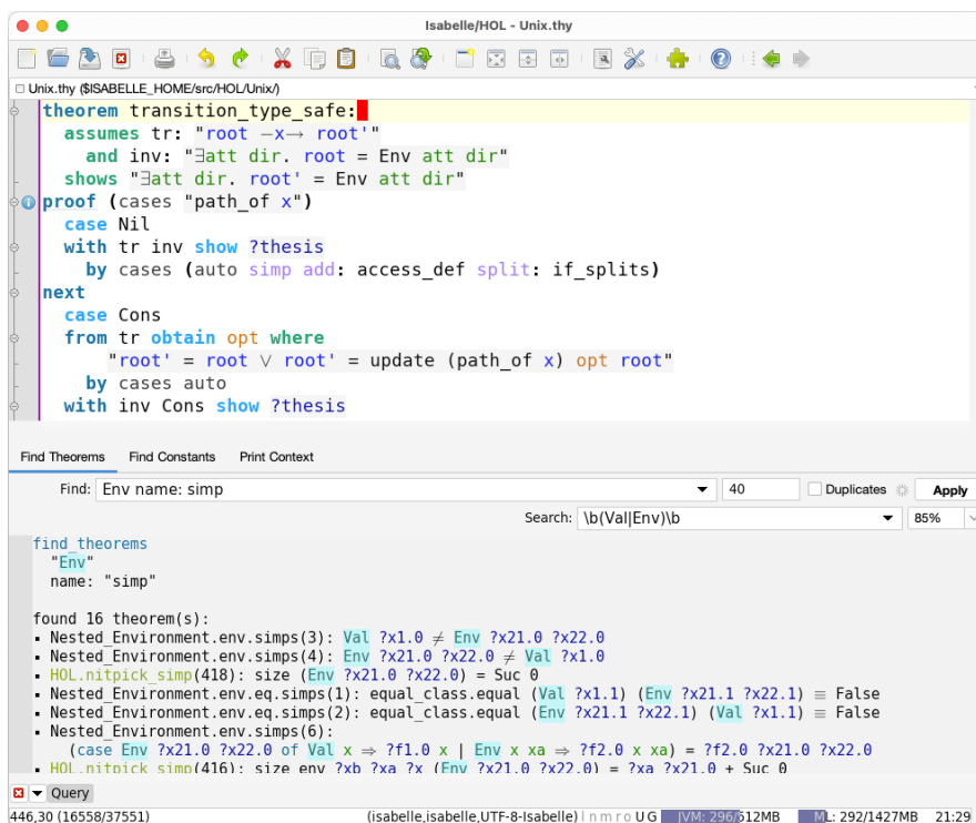
Figure 3.5: An instance of the Query panel: find theorems
