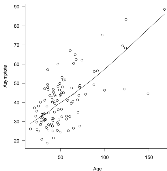
Figure 13.3: Plot of the estimated age at which the tree reaches half its maximum diameter against the estimated tree-level maximum diameter.
