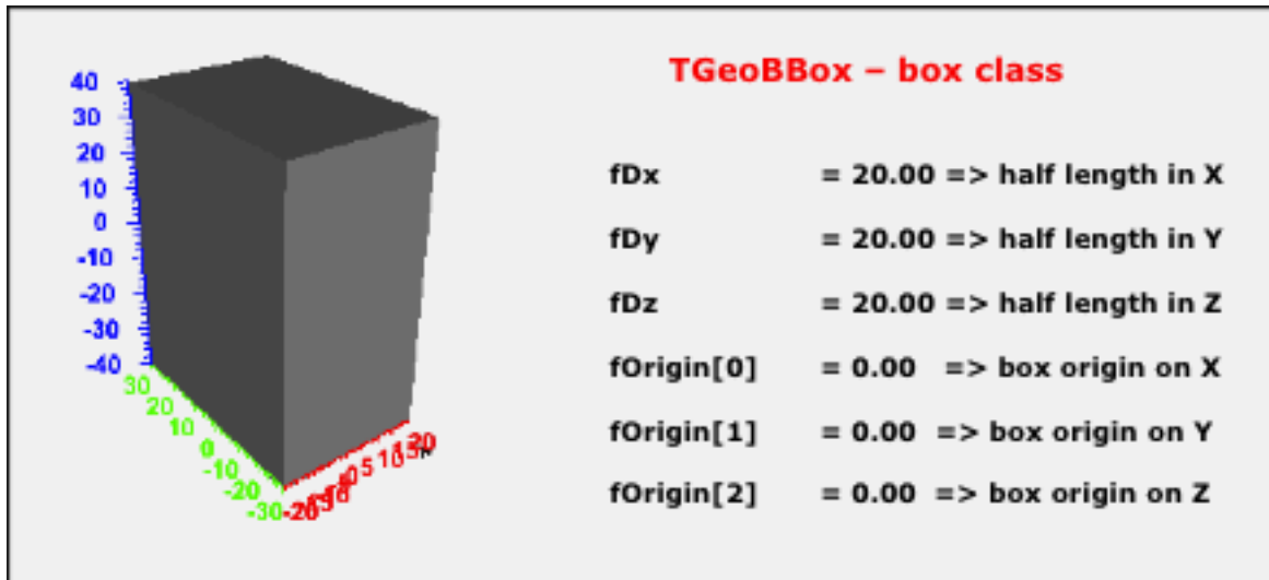
Figure 1.4: TGeoBBox class
