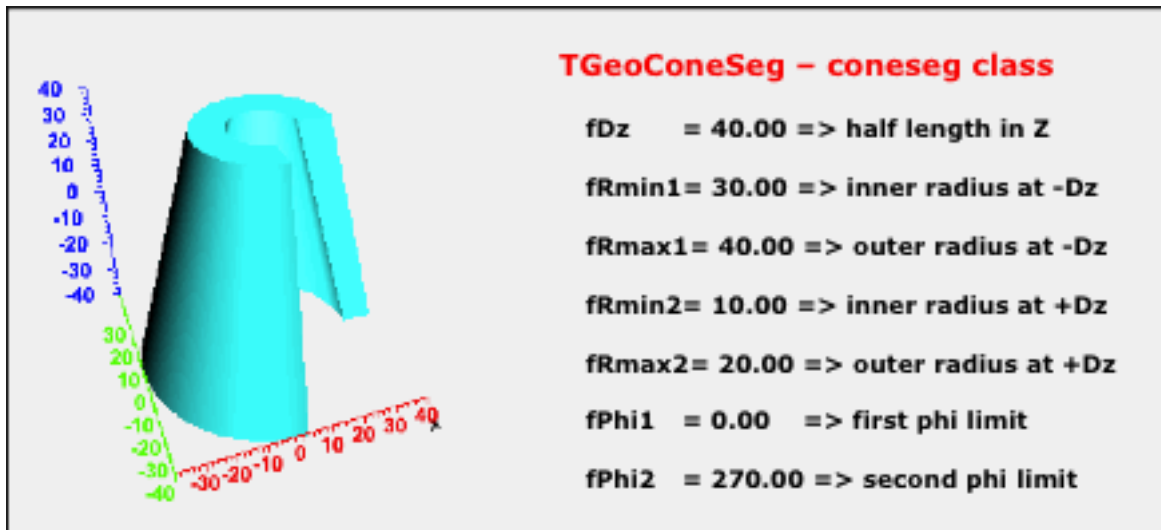
Figure 1.17: TGeoConeSeg Class
