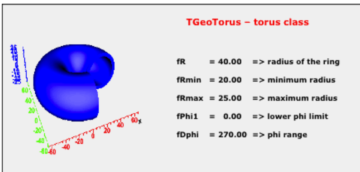
Figure 1.19: TGeoTorus Class
