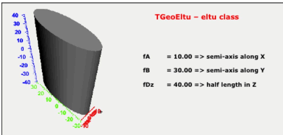
Figure 1.14: TGeoEltu Class
