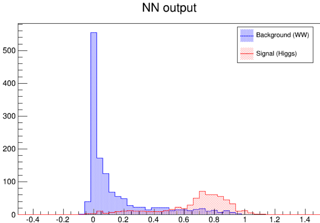
Figure 5.5: The neural net output
