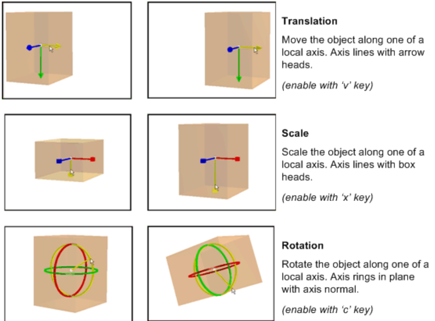
Figure 9.39: GL Viewer object manipulators
