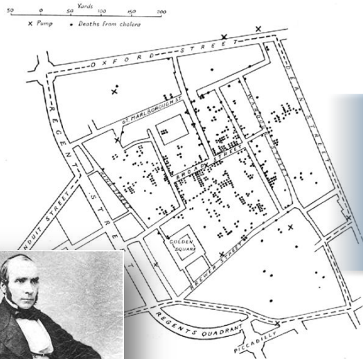
1854: London Cholera Death Scale
