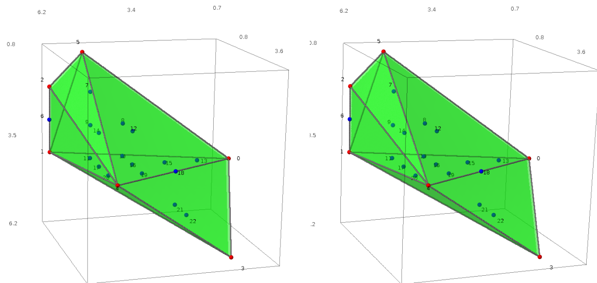
Fig. 5.3: Figure: The polytope L and its integer points, in cross-eyed stereographic perspective.
