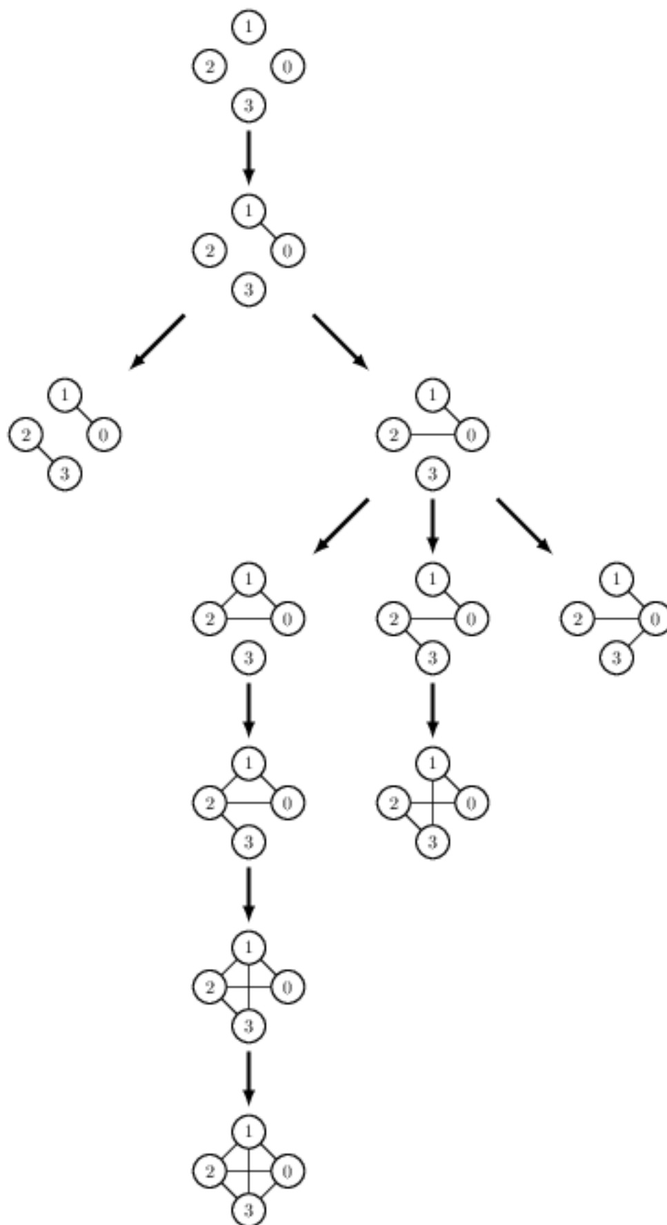
Fig. 5.4: Figure: The generation tree of simple graphs with 4 vertices.
