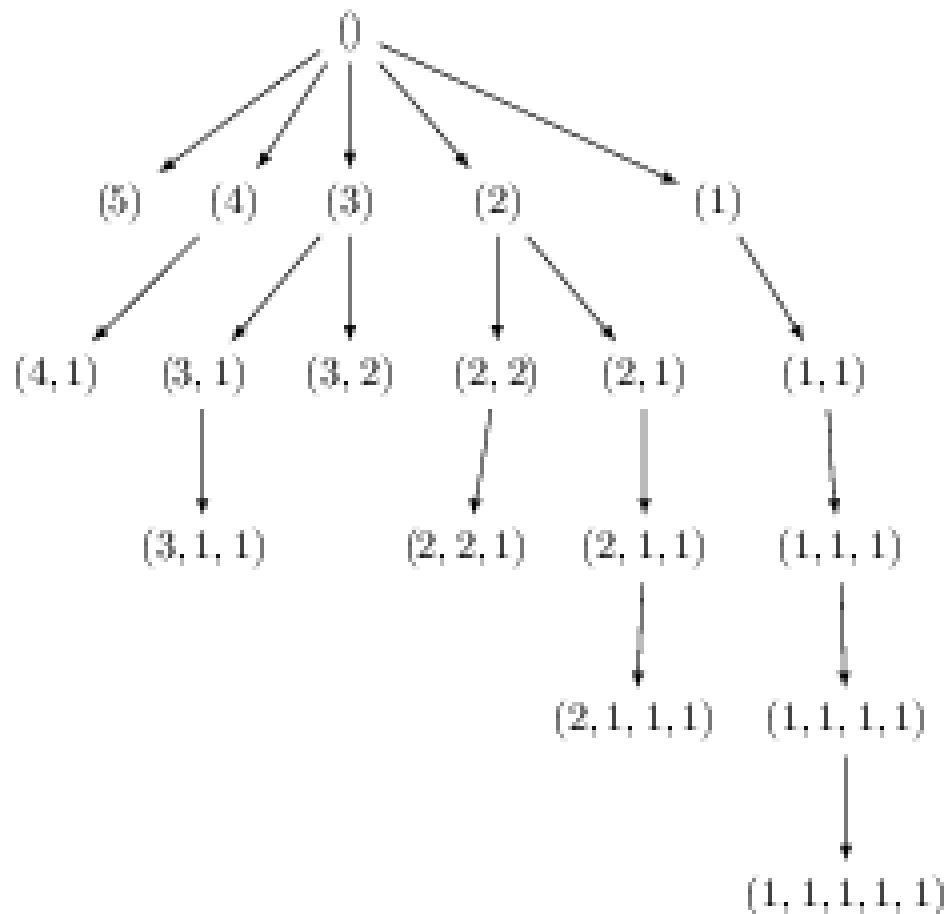
Fig. 5.2: Figure: The prefix tree of the partitions of 5.
