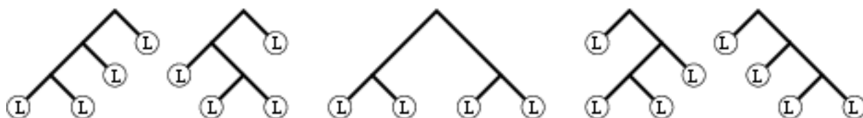
Fig. 5.1: Figure: The five complete binary trees with four leaves
