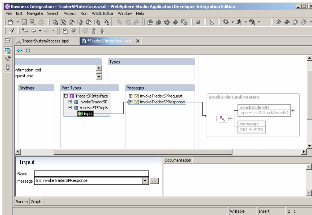
Figure 9-28 Trader system process interface including the receiveEISReply operation
