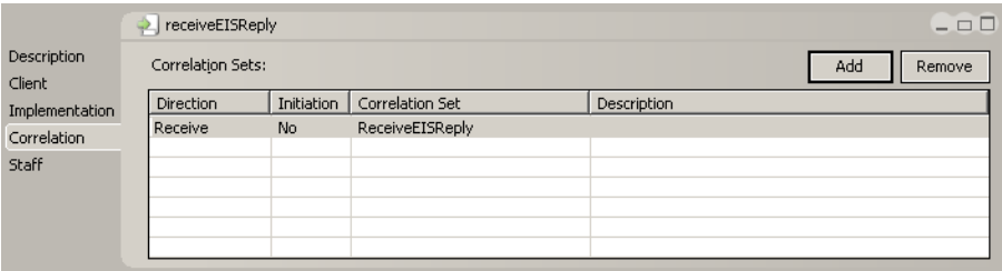
Figure 9-32 Correlation settings for the Pick activity
