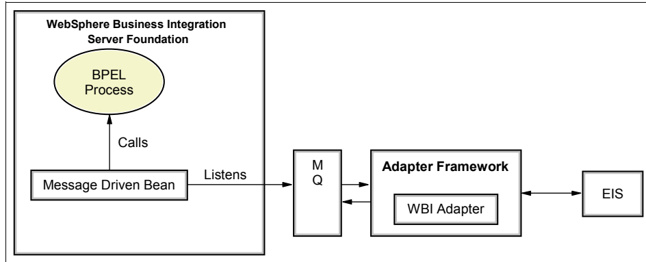
Figure 8-2 Event notification Interaction components view
