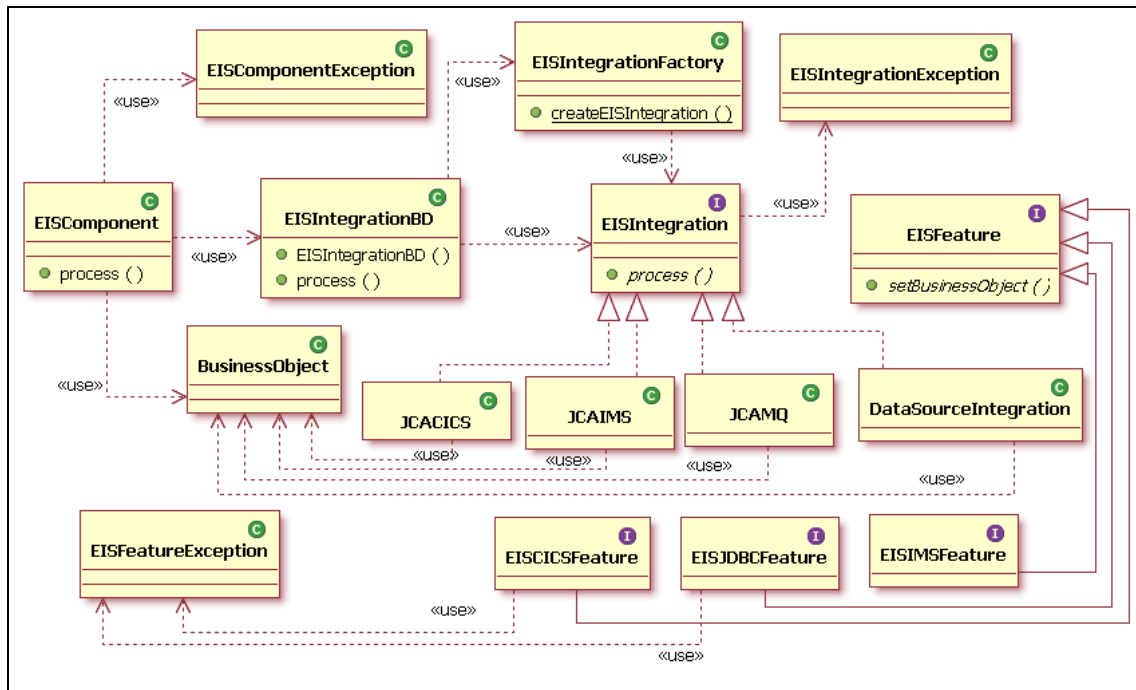
Figure 2-12 EIS component model
