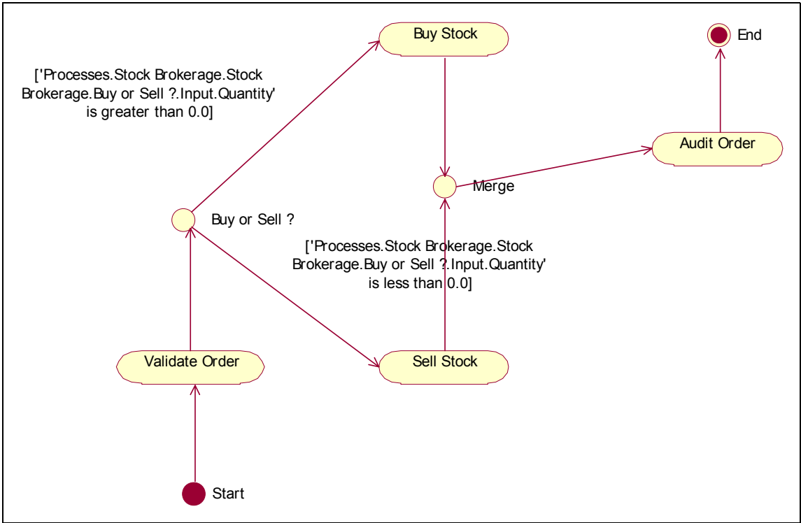
Figure 9-10 Stock Brokerage activity diagram
