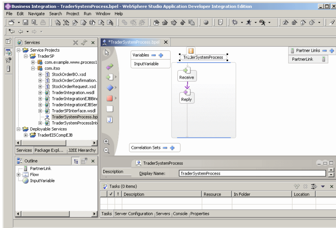
Figure 9-14 BPEL editor
