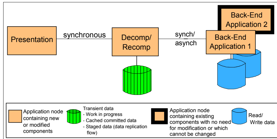
Figure 3-7 Self-Service::Decomposition pattern
