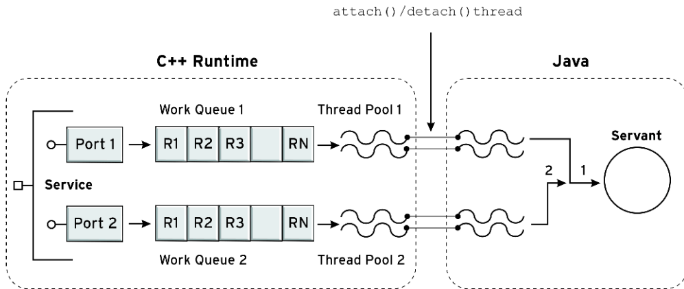
Figure 2: SerializedServant
