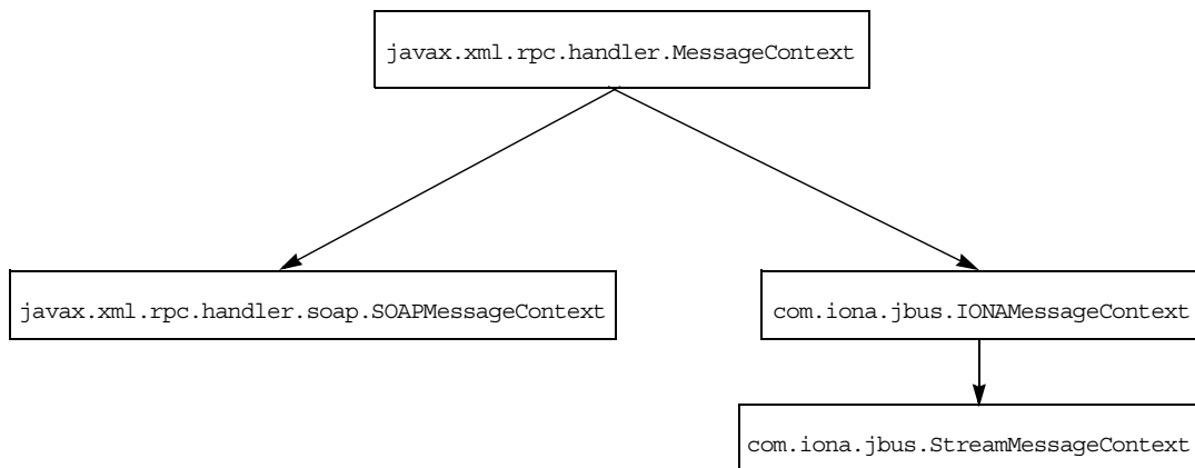
Figure 5: Artix Message Context Hierarchy
