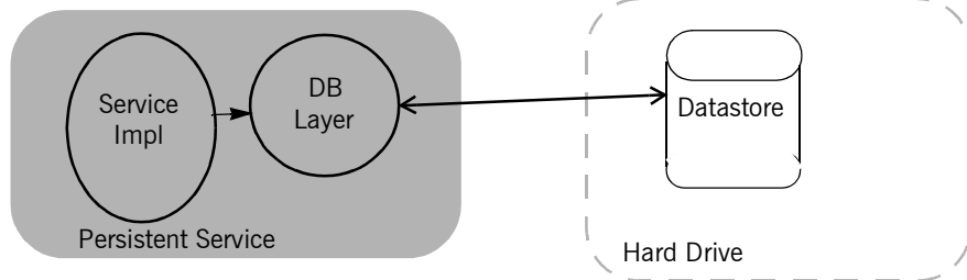
Figure 8: The Artix Persistence Mechanism
