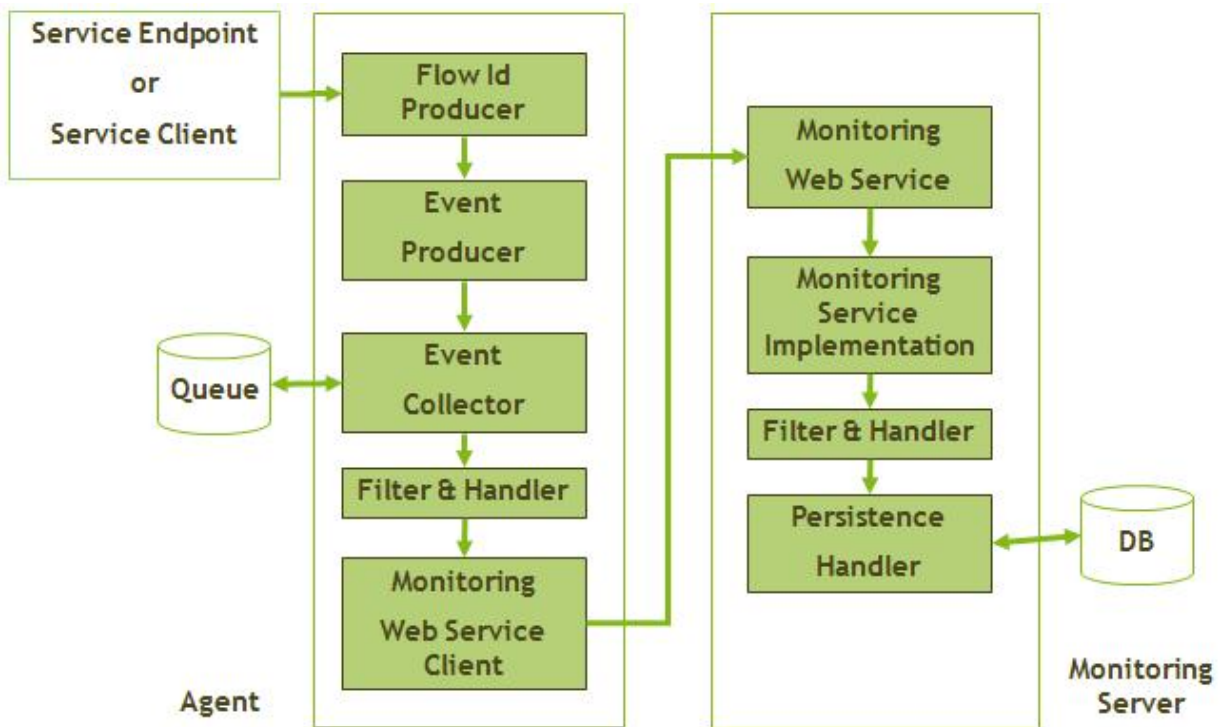
Figure 7.1. Architecture of Service Activity Monitoring
