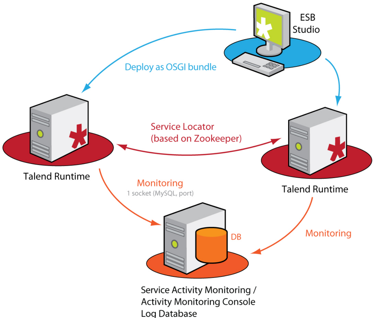
Figure 2.2. Talend Open Studio for ESB components
