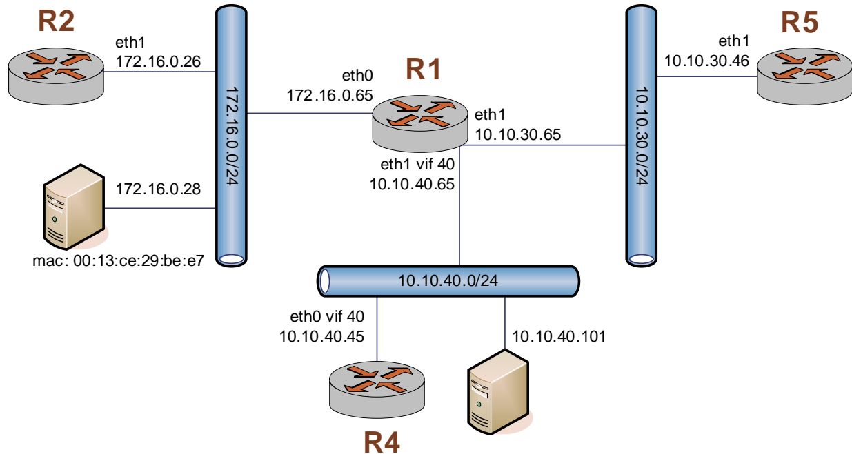
Figure 2-1 Firewall
