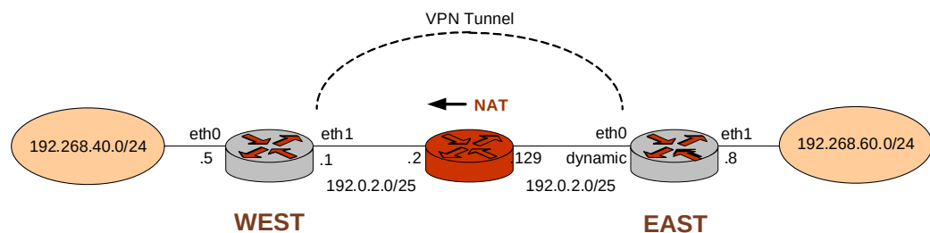
Figure 14-2 IPsec VPN connection with dynamic IP address and NAT
