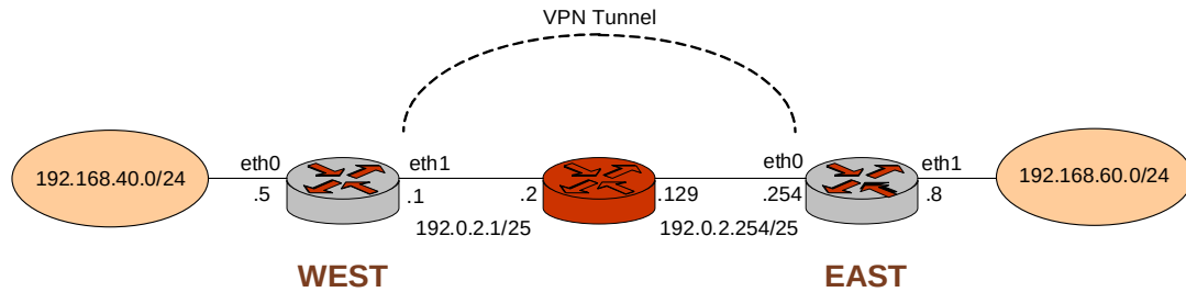
Figure 14-1 Basic site-to-site IPsec VPN connection
