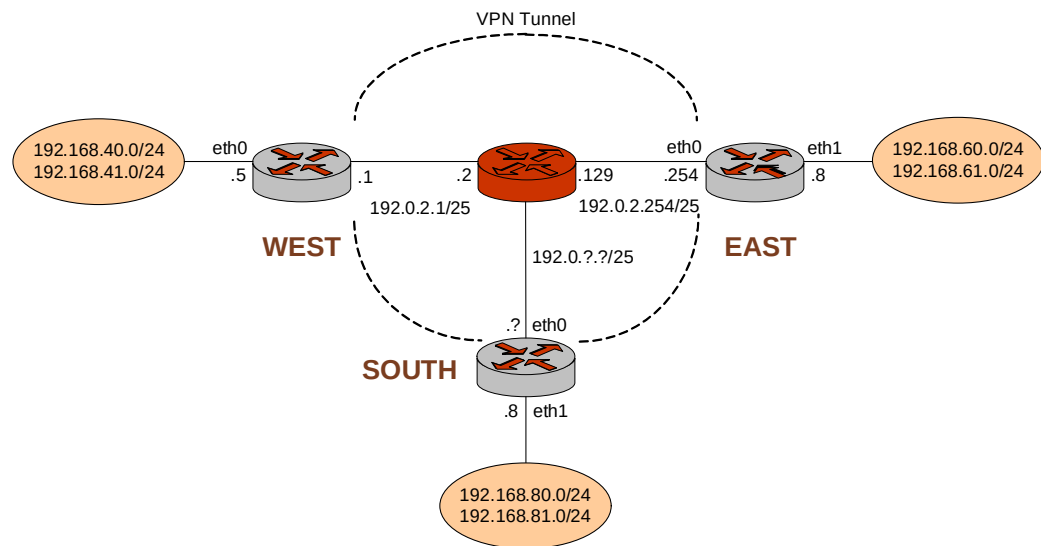
Figure 14-3 Multiple site-to-site tunnels between three gateways
