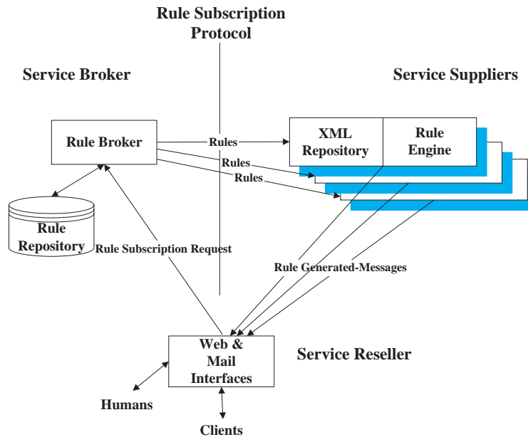
Figure 1: Reactive E-service Application Scenario
