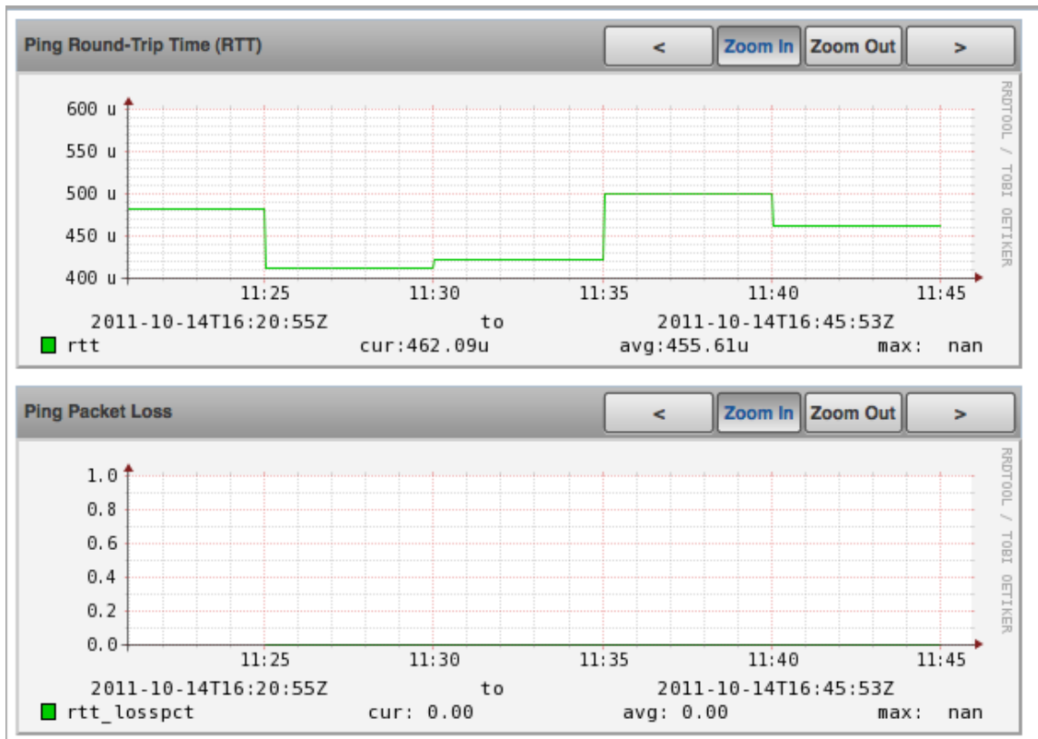
Figure 6.12. Ping Graph
