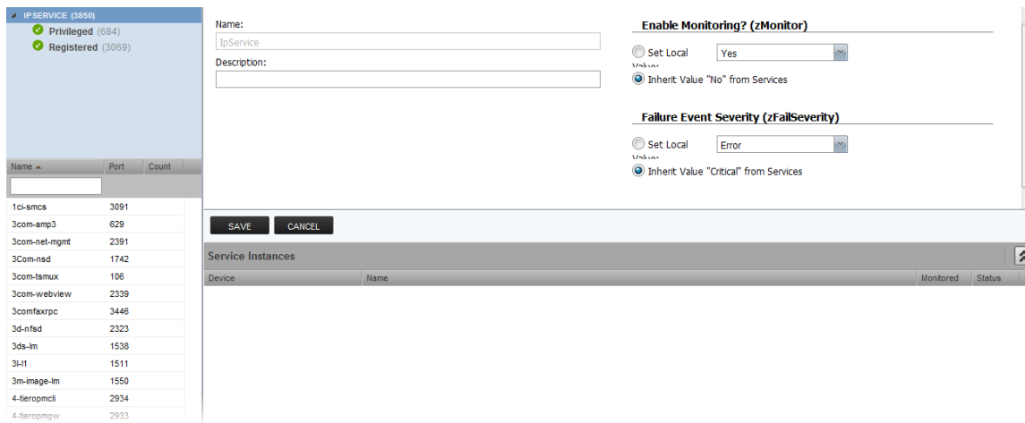
Figure 6.3. IP Services
