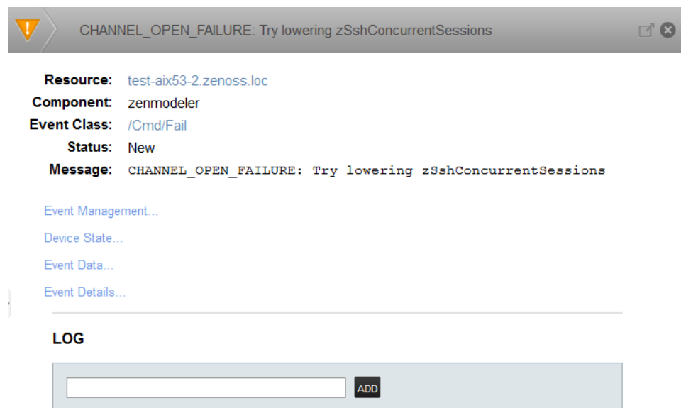
Figure 2.12. Event Detail
