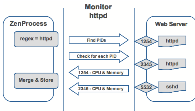
Figure 6.1. Process Monitoring
