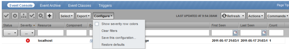
Figure 7.3. Event Console
