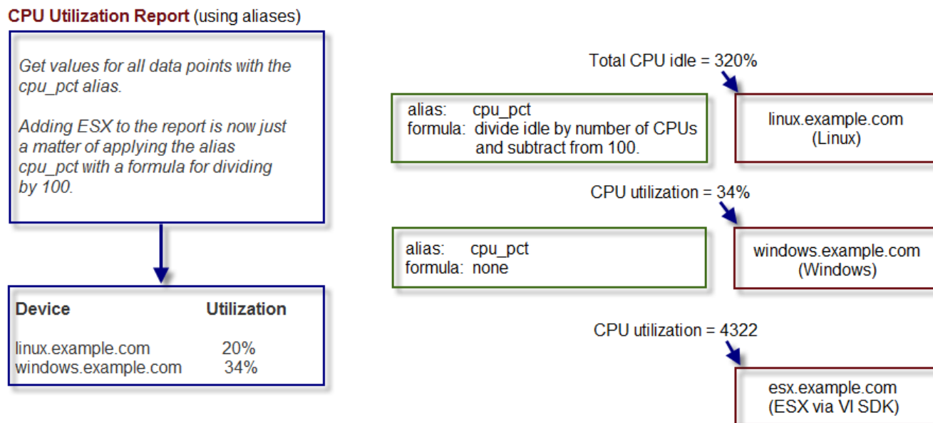
Figure 6.7. Alias-Based CPU Utilization Report
